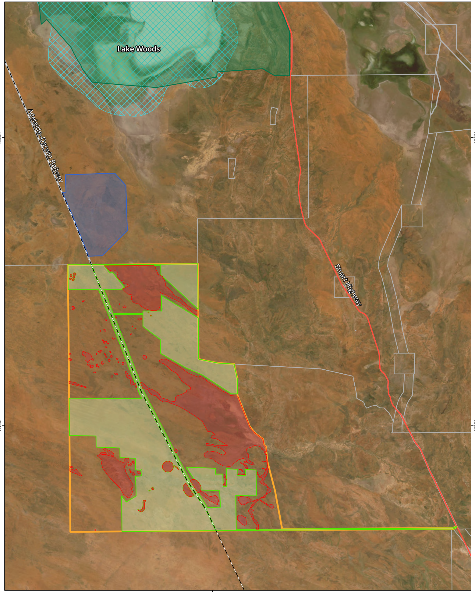
Figure 2-3 Preliminary Disturbance Footprint and Avoidance Areas Project: Australia-Asia PowerLink
