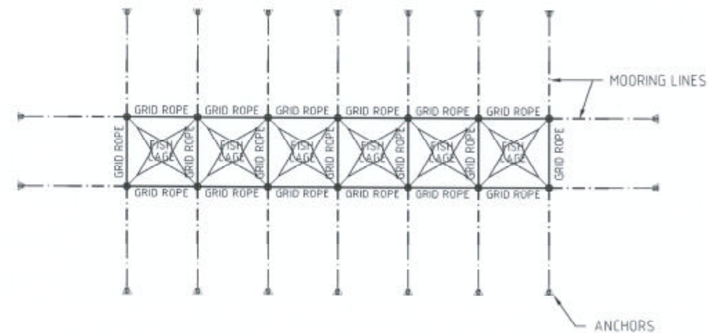
PLAN VIEW - MOORING ARRANGEMENT
