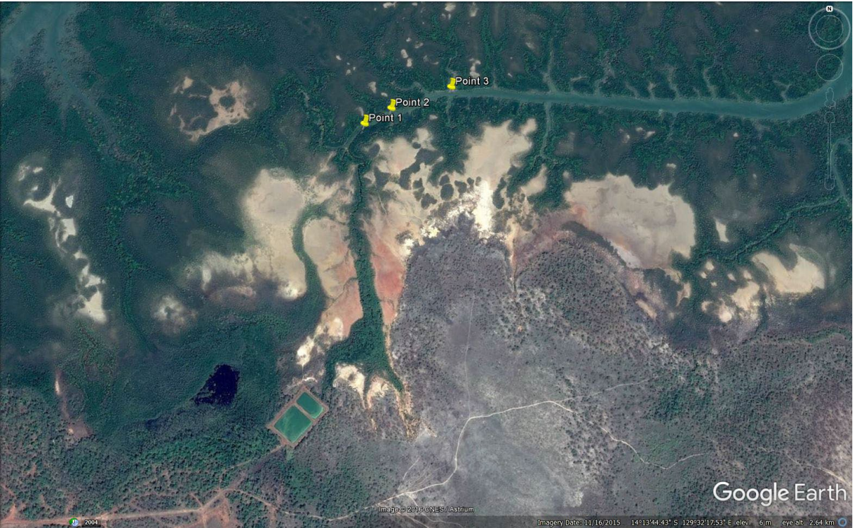
Figure 8: Dee Creek surface watercourse showing 100, 200 and 400 m locations from point where treated wastewater enters estuary (Google Earth 2017)
