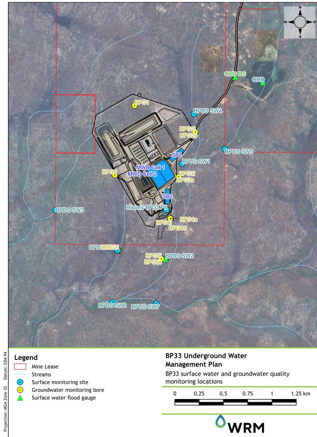
Figure 6.1 Surface water and ground water quality monitoring sites
