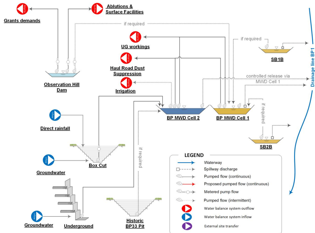
Figure 4.1 BP33 WMS schematic (base case conditions)
