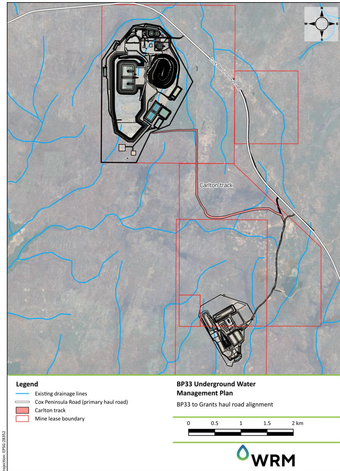
Figure 4.2 BP33 to Grants haul road alignment
