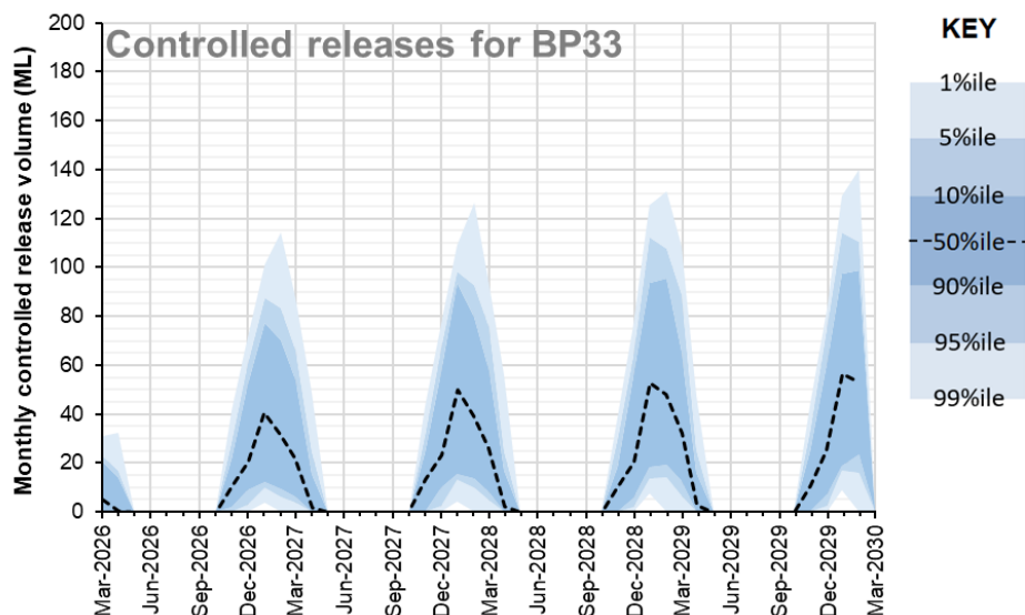
Figure 5.3 Monthly controlled releases
