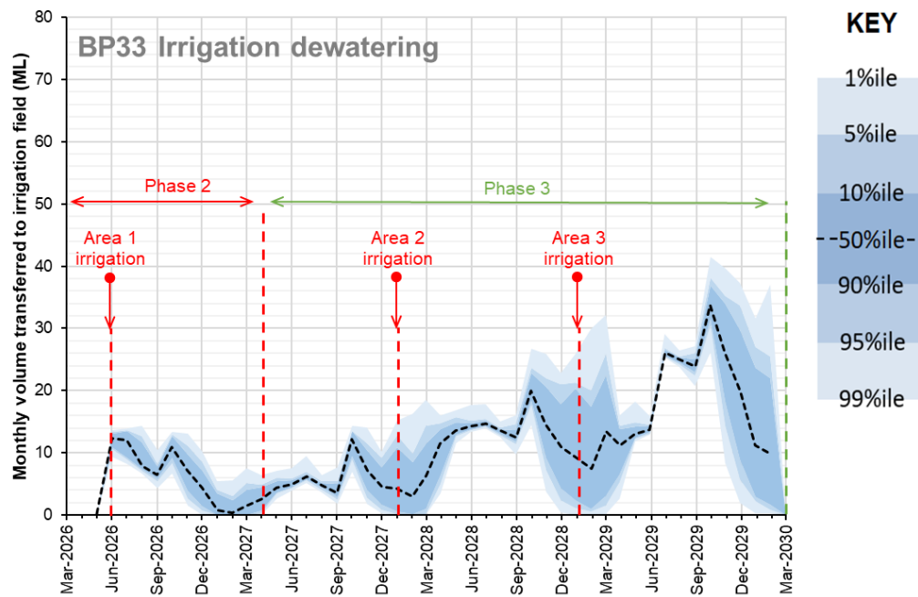
Figure 5.4 Monthly irrigation releases
