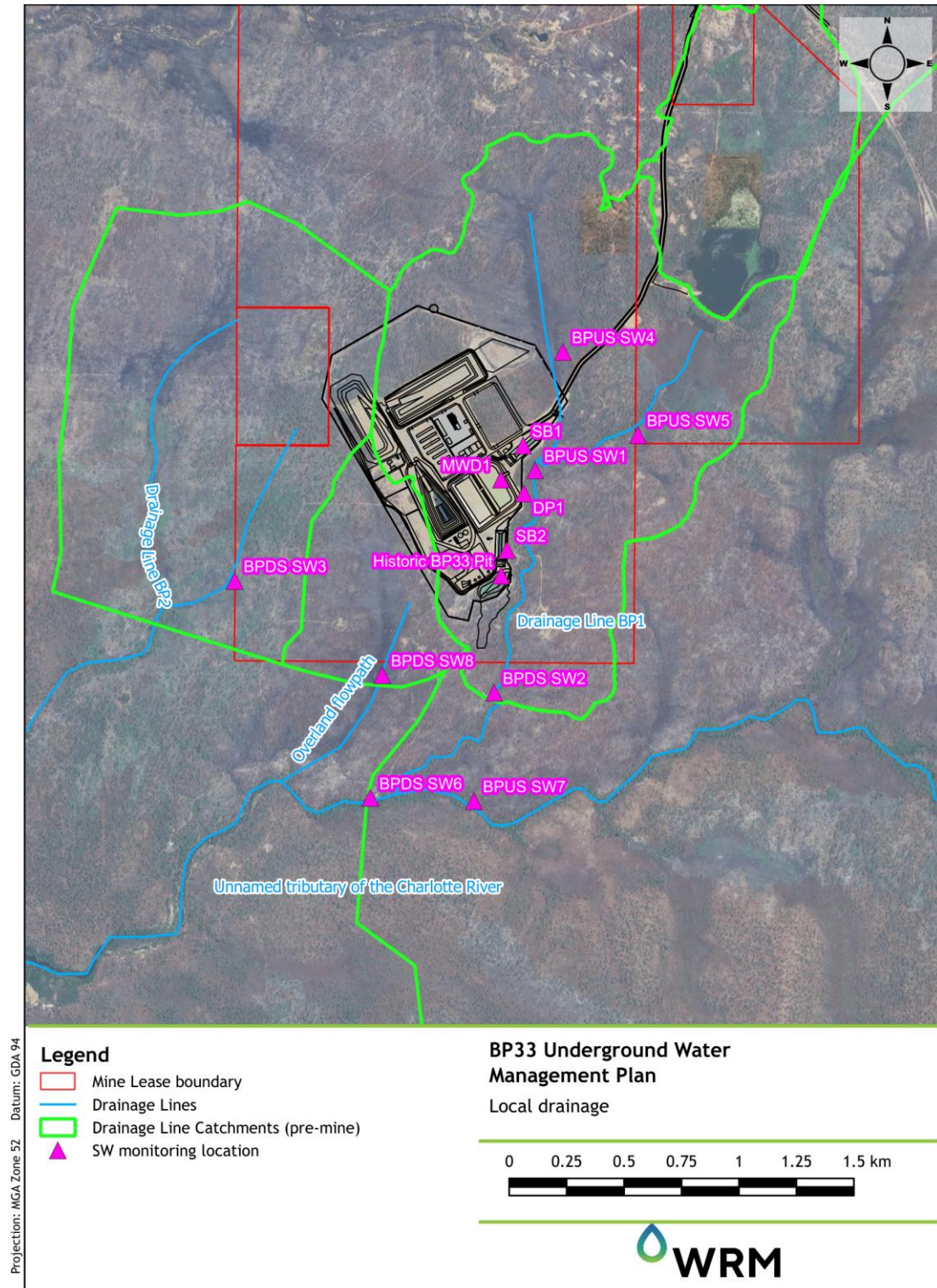
Figure 2.2 Local drainage
