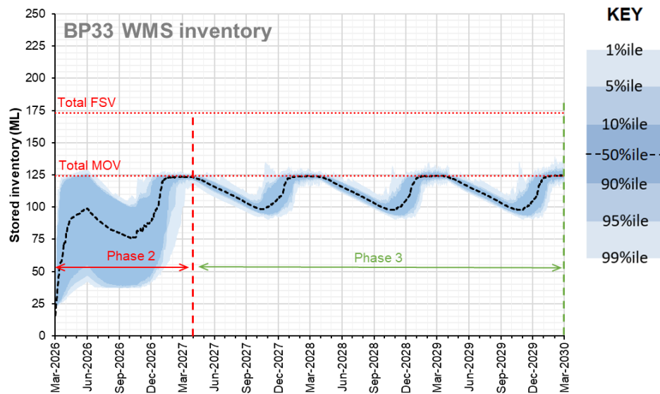
Figure 5.2 Total storage inventory in the WMS
