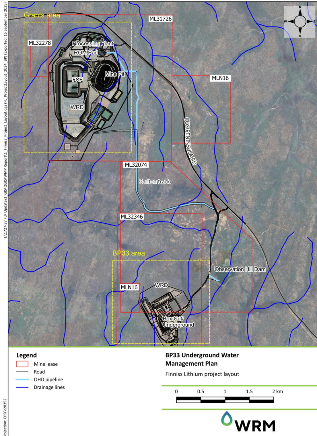
Figure 1.4 Finiss Lithium project layout
