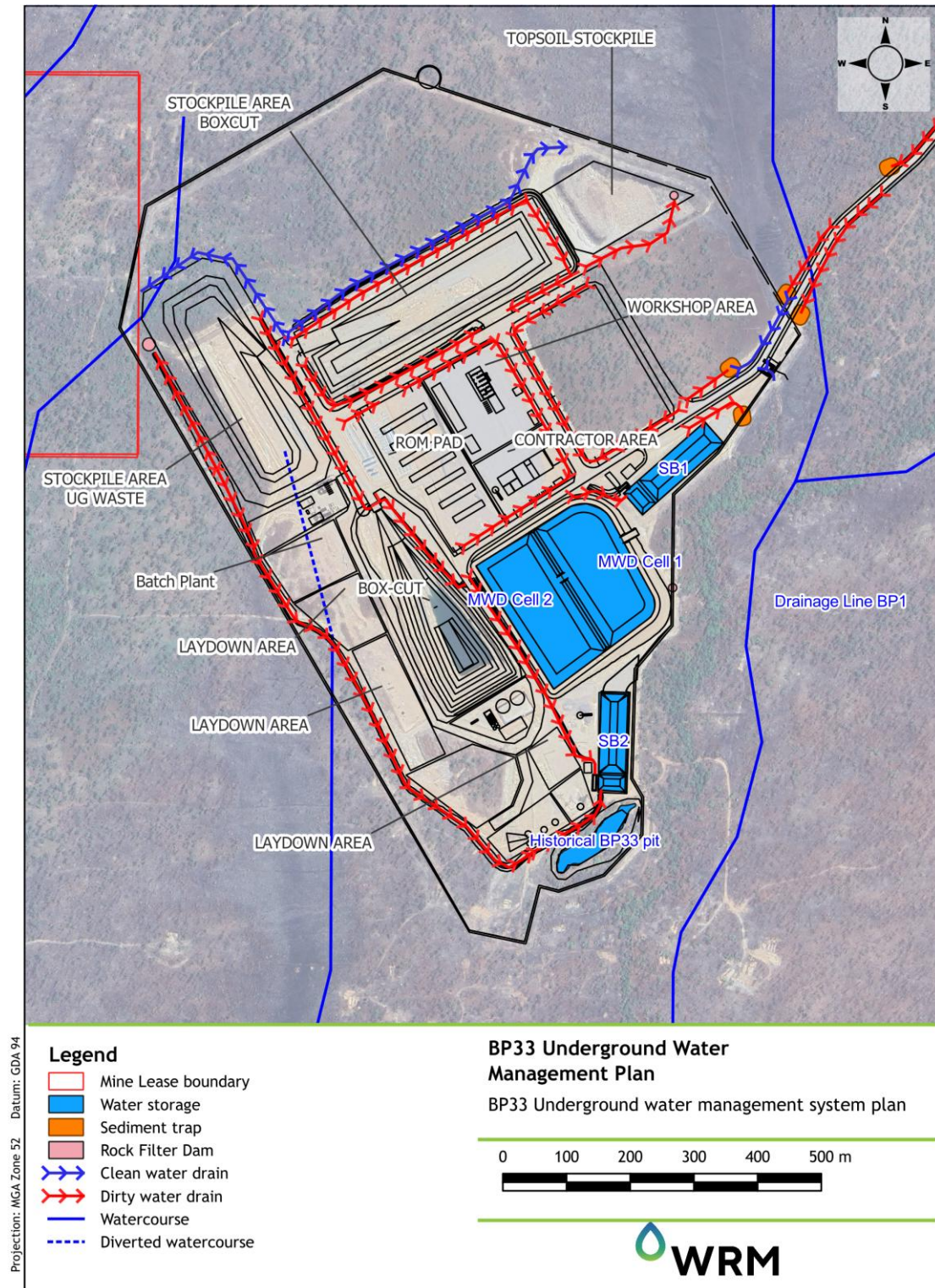
Figure 1.3 BP33 water management system plan
