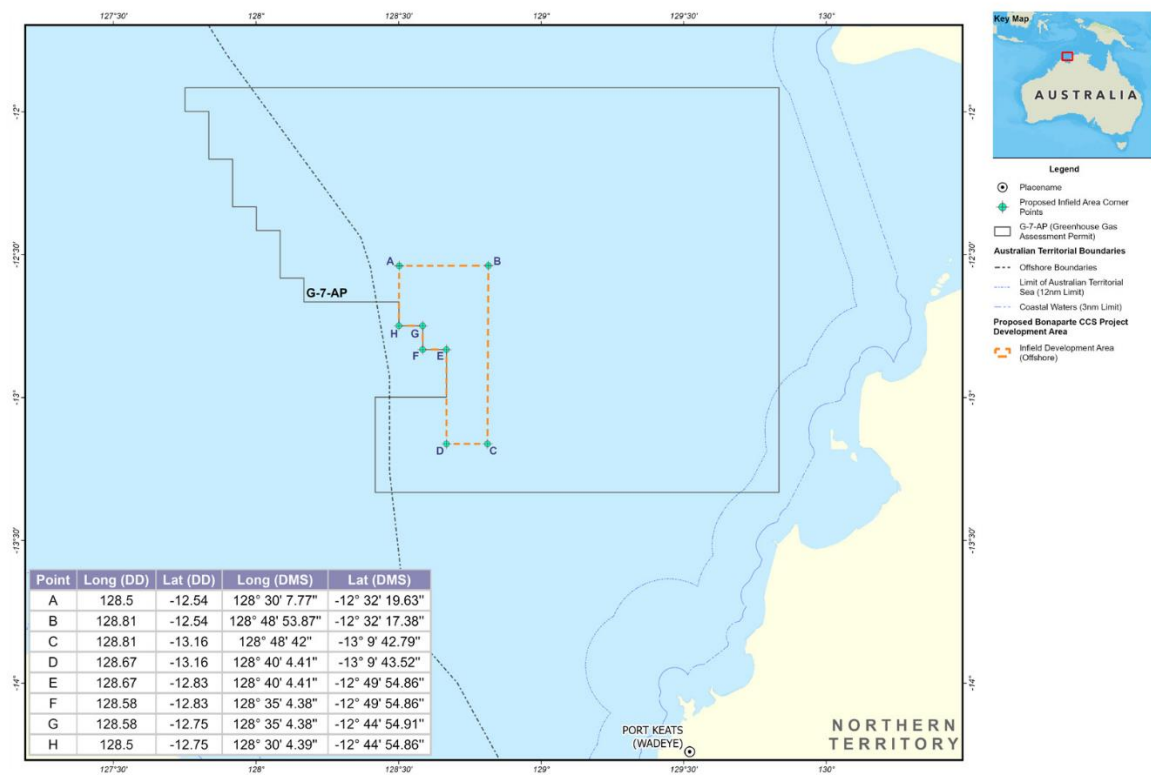
Figure 4: Infield extent area of the proposed Bonaparte CCS Project
