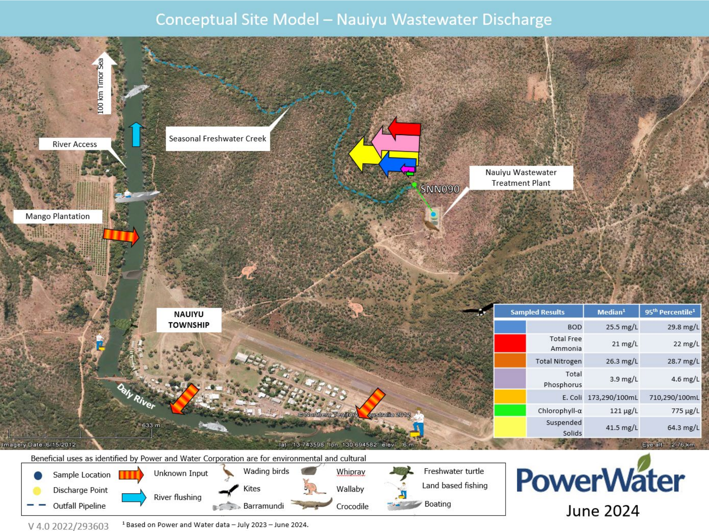
Figure 7: Conceptual site model for the Naiyu WwTP.
