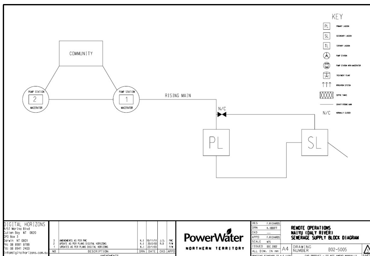
Figure 5: Naiyu wastewater collection and treatment configuration.
