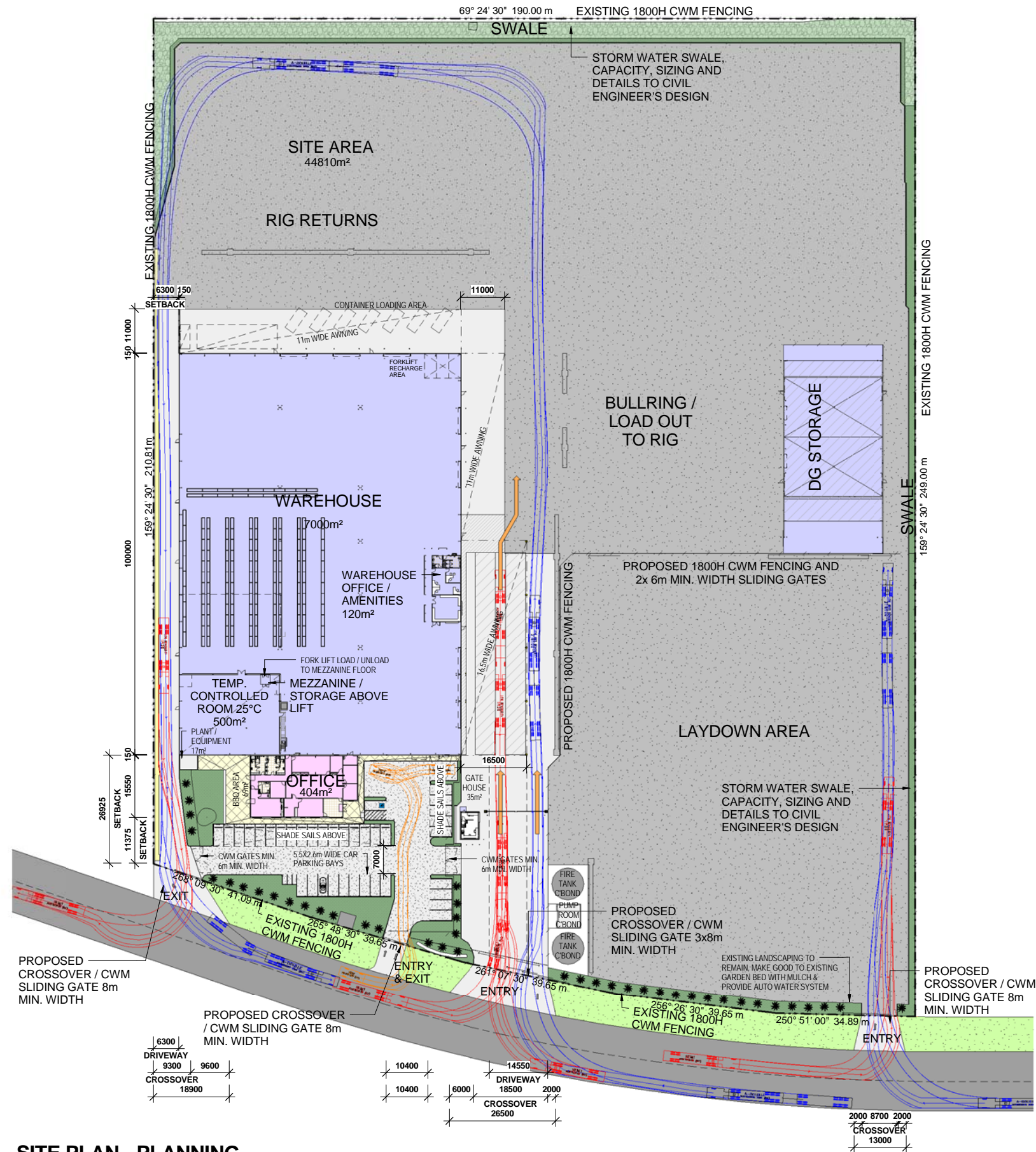
SITE PLAN - PLANNING 1 : 600 @ A1
