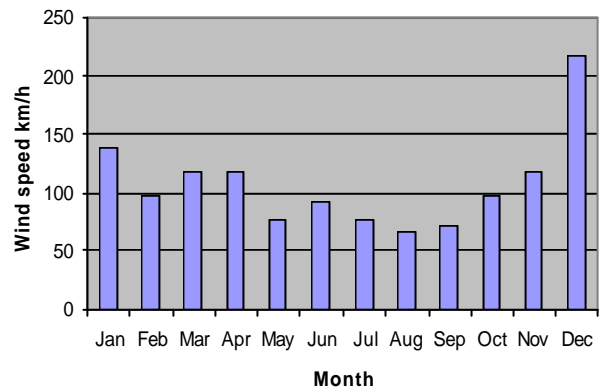
Highest recorded wind gust - km/h - Darwin
