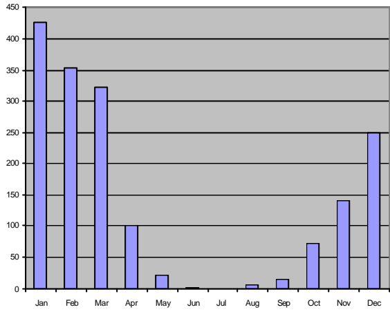
Mean daily evaporation - mm - Darwin
