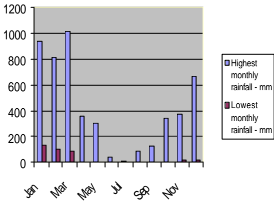
Maximum and minimum monthly rainfalls - Darwin
