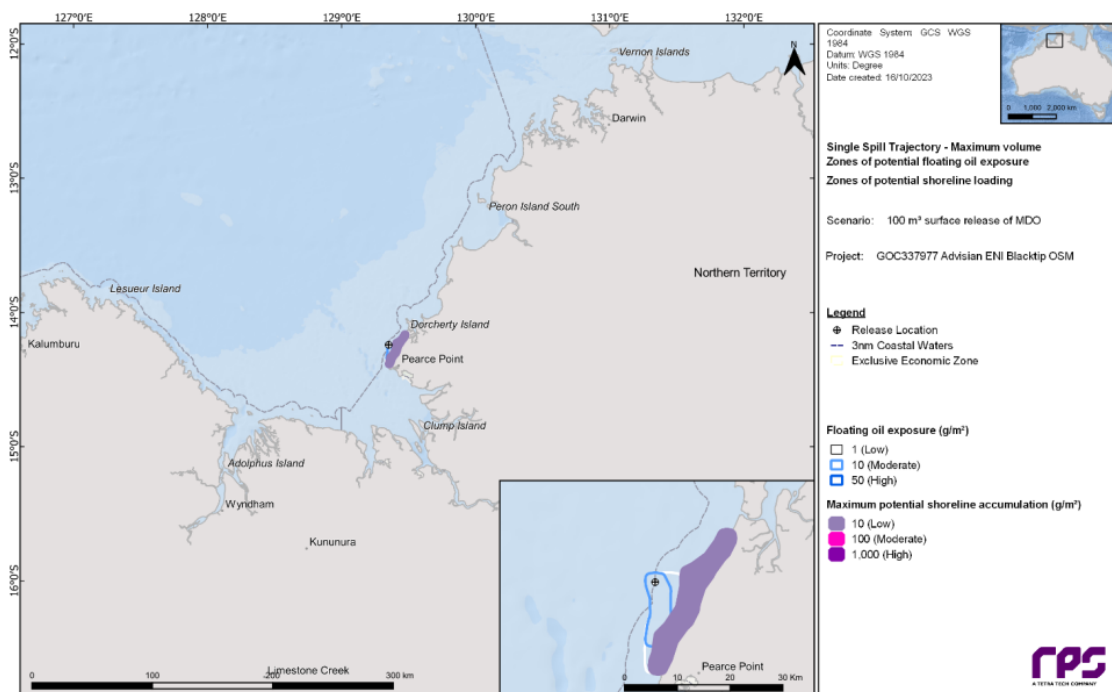
Figure 1.4: Predicted extent of the floating oil exposure and shoreline loading over the entire 30 days for the simulation that led to the longest length of shoreline accumulation above 10 g/m² from a surface vessel spill
