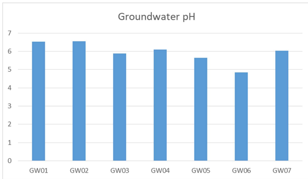
Figure 7: Groundwater pH May 2021
