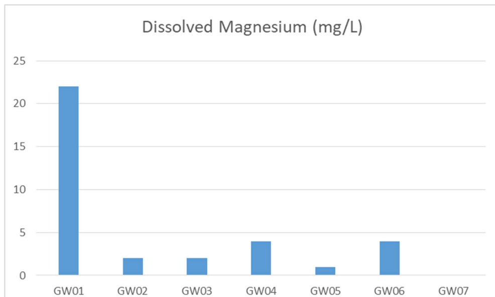
Figure 11: Dissolved Magnesium May 2021
