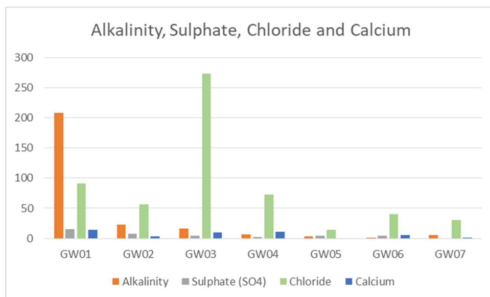
Figure 10: Alkalinity, Sulphate, Chloride and Calcium May 2021
