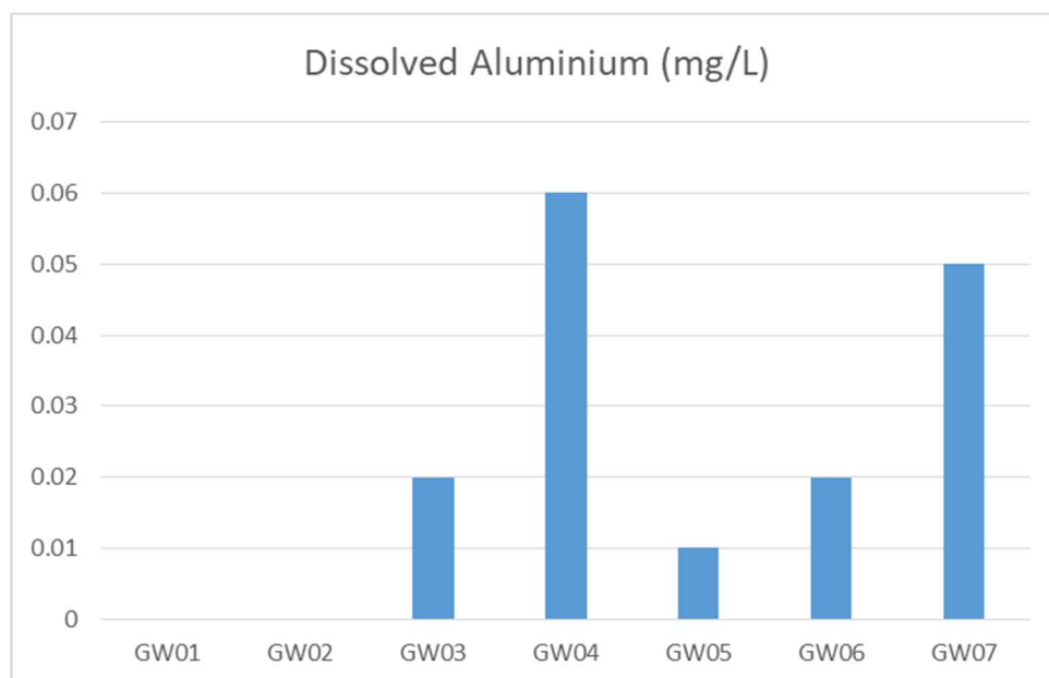
Figure 12: Dissolved Aluminium May 2021
