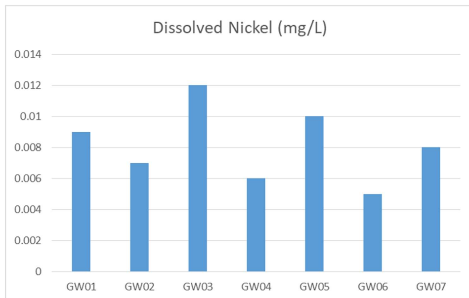
Figure 16: Dissolved Nickel May 2021
