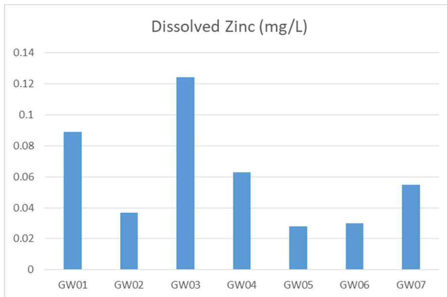
Figure 17: Dissolved Zinc May2021
