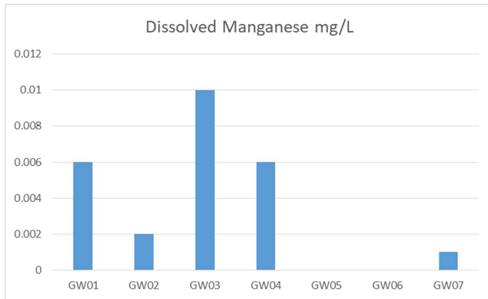
Figure 15: Dissolved Manganese May 2021
