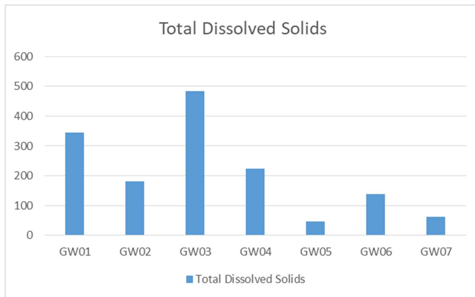
Figure 9: Total Dissolved Solid (TDS) May 2021
