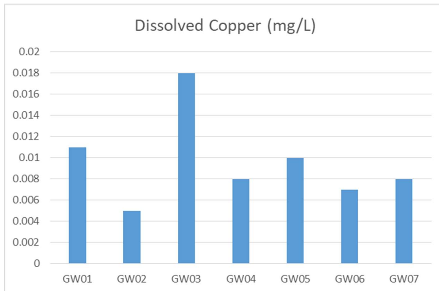
Figure 13: Dissolved Copper May 2021
