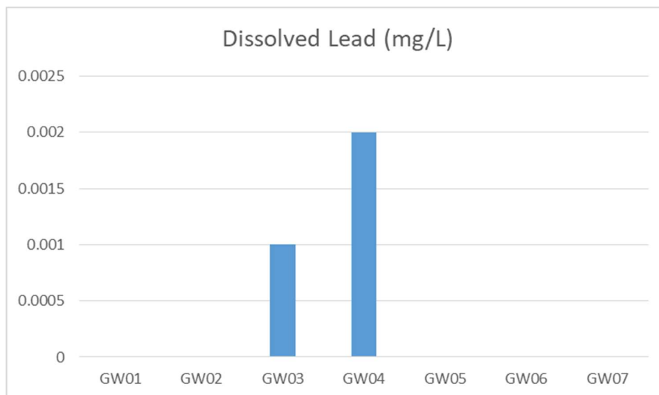
Figure 14: Dissolved Lead May 2021
