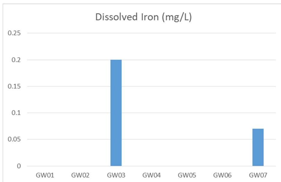
Figure 18: Dissolved Iron May2021
