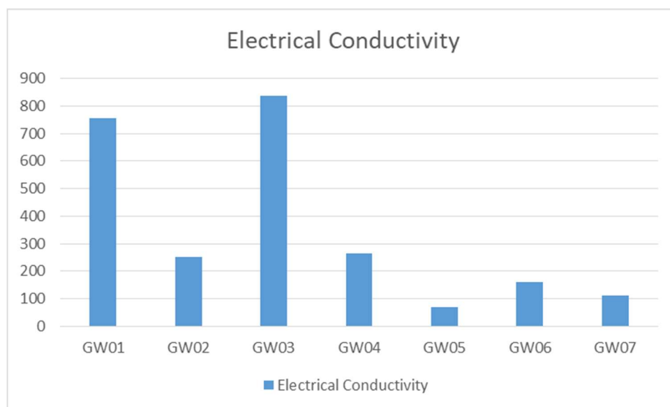
Figure 8: Electrical Conductivity (µS/cm) May 2021
