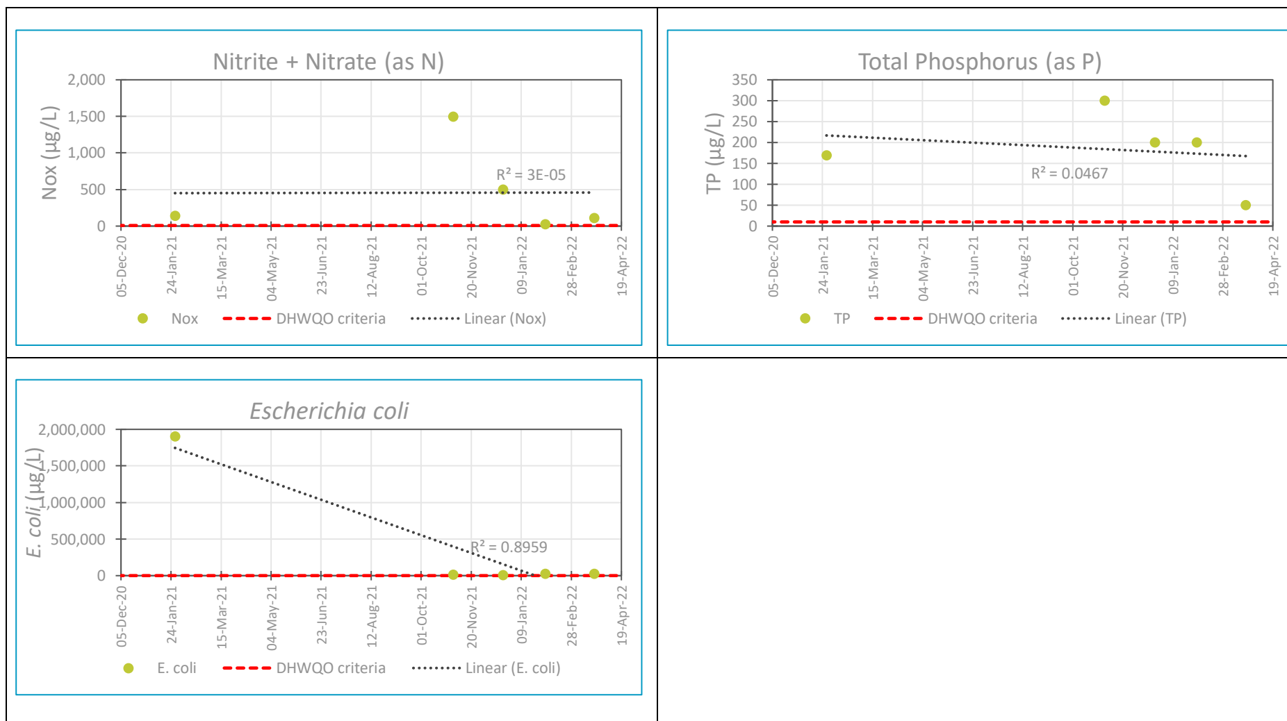
Figure 6 Nutrient and Escherichia coli concentrations in Humpty Doo WTS
