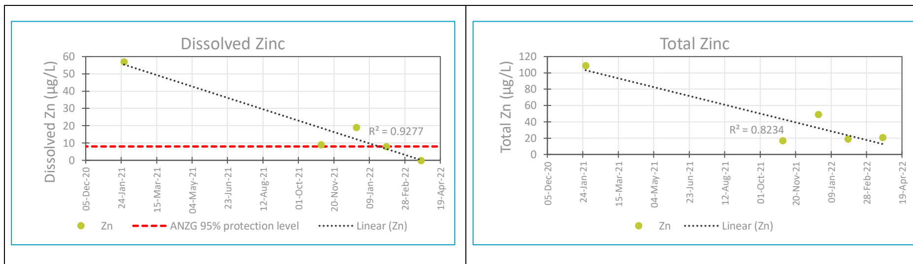
Figure 7 Copper, lead and zinc concentrations in Humpty Doo WTS
