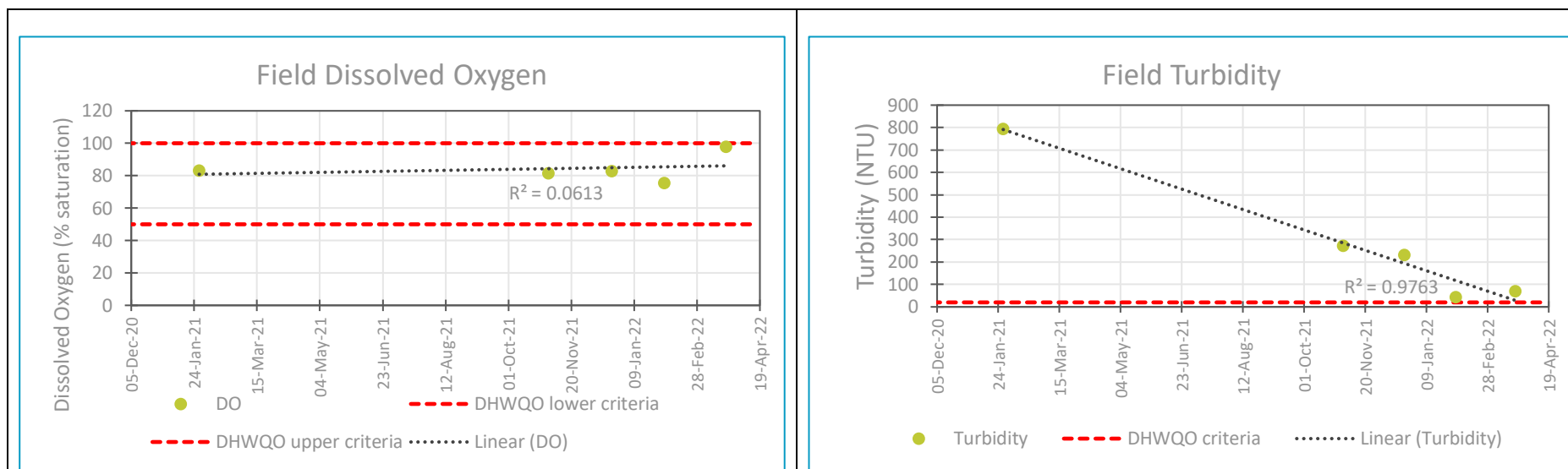
Figure 5 Field water quality measurements in Humpty Doo WTS
