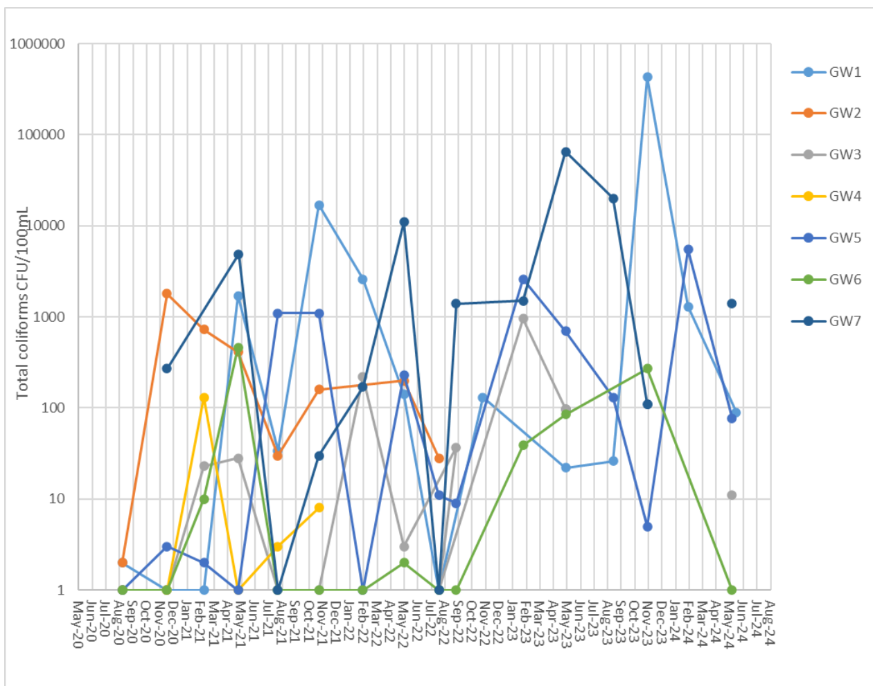
Figure 5-5. Graph of Total coliforms concentrations measured in groundwater since monitoring of this parameter began in 2020 (note logarithmic scale)
