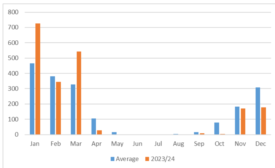
Figure 3-1. Monthly rainfall totals (BoM station 14219)
