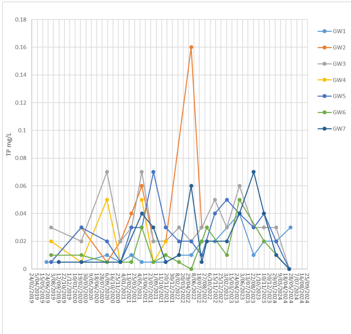
Figure 5-4. Graph of TP concentrations since monitoring began in 2019
