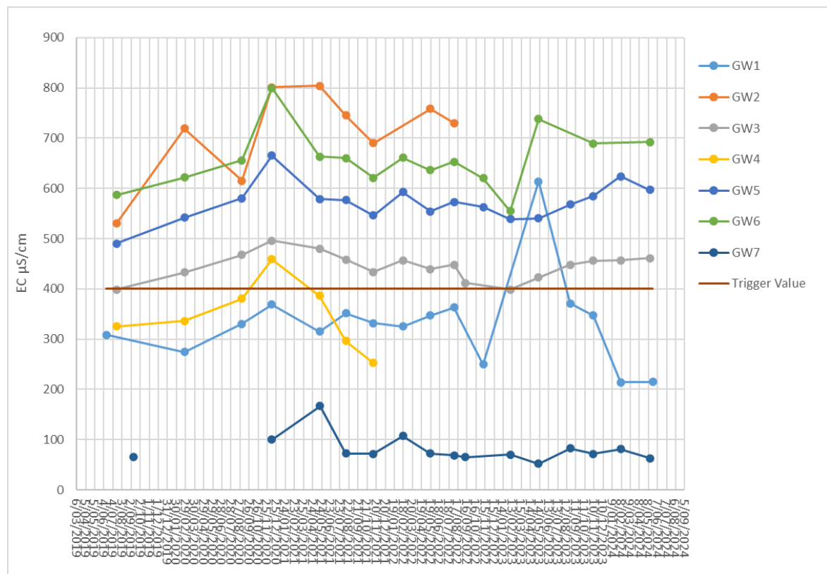
Figure 5-2. Graph of EC measurements in groundwater bores since measuring began in 2019
