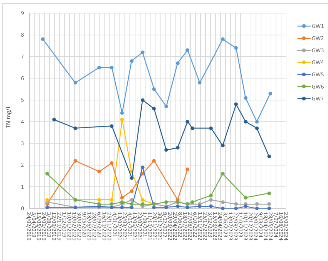
Figure 5-3. Graph of TN concentrations since monitoring began in 2019
