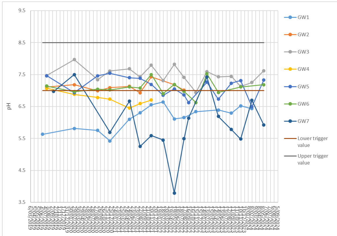
Figure 5-1. Graph of pH values measured in groundwater bores since monitoring began in 2019
