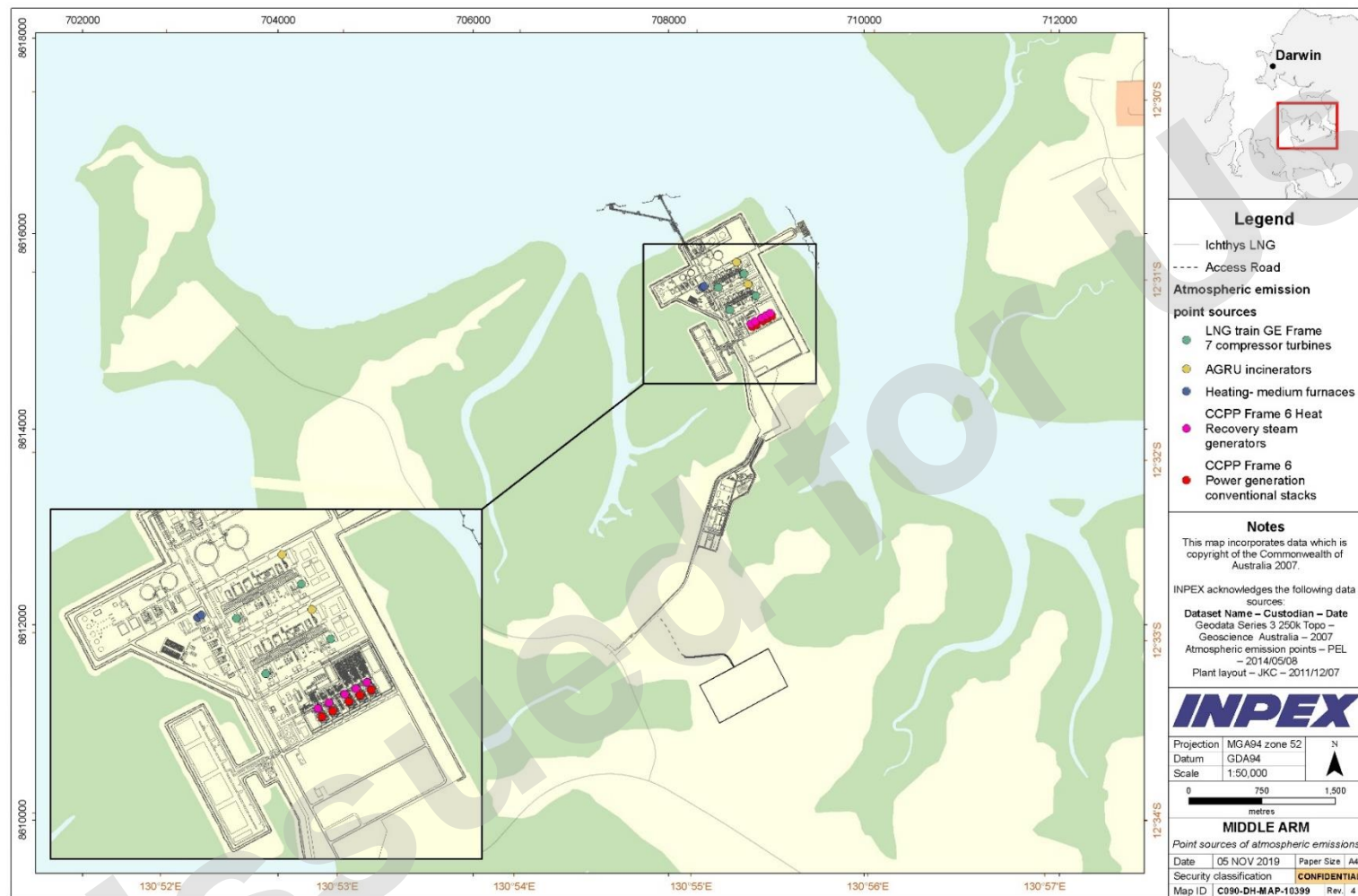
Figure 7-1: Stack emissions monitoring locations
