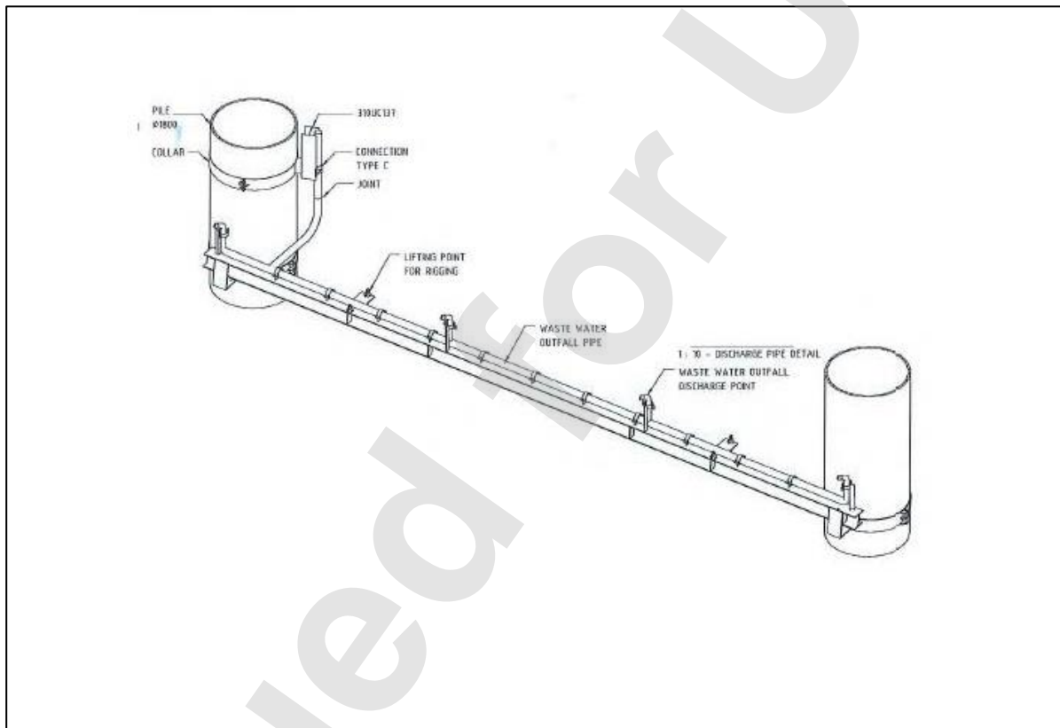
Figure 3-12: Jetty diffuser
