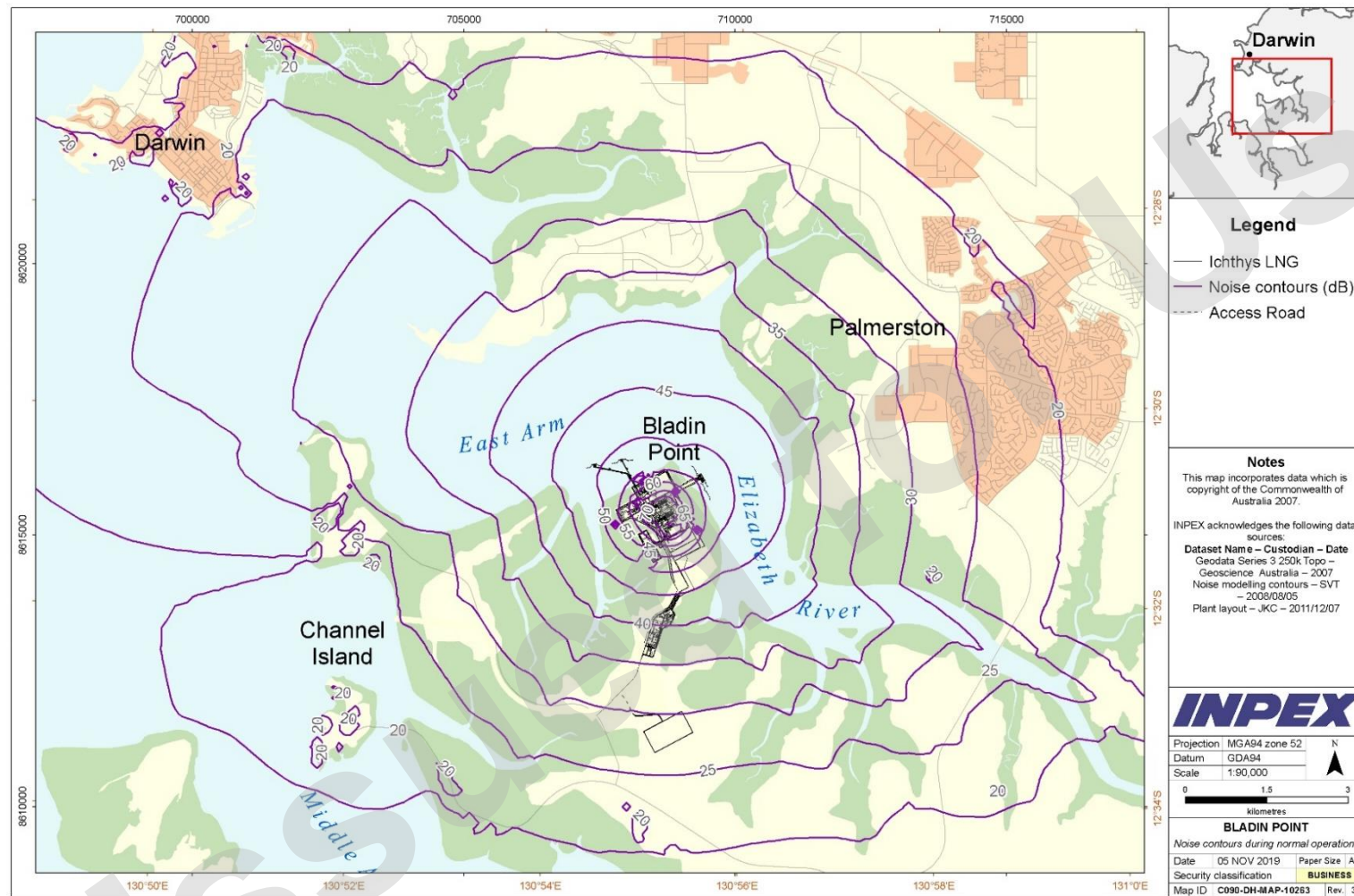
Figure 3-8: Noise contours during normal operations
