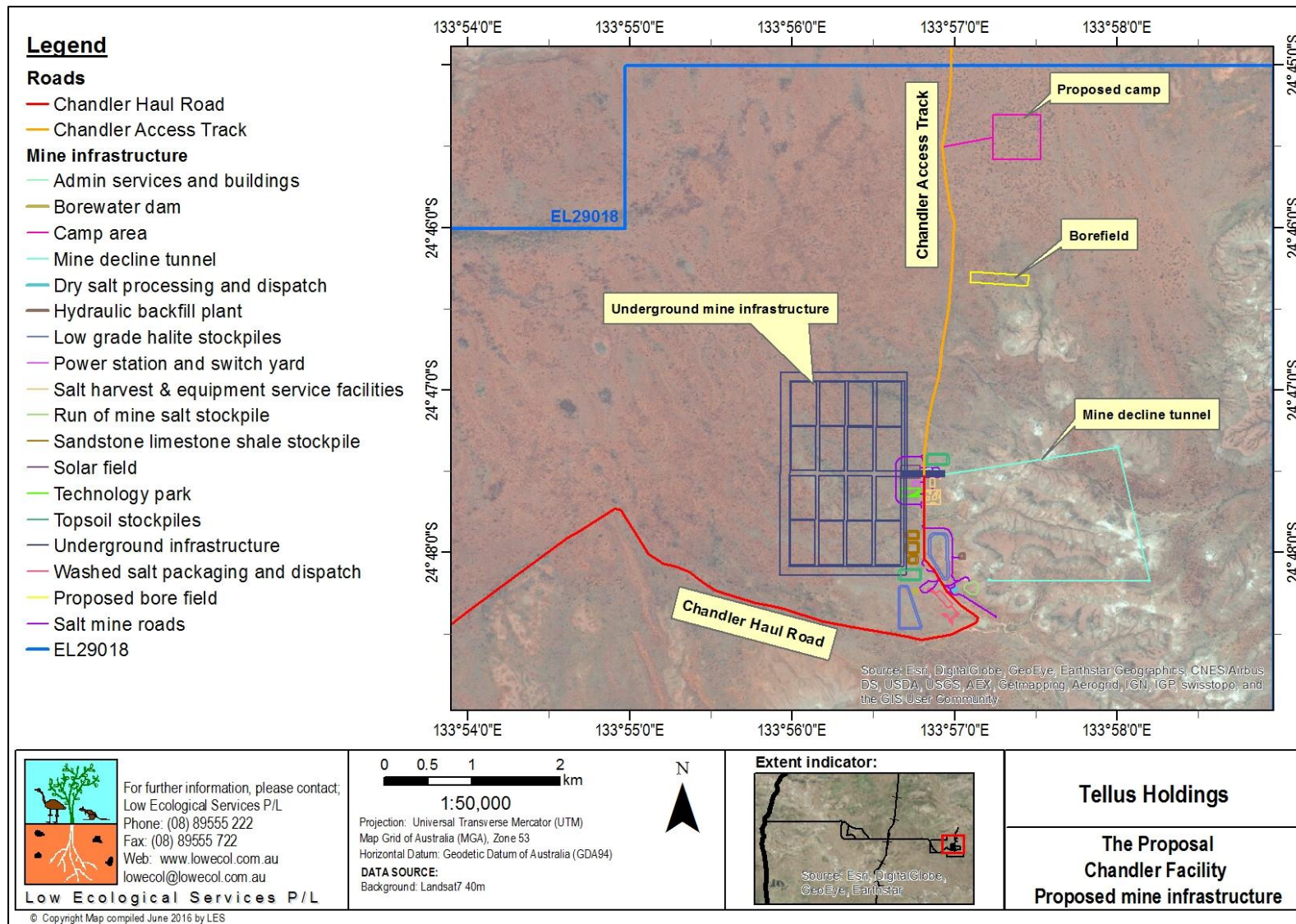
Figure 11-2 Location of the Chandler Facility infrastructure.
