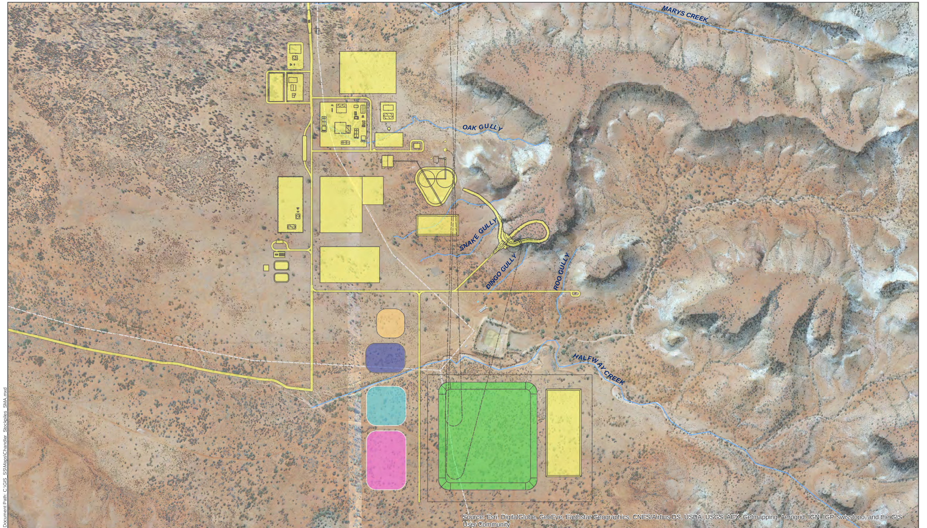
Figure 3-18 Stockpiles including run of mine salt
