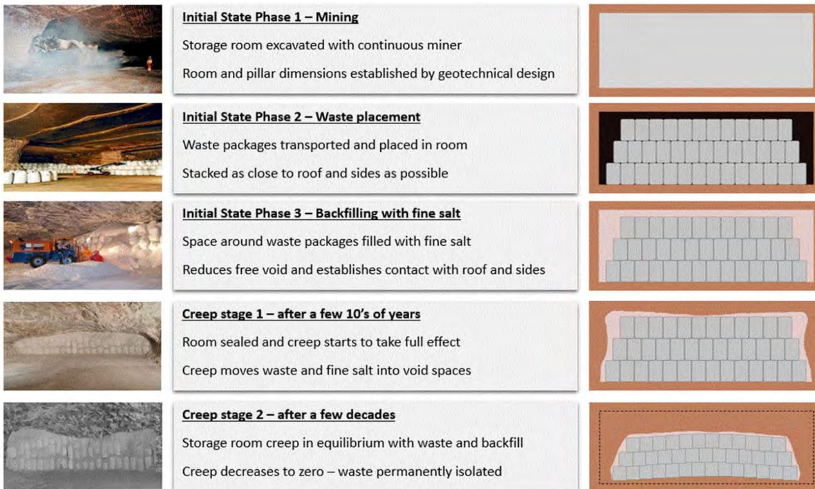
Figure 3-23 Salt creep in excavated room
