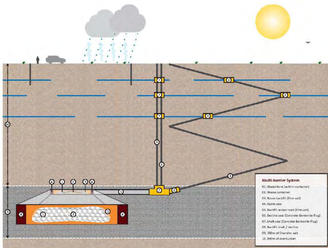
Figure 3-12 Multi-barrier isolation of waste at the Proposed Chandler Facility
