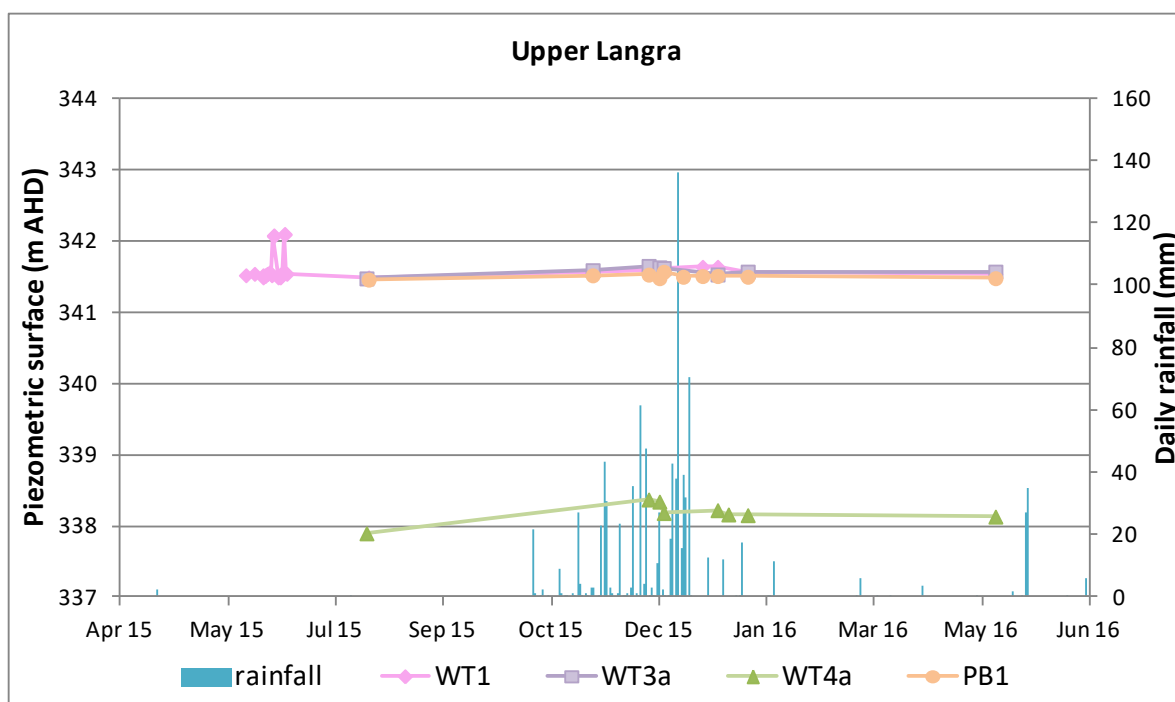
Figure 8-7 Hydrograph for the Upper Langra Formation
