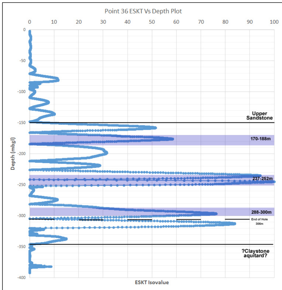
Figure 8-5 Electro seismic hydraulic conductivity tomography across the Proposal area (Geo9 2015)
