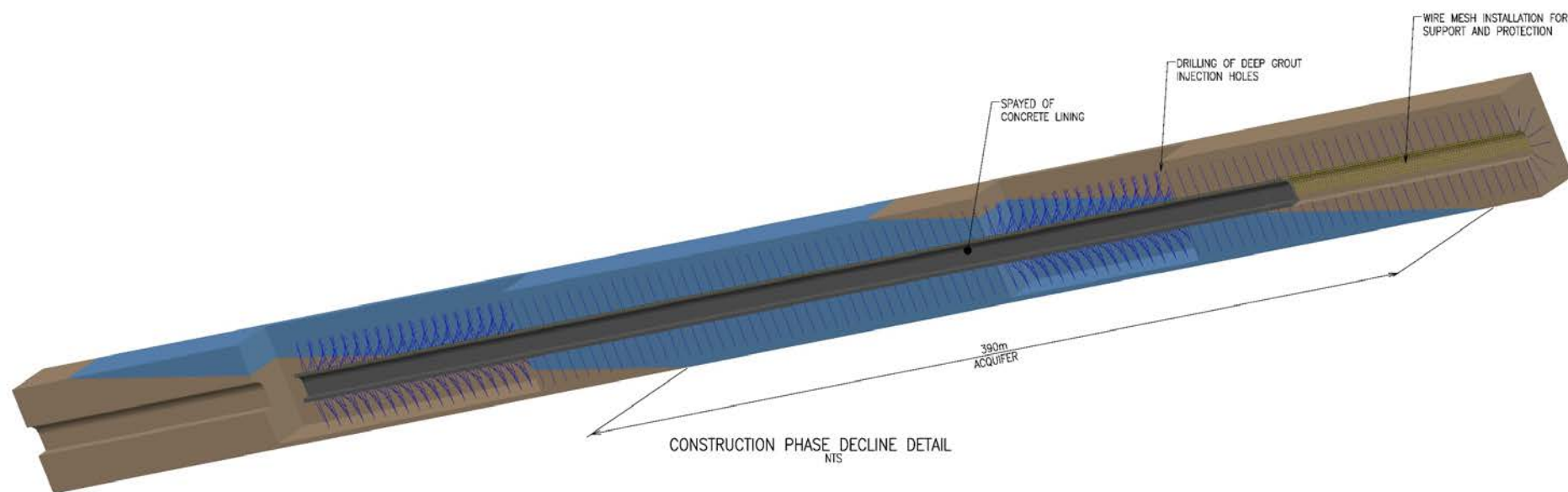
Figure 8-23 Decline sealing techniques during construction
