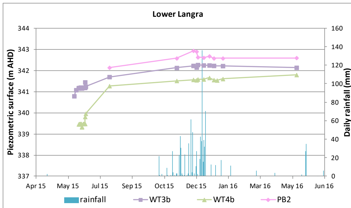
Figure 8-8 Hydrograph for the Lower Langra Formation
