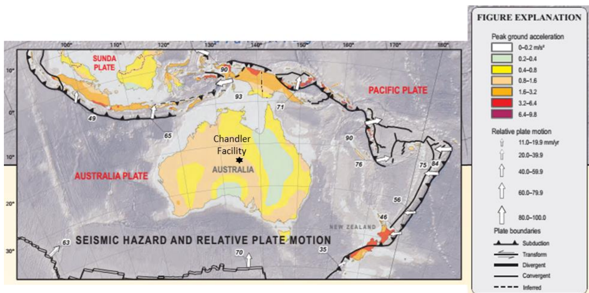
Figure 8-20: Location of the Chandler Facility in the stable interior of the Australian tectonic plate (after Benz et al. 2011).
