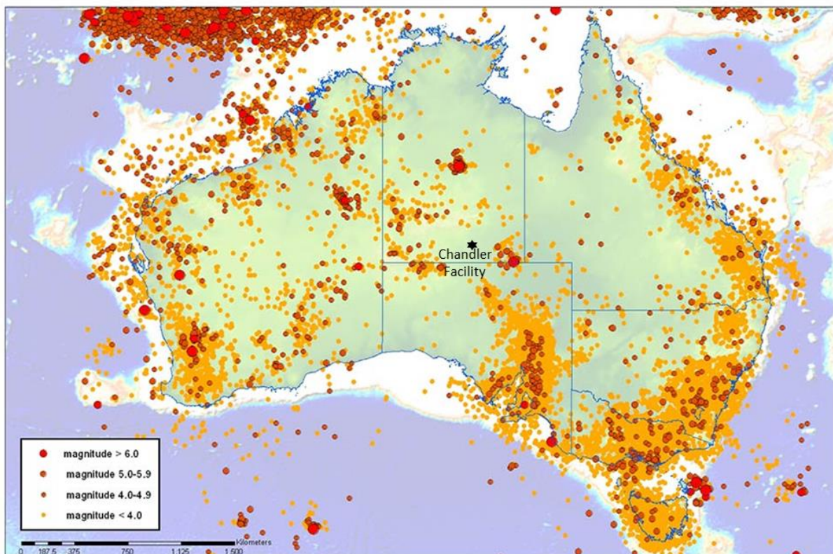
All Australian earthquakes located up to 2011
