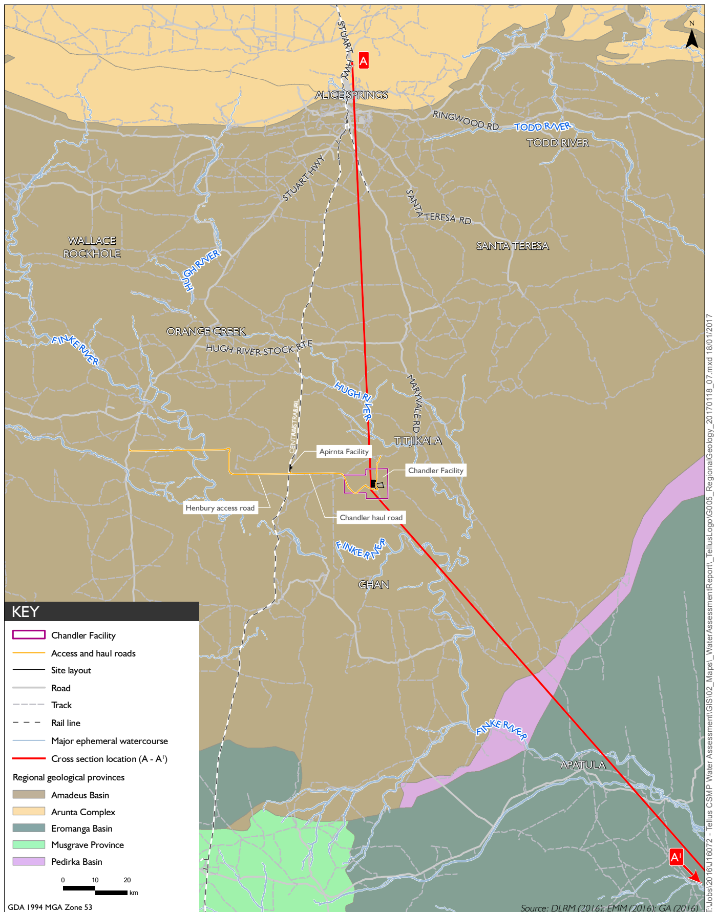
Regional geological provinces
