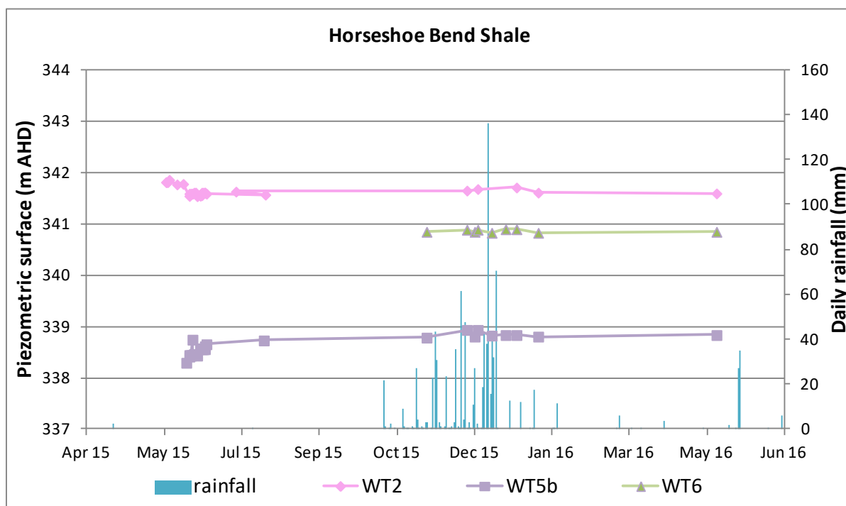
Figure 8-6 Hydrograph for the Horseshoe Bend Shale Formation
