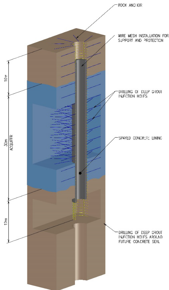
Figure 8-22 Shaft sealing techniques during construction
