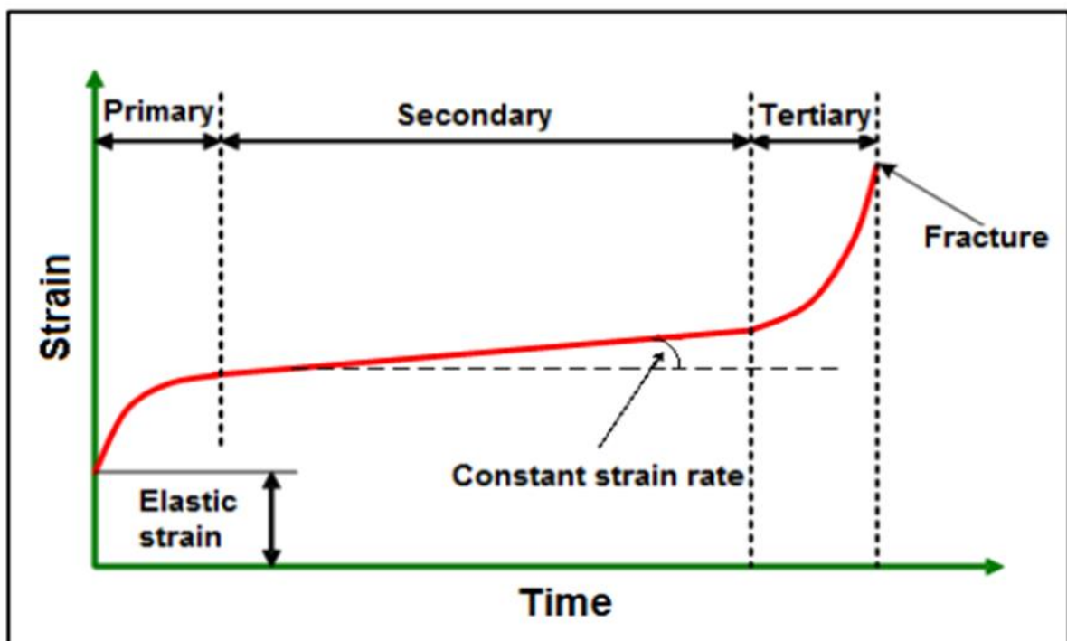
Figure 8-19: The idealised strain-time curve for a creep test - Atkins (2016).
