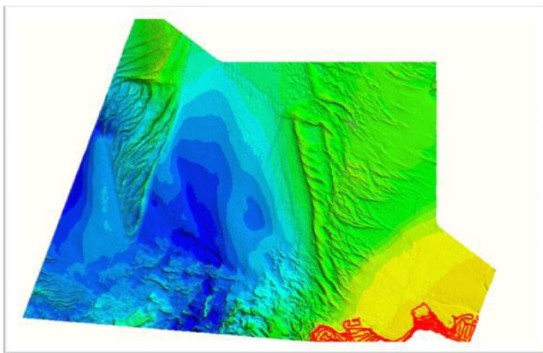
Figure 8 Extent of the East Point topographic survey marked in red.
