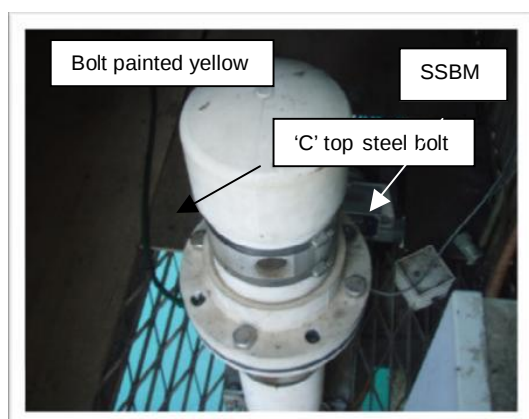
Figure 2 NTC Tide Gauge showing Seaframe Sensor Bench Mark. (Elevation = 6.374m AHD)
