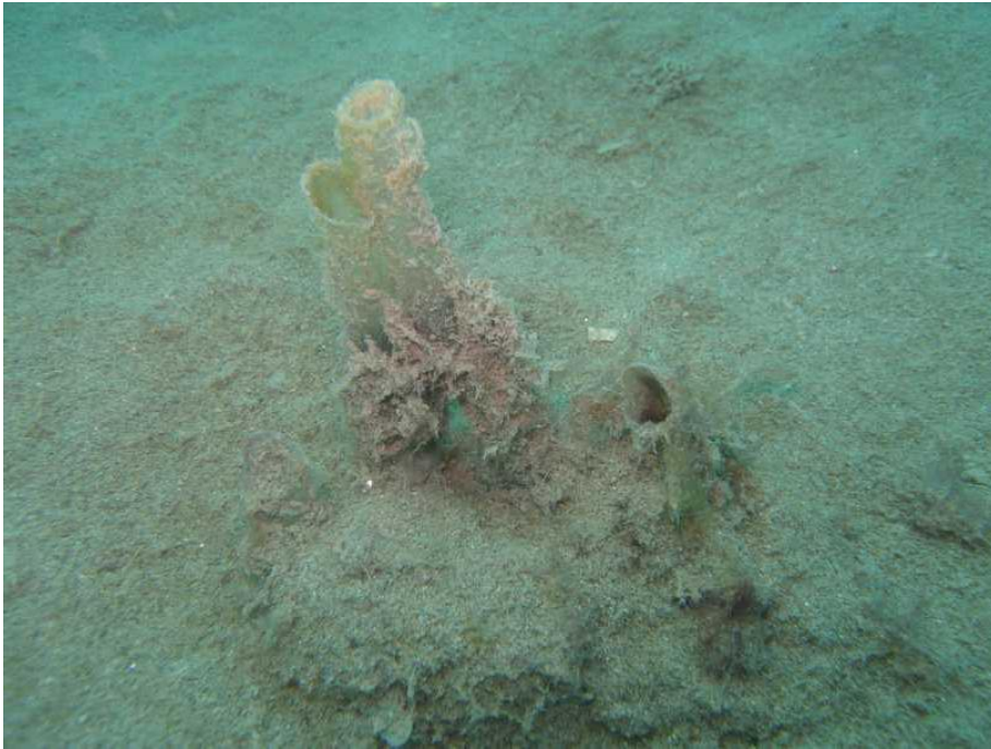
Figure 7 A species of solitary ascidian was the only common benthic organism encountered between sites A10 to A2
