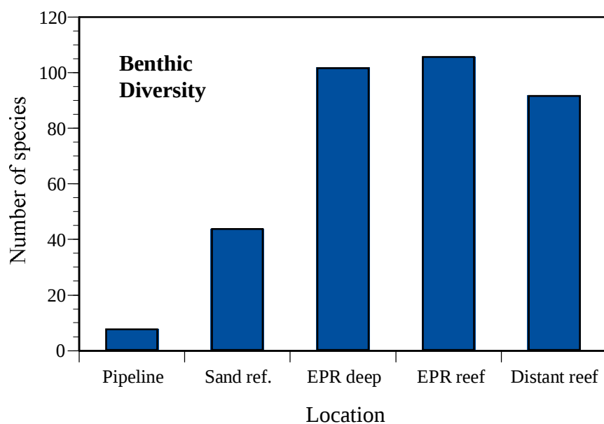
Figure 29 Benthic Diversity Comparison Graph
