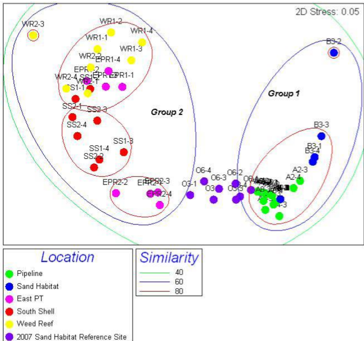
Figure 33 MDS analysis of fauna percentage cover (stress = 0.04)
