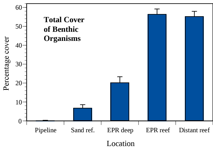
Figure 30 Total Benthic Cover Comparison Graph
