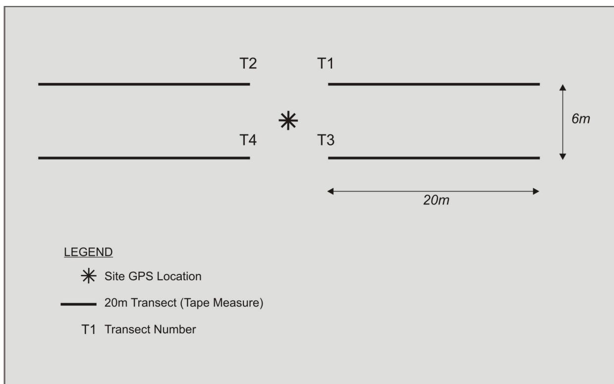
Figure 4 Benthic transect basic set up.
