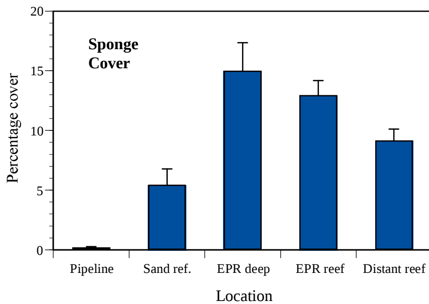
Figure 32 Sponge Cover Comparison Graph
