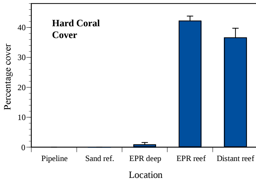
Figure 31 Hard Coral Cover Comparison Graph
