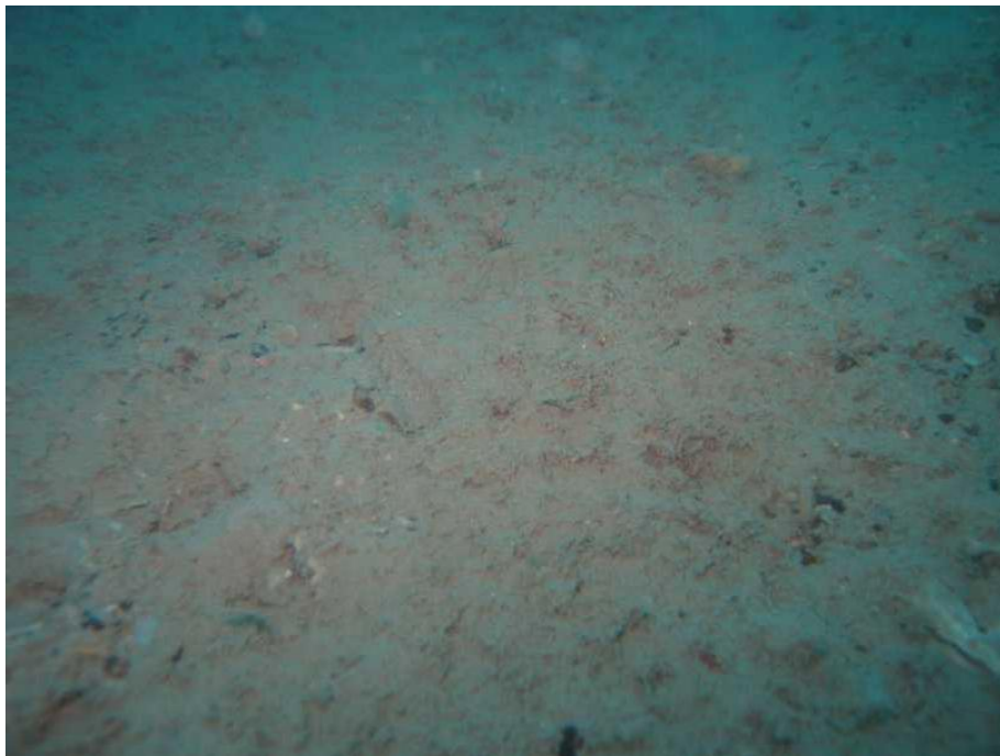
Figure 9 Silty substrate type observed within the deeper basin of the preferred pipeline corridor (site: A6)
