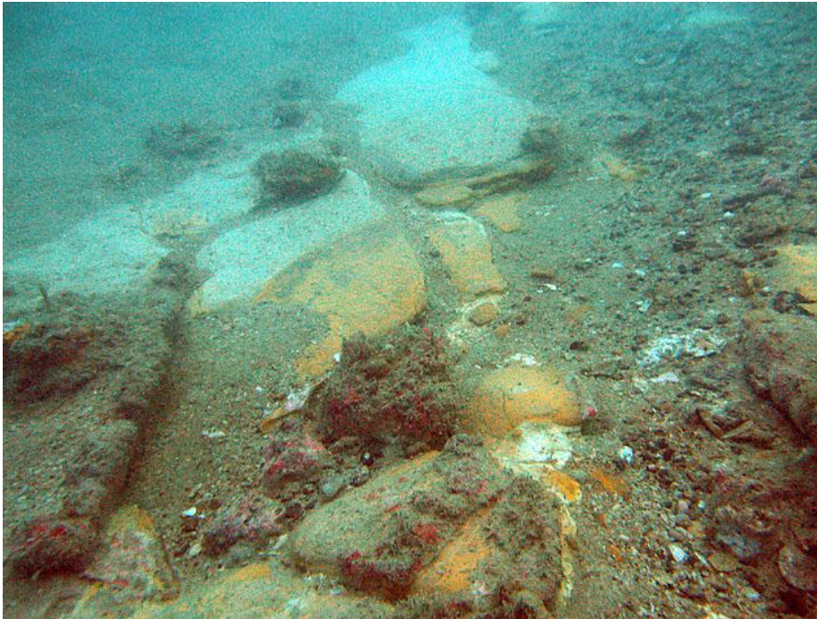
Figure 16 Exposed rock basement between sand waves at Outfall 6
