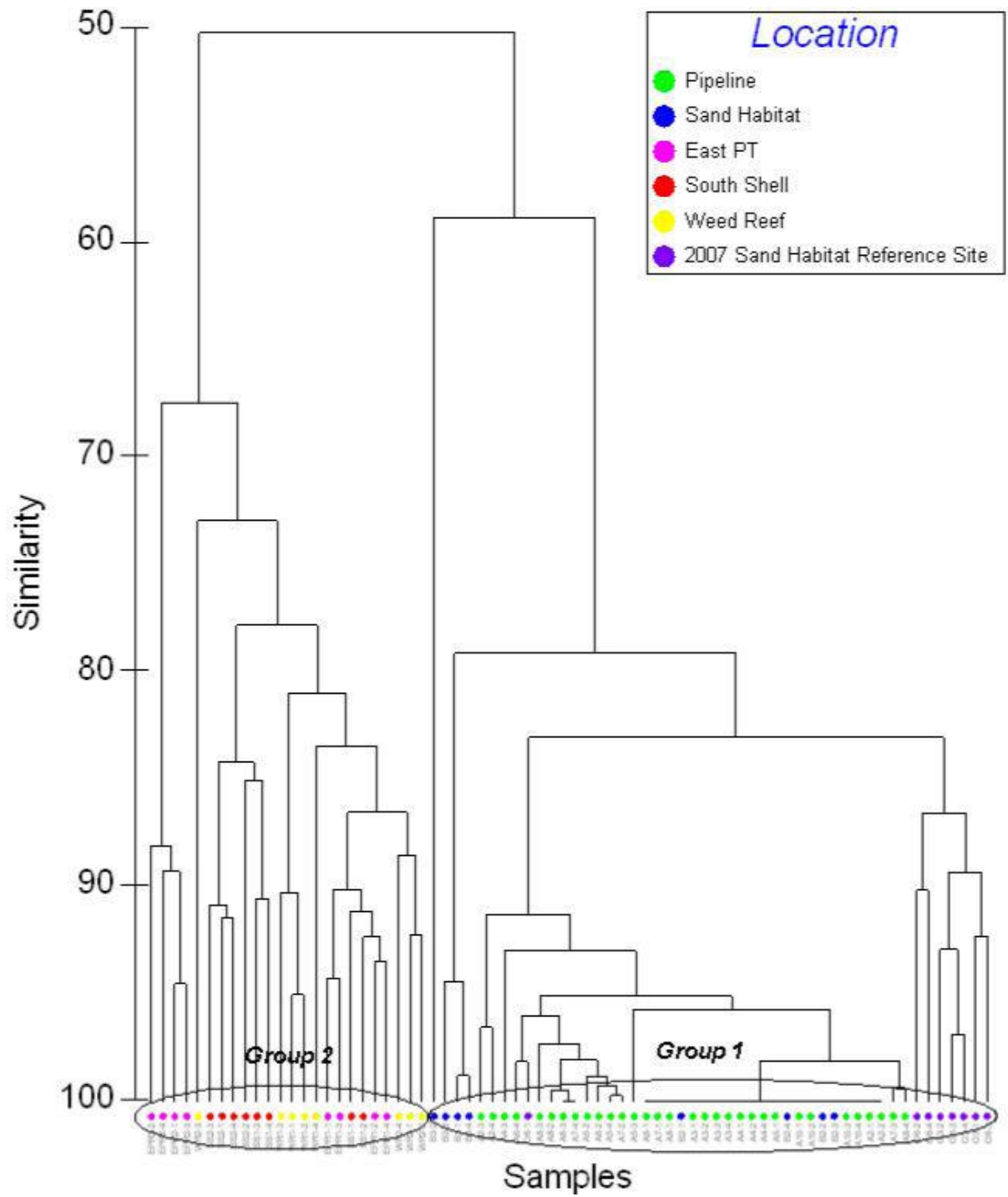
Figure 34 Cluster analysis of fauna percentage cover
