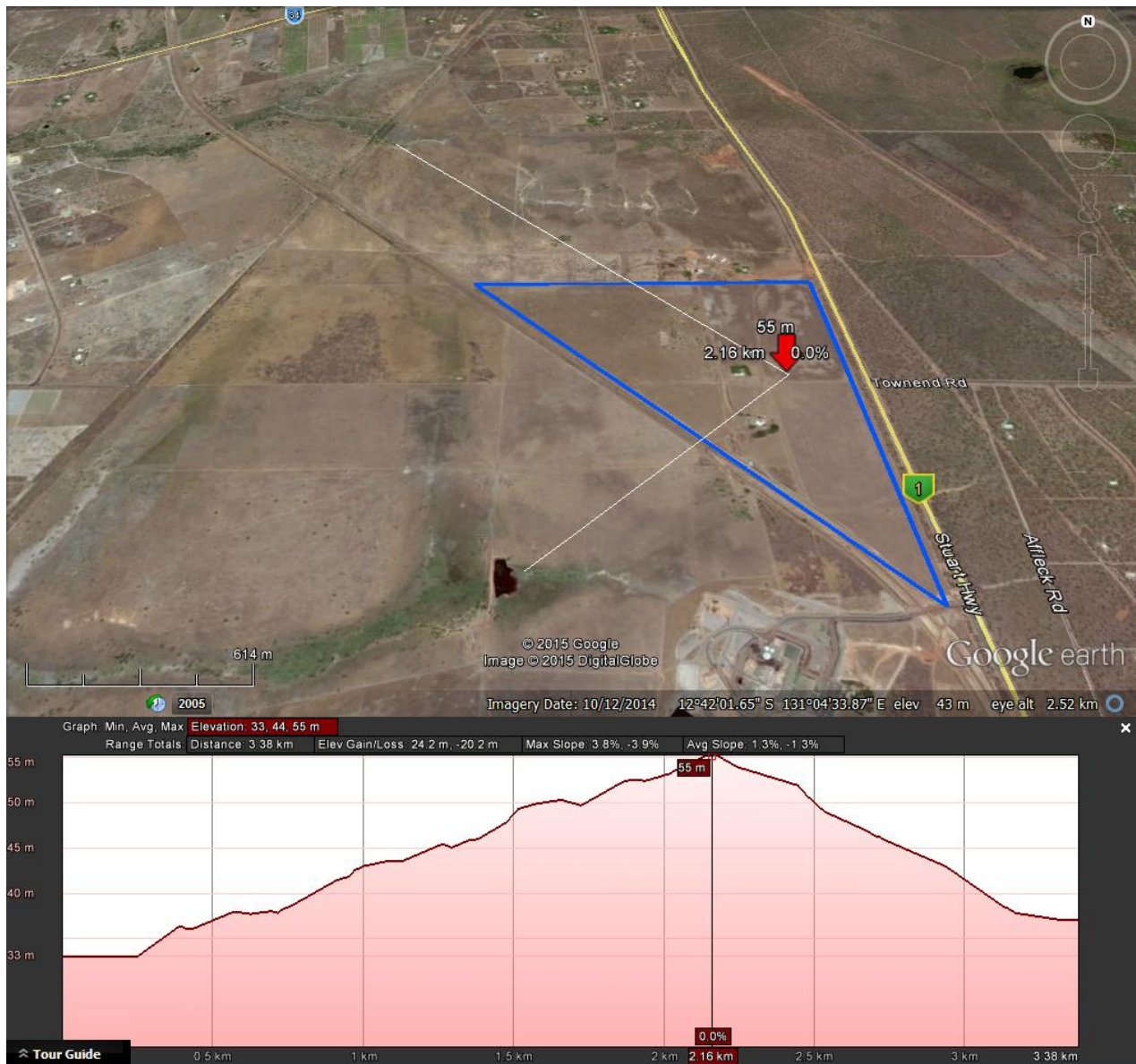
Figure 2 Topographic cross section plan from irrigation area midpoint to nearest watercourses
