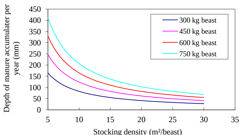
Figure 10 Depth of manure accumulated annually at various stocking densities of cattle of various live-weights (Watts et al., 1994)
