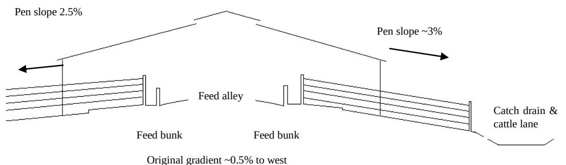
Figure 5 Notional north (left) south (right) transect (not to scale) through a row of “back-to-back” ILEF pens showing location of roof, feed alleys and catch drains.
