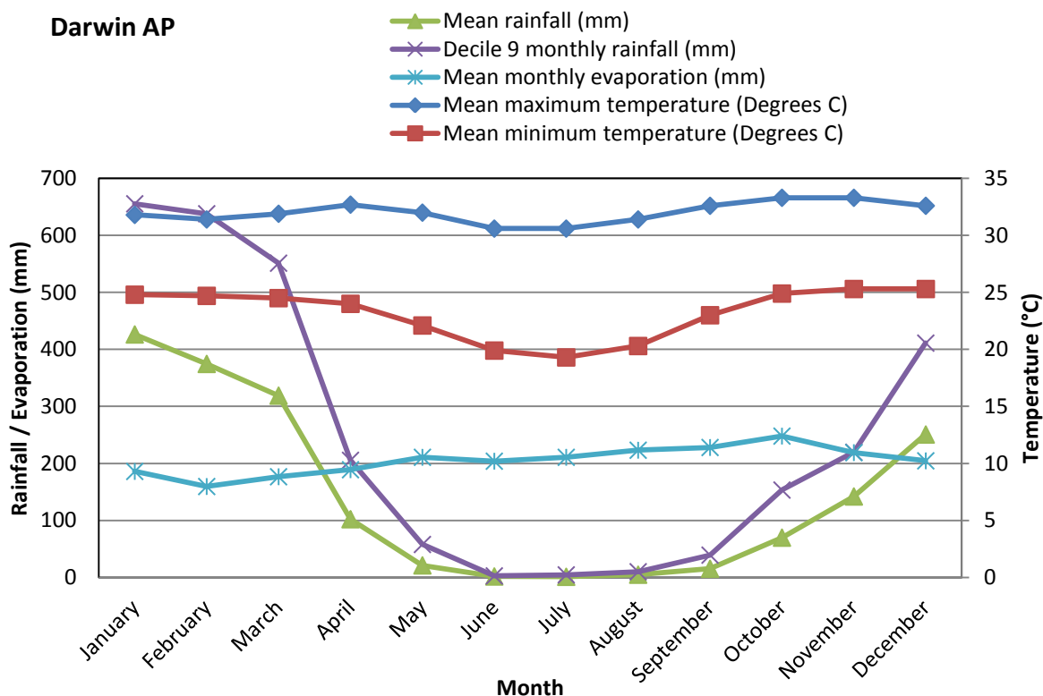
Figure 13 Graph of Temperature and Rainfall and Evaporation for Darwin AP
