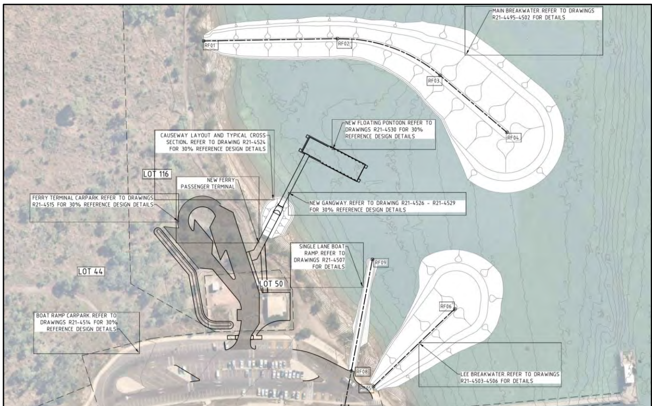
Figure 2-1 Project infrastructure layout (extract from design drawing R21-4488)
