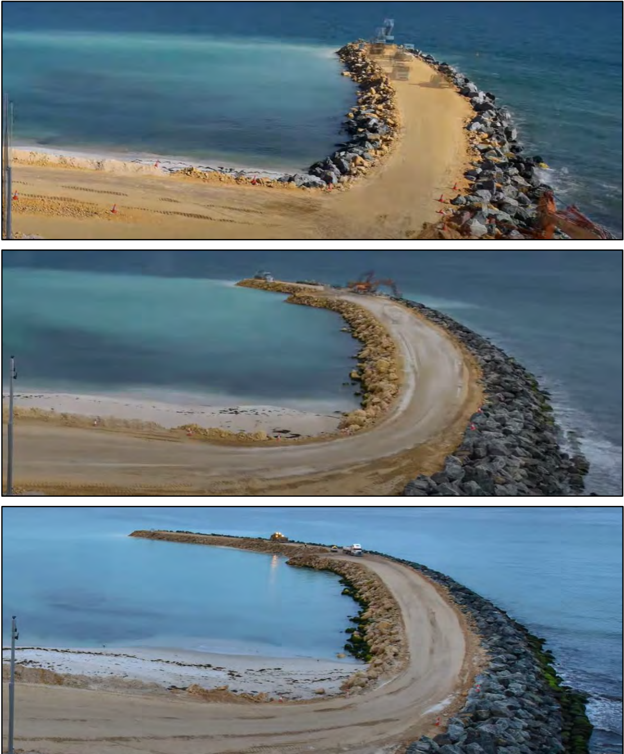
Figure 2-5 Example of staged breakwater construction (Ocean Reef Marina – DevelopmentWA, 2021)
