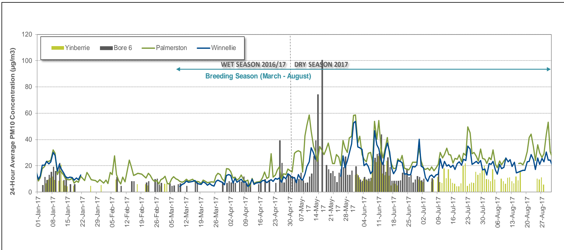
Figure A4 24-Hour Average PM 10 Concentrations Recorded at Mt Todd Compared to Winellie and Palmerston (January 2017 – August 2017)
