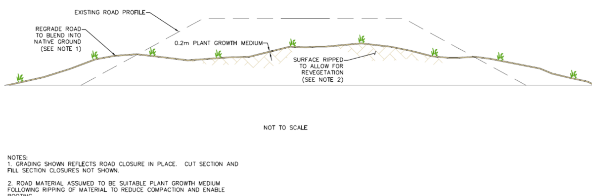
Figure 4-6 Proposed Cover Design for Mine Road Close Out
