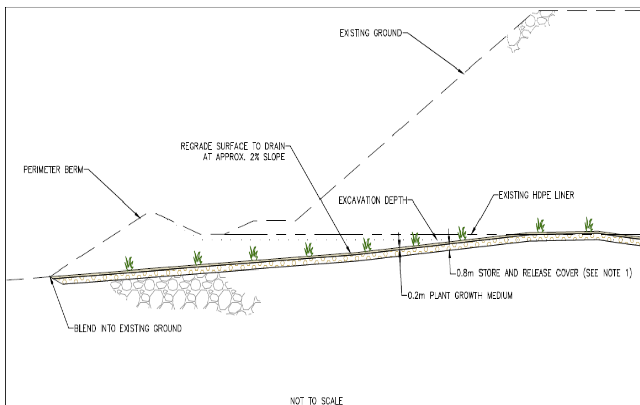
Figure 4-1 Closure Cover Design of the HLP
