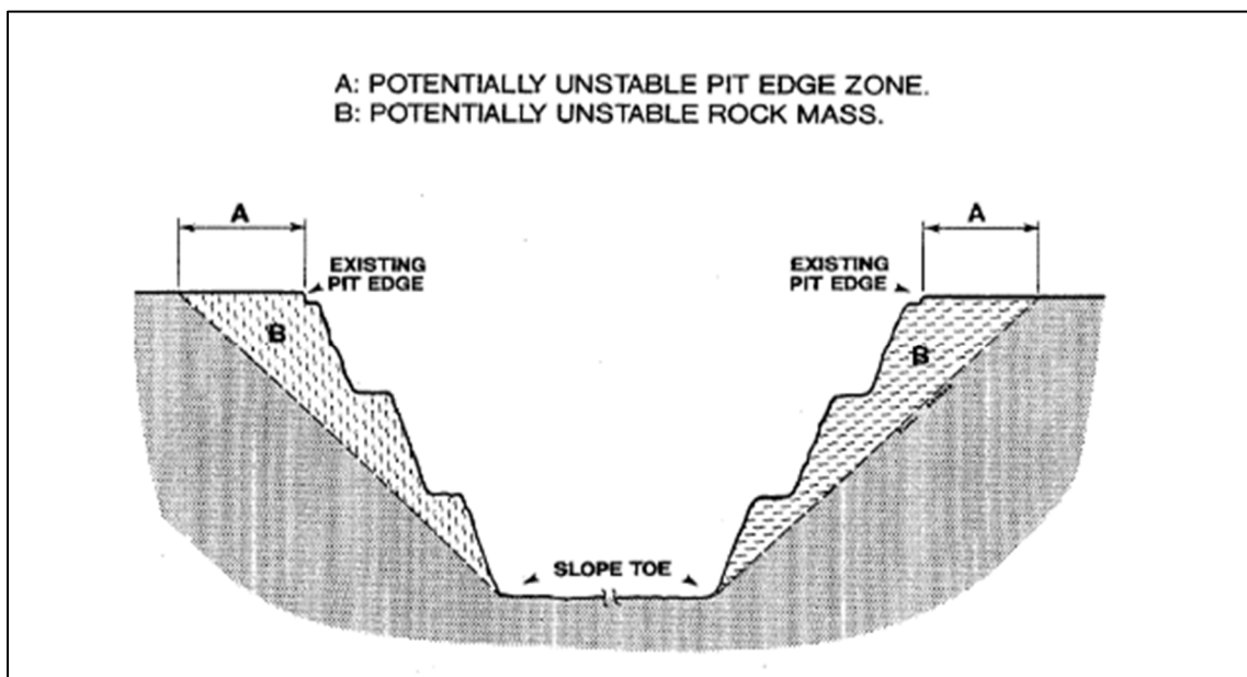
Figure 4-3 Potential Instability Zones (DIR 1997)
