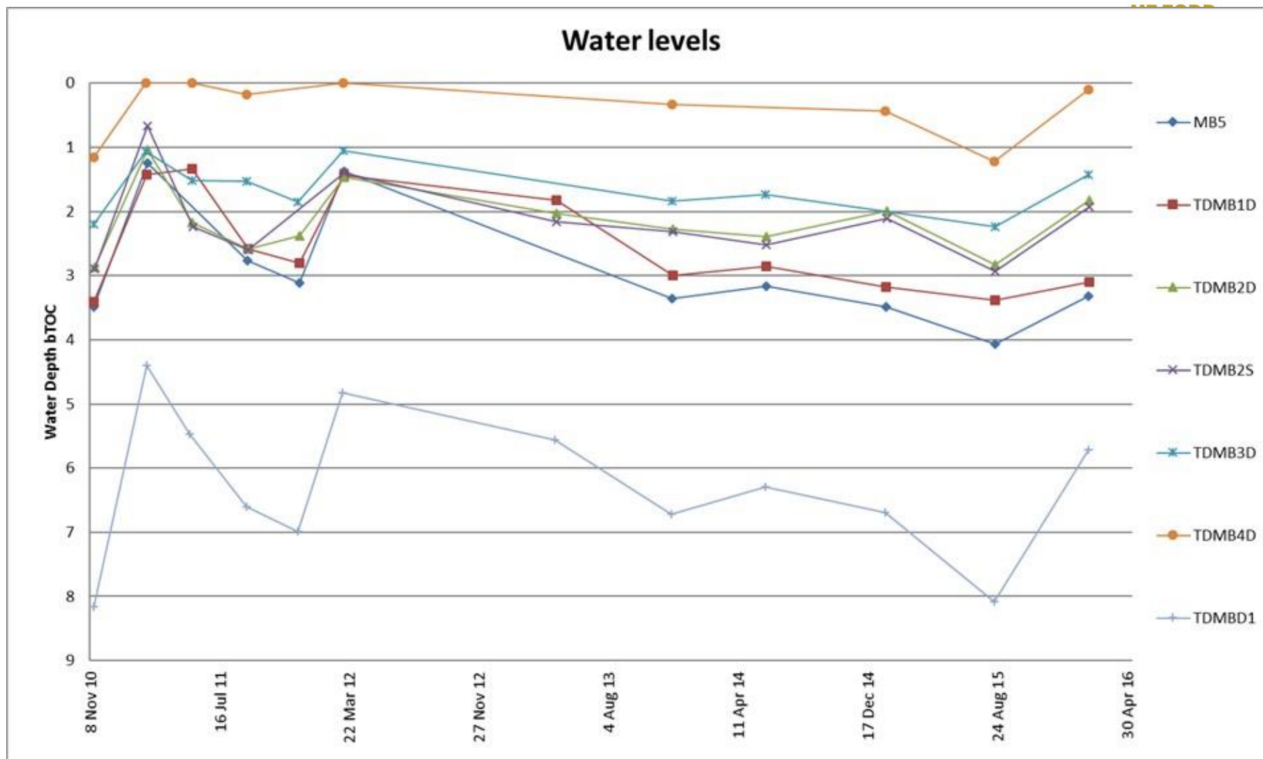
Figure 10-12 Group 3 Water Levels
