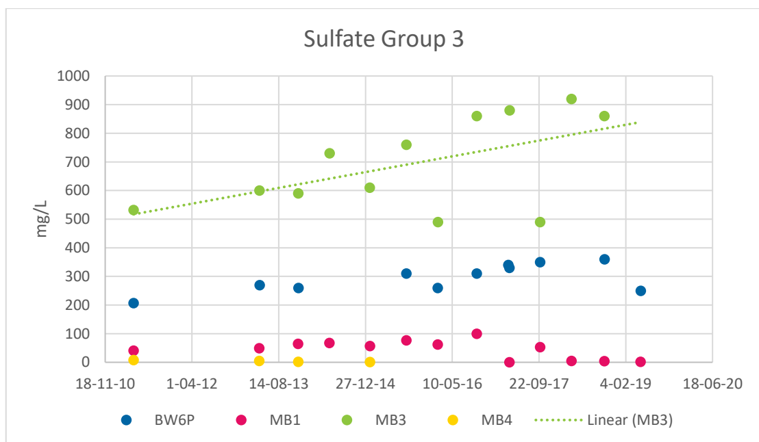
Figure 10-6 Group 3 Sulfate
