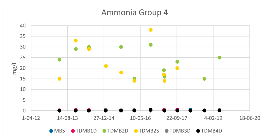
Figure 10-7 Group 4 Ammonia
