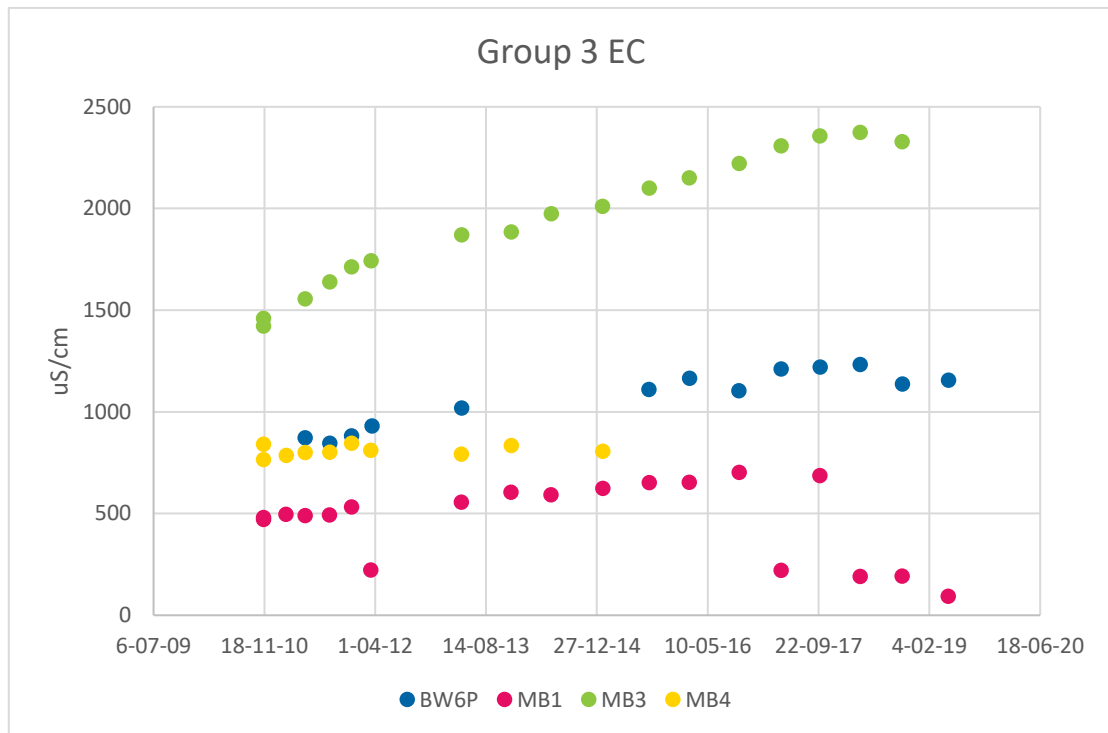
Figure 10-5 Group 3 EC
