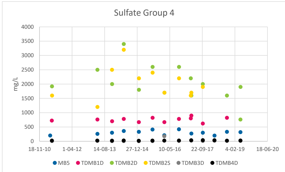
Figure 10-9 Group 4 Sulfate
