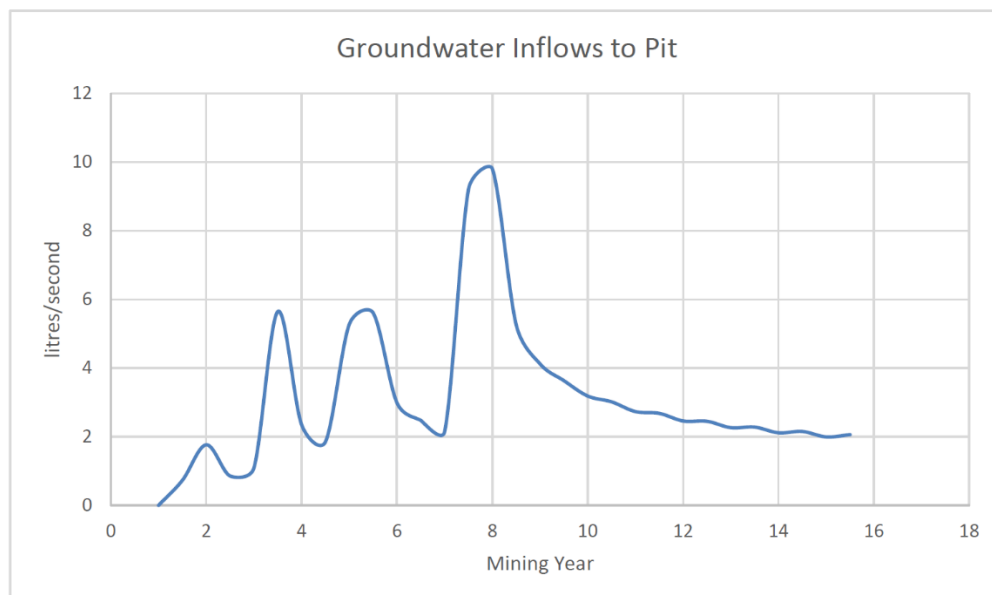
Figure 3-1 Predicted groundwater inflows to Batman Pit
