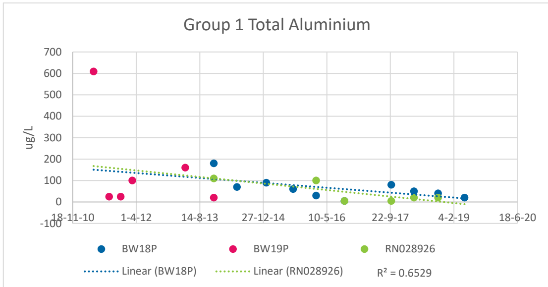
Figure 10-1 Total aluminium Group 1
