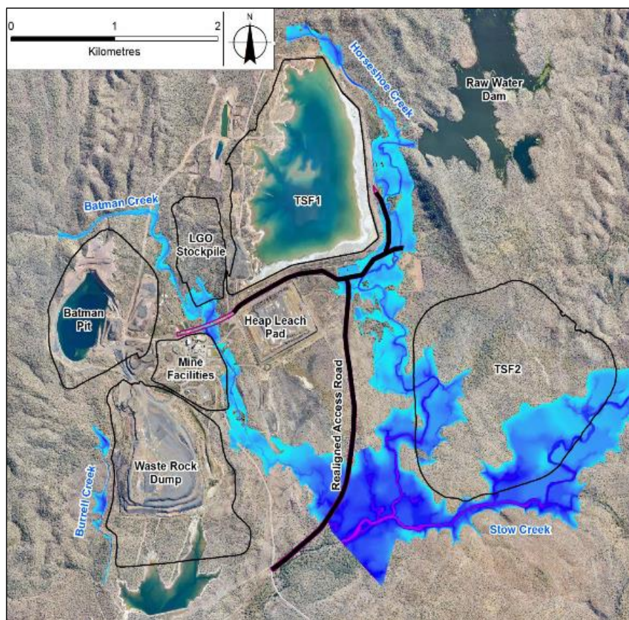
Figure 2-8 Modelled 100-year ARI Flood Extent
