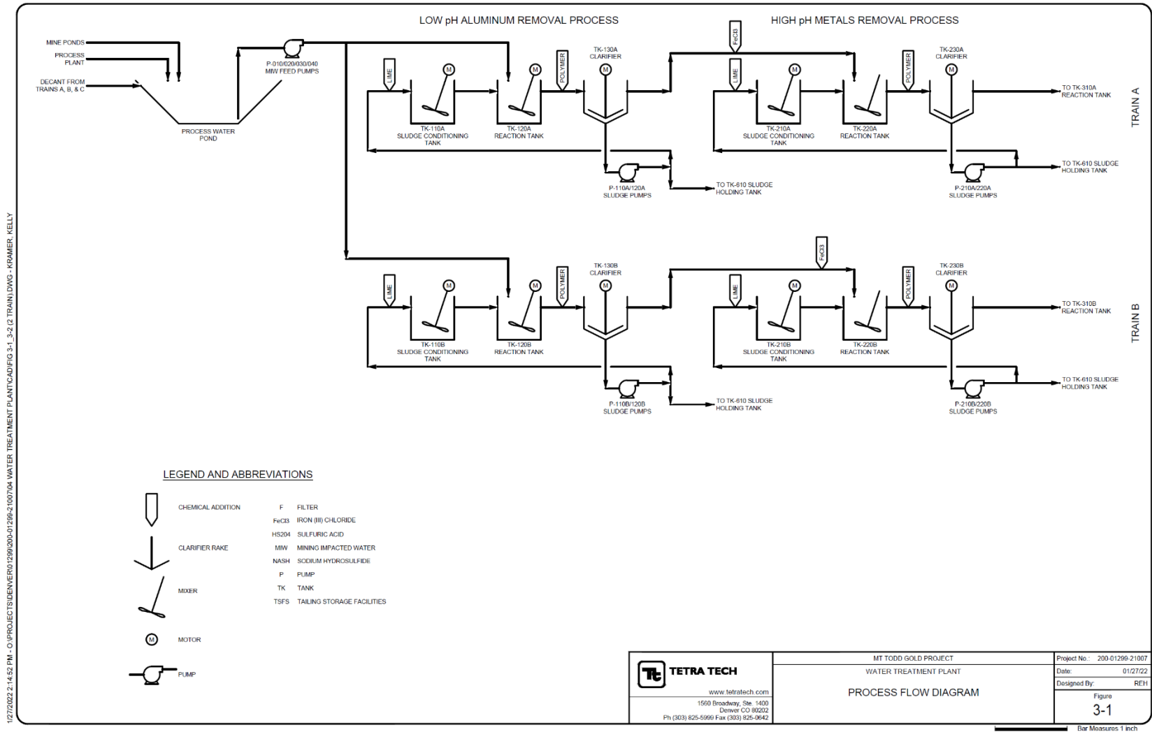
Figure 2-6 WTP Process 1 of 2
