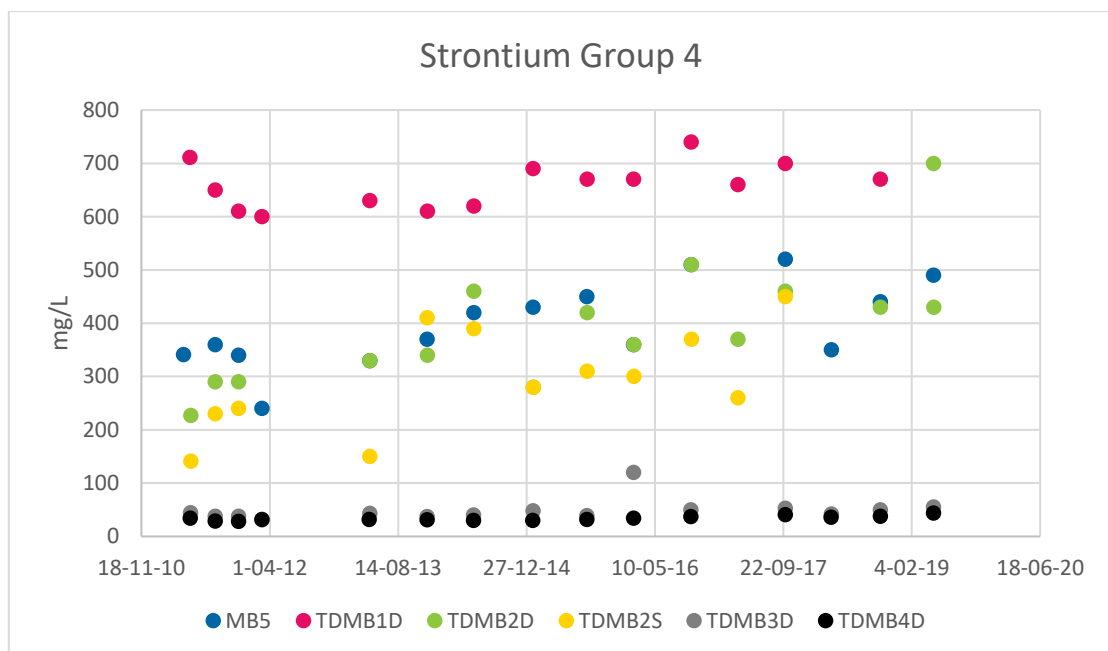
Figure 10-8 Group 4 Strontium
