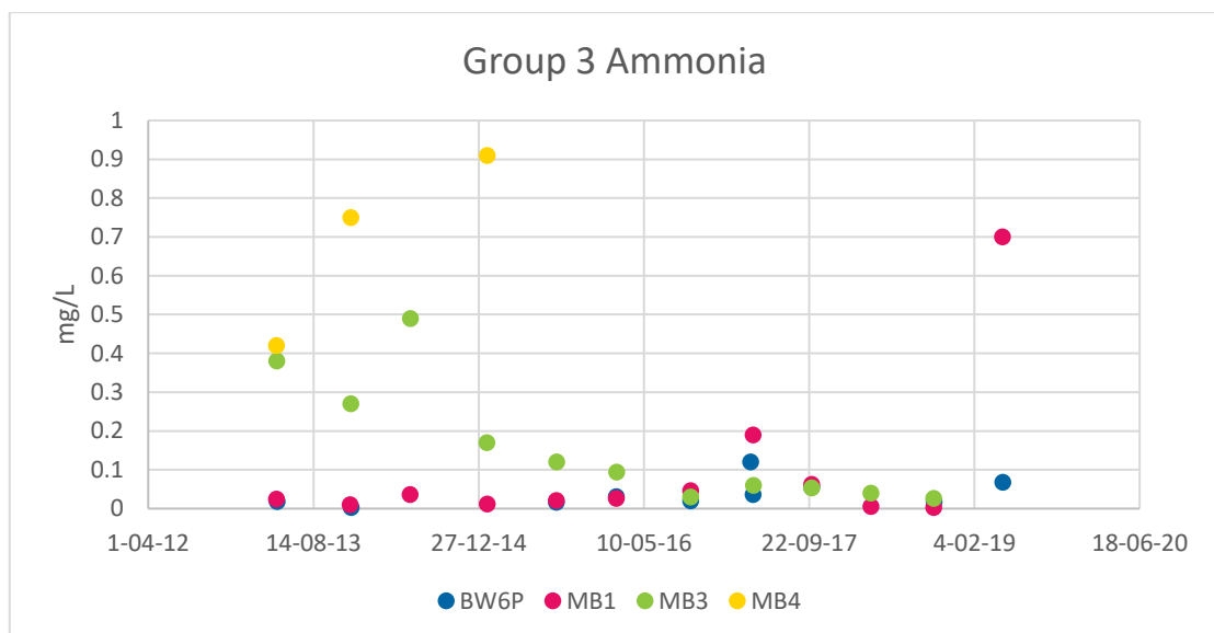
Figure 10-4 Group 3 Ammonia
