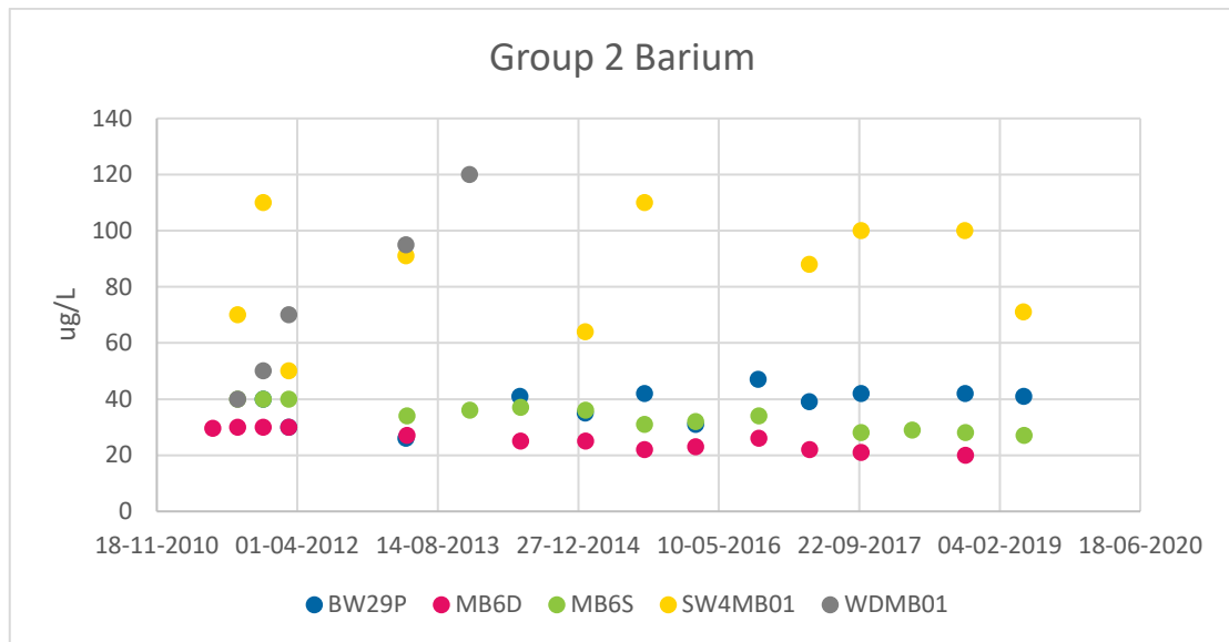
Figure 10-3 Group 2 Barium
