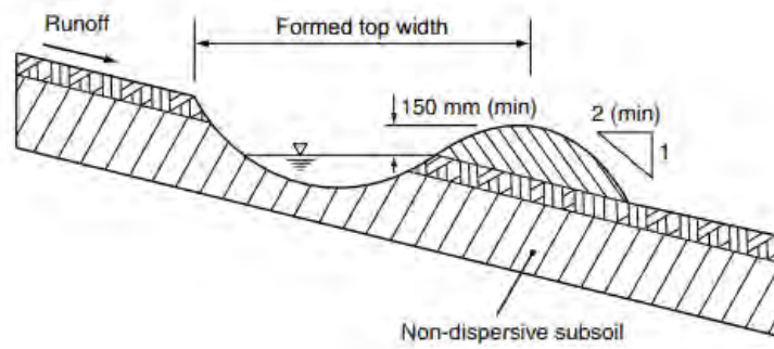
Figure 4-19 Typical catch drain, from Standard Drawing CD-01 (IECA 2008)
