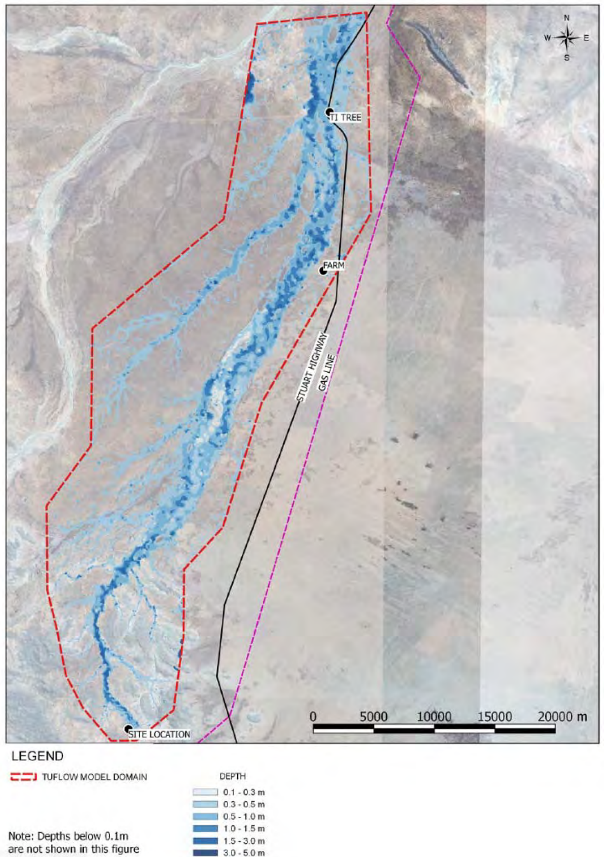
Figure 4-25 TSF flood failure dam break extent (Appendix J)
