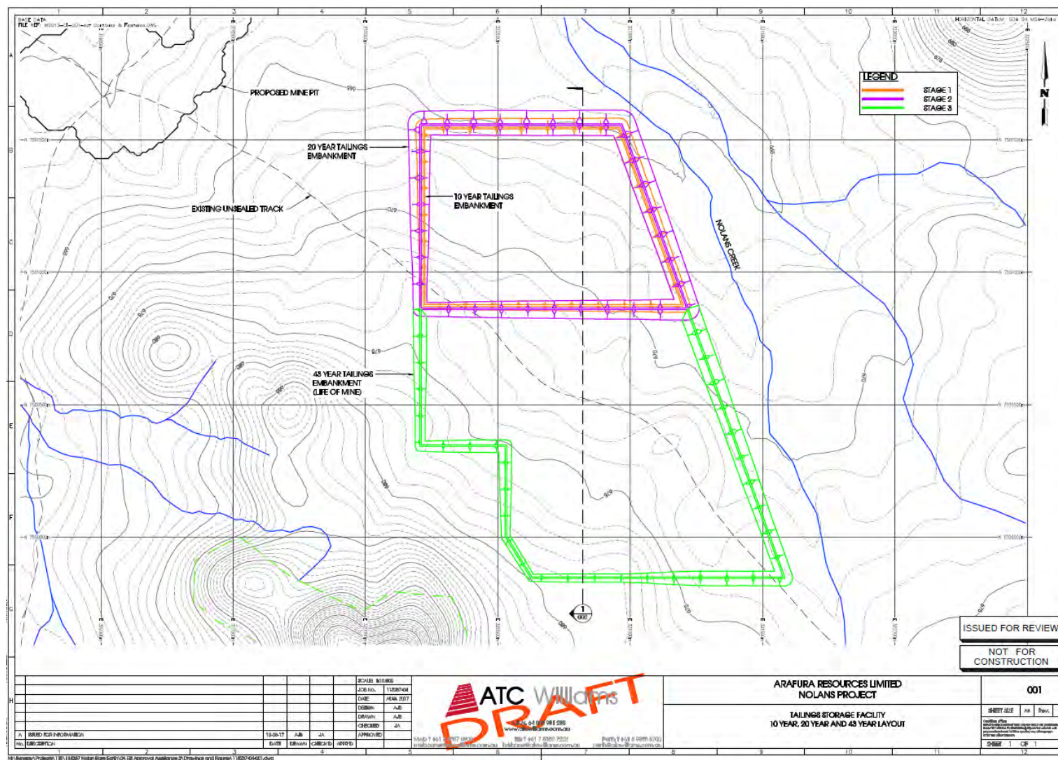
Figure 2-15 TSF layout
