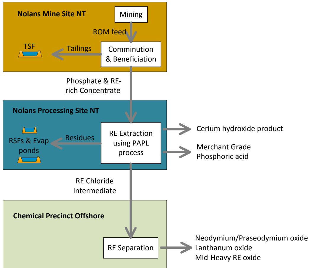
Figure 2-12 Process configuration
