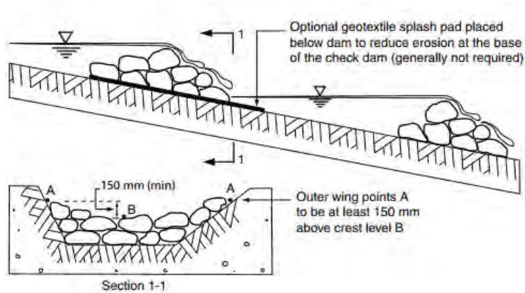
Figure 4-20 Typical check dam, from Standard Drawing RCD-01 (IECA 2008)
