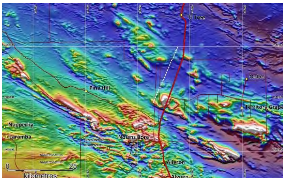
Figure 4-44 Magnetic image showing the location of the Woodforde lineament*
