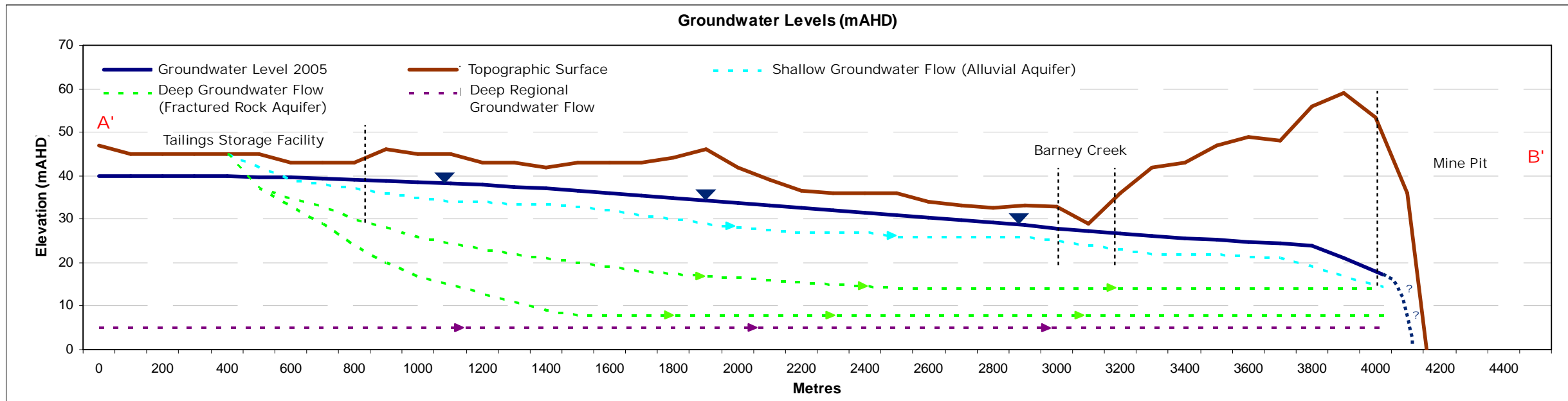
RPS Aquaterra FIGURE 3 Groundwater & Topographic Surface Elevations Along Cross Section From Tailings Storage Facility to Mine Pit
