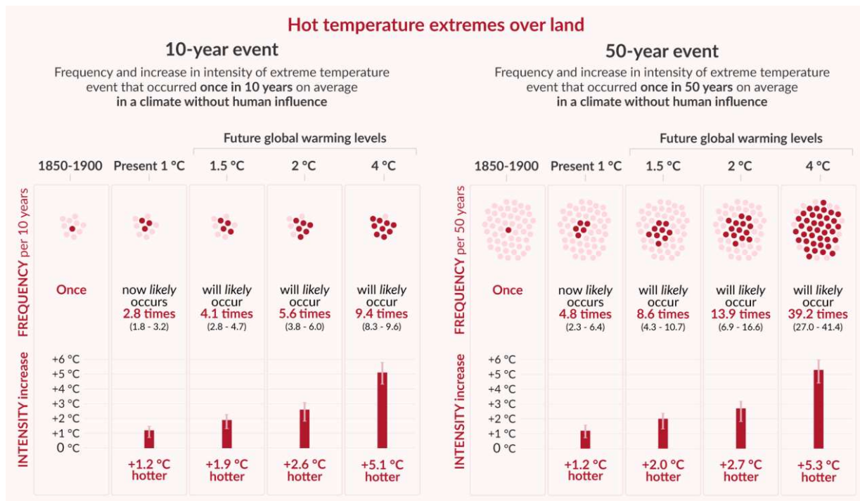
Figure 4 IPCC Sixth Assessment Report – Predicted Changes in Extreme Temperatures and Rainfall
