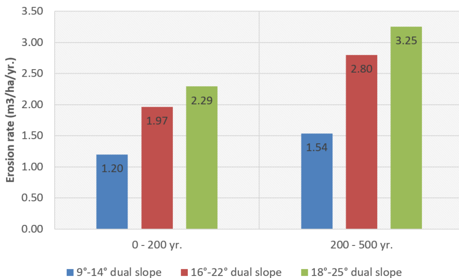
Figure 7 Stage 1 Erosion Rates in the First 500 Years
