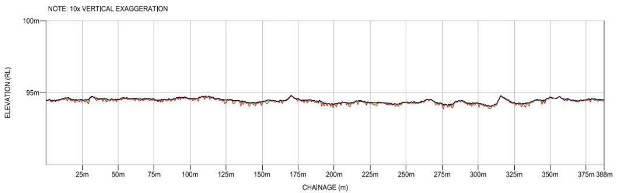
C-C - LONGSECTION
