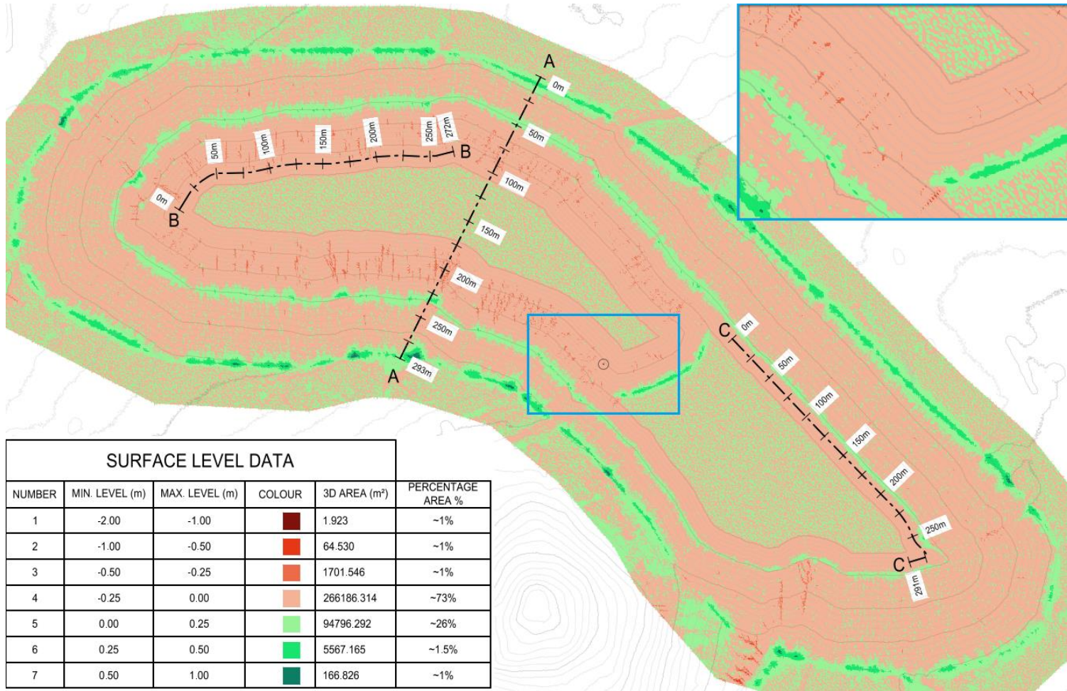
Stage 2, Soil Loss Map, Vegetated 500-year Scenario, EWSF
