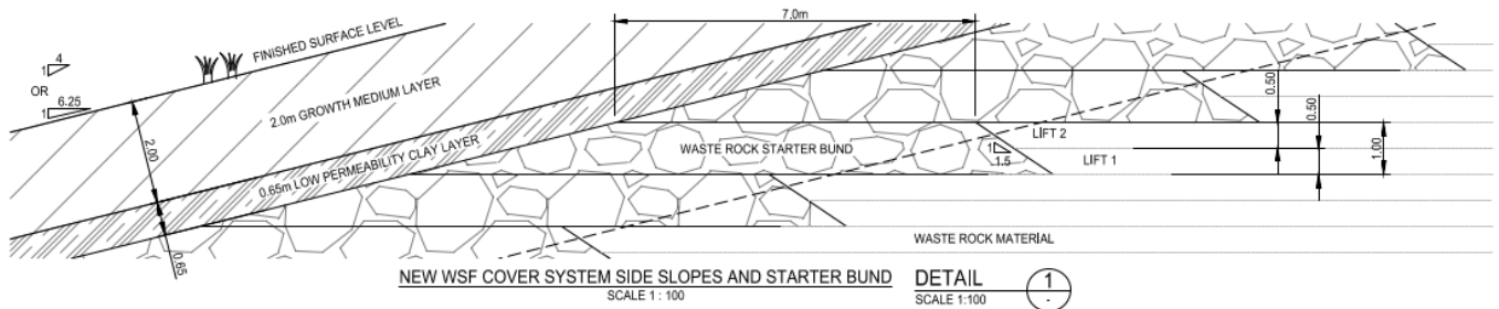
Figure 4 Typical WSF Capping Section, Side Slopes and Starter Bund - Detail 1.
