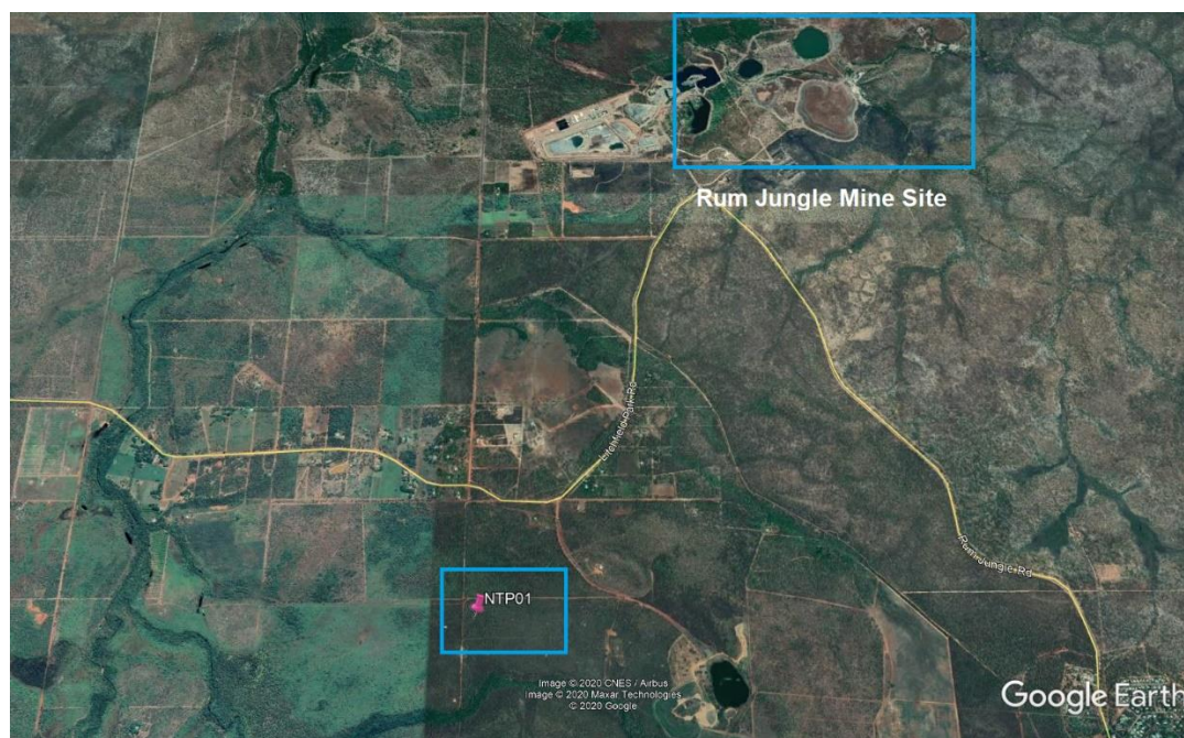
Figure 6 Location of Test Pit NTP01 Where Laterite and Saprolite Materials Were Sampled
