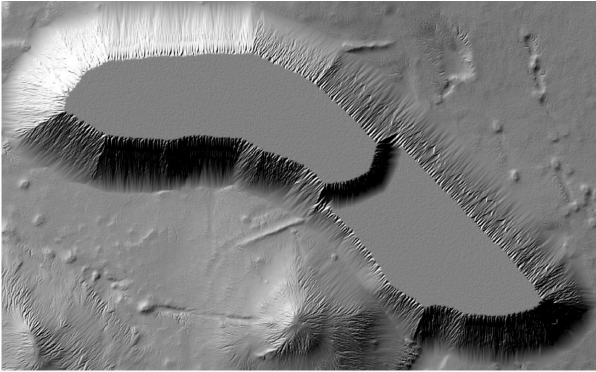
Stage 1, EWSF Hillshade After 500 Years, 16°-22° Dual-slope
