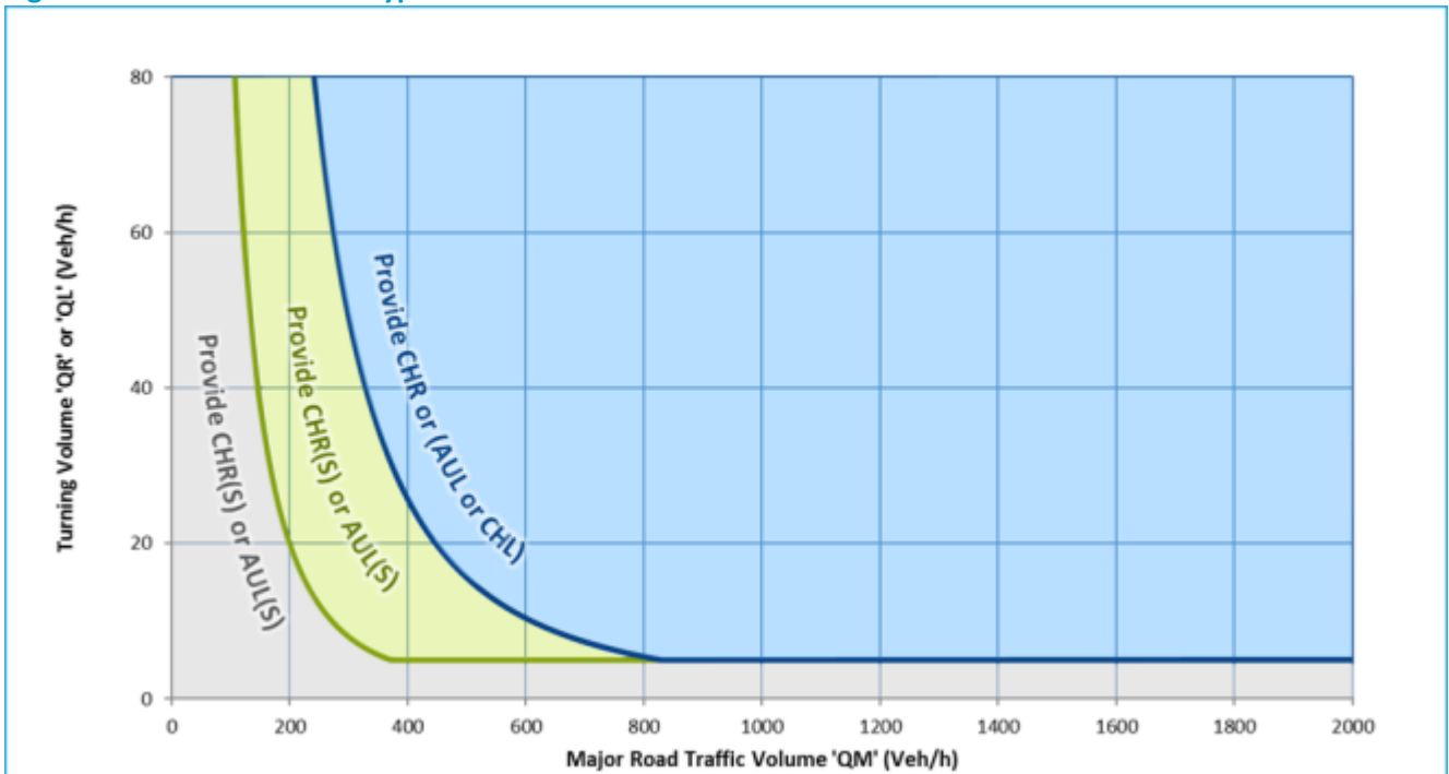
Figure C1 Turn Treatment Types
