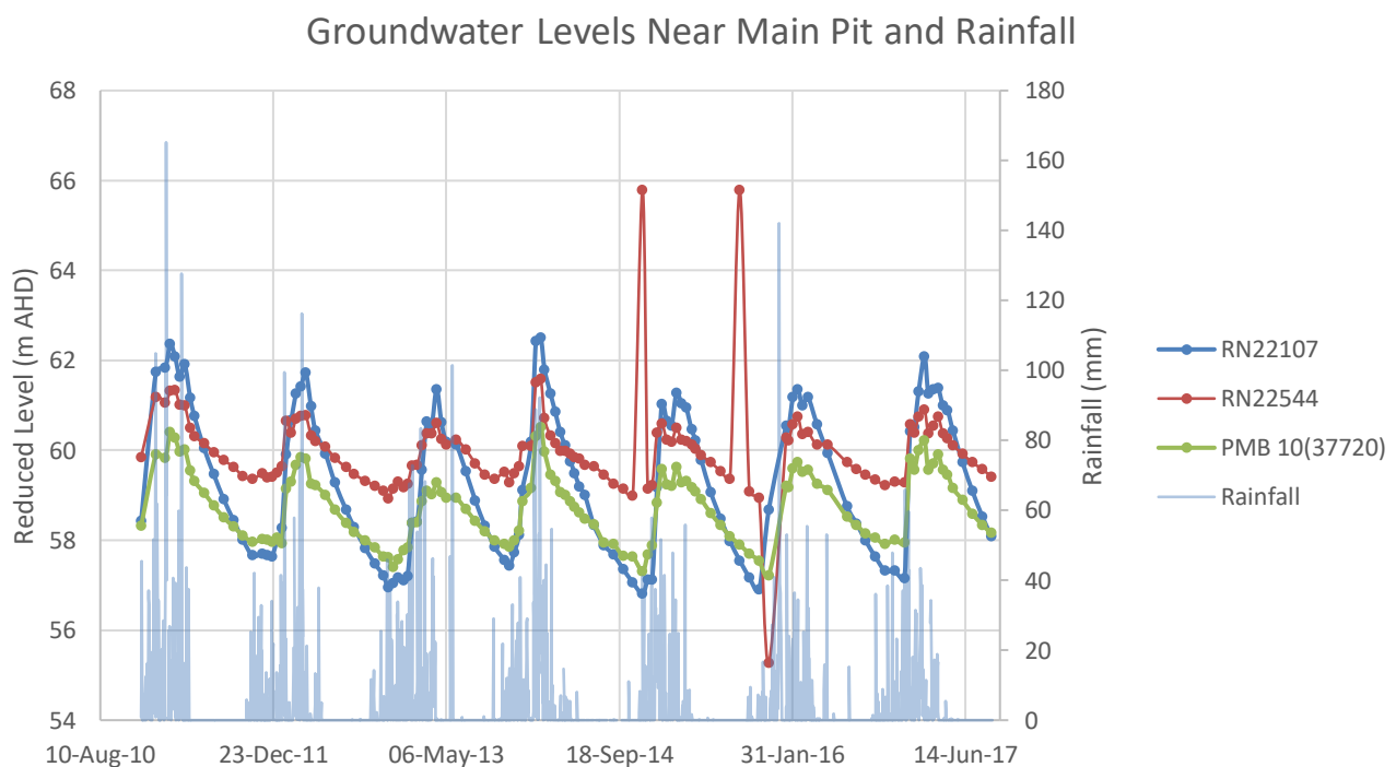
Figure 4 Annual Main Pit Surface Water and Groundwater Levels (DPIR Monitoring Data Dec-2010 to Aug-2017)
