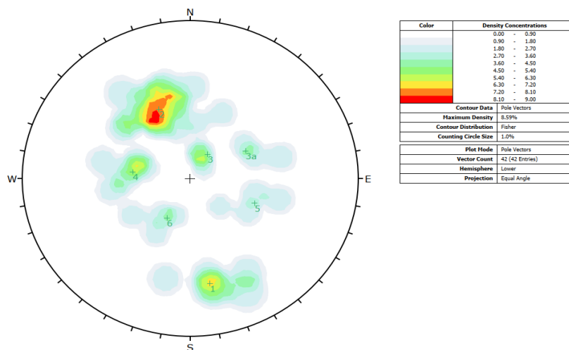
Figure 19 Pole Plot of Orientated Defect Data for Dolostone
