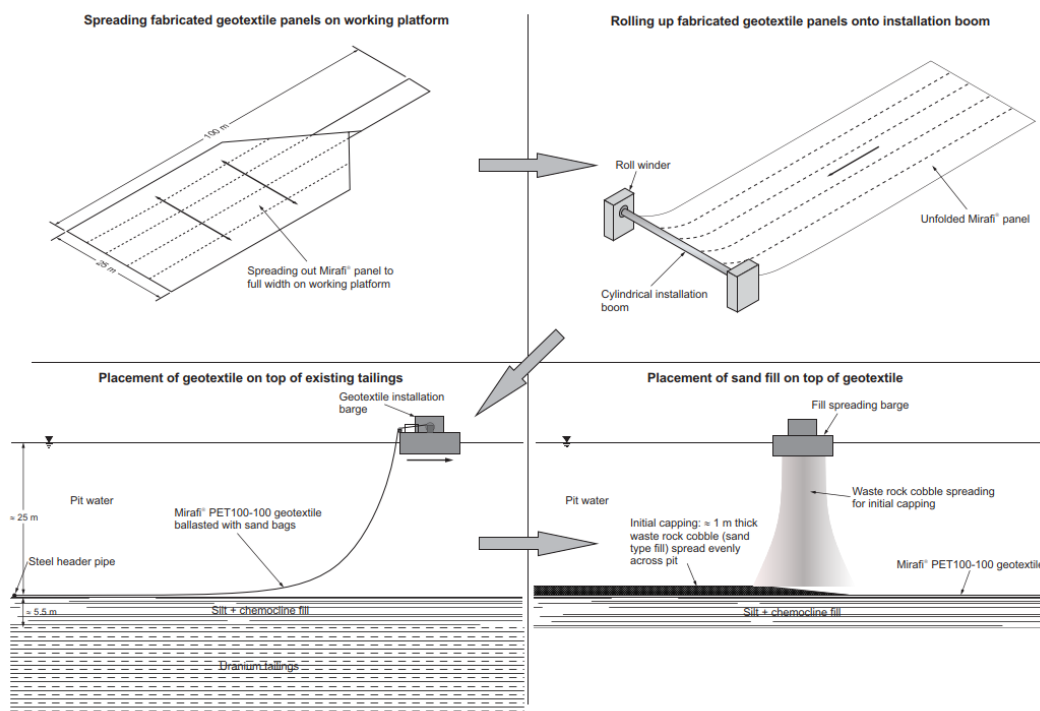
Figure 40 Concept Design of Geotextile Option
