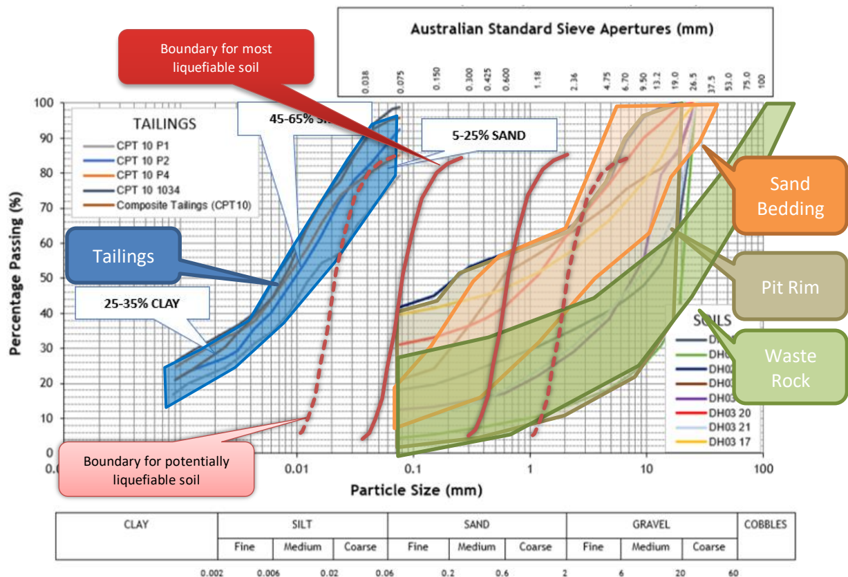
Figure 60 Liquefaction screening based on grading (after Tsuchida 1970 [55])
