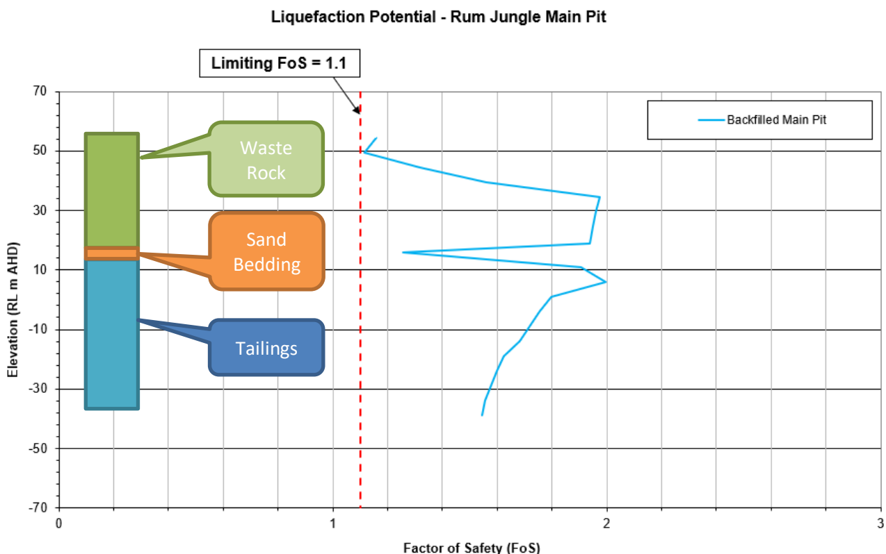
Figure 61 Liquefaction FoS Assessment (after Kramer 1995 [56])
