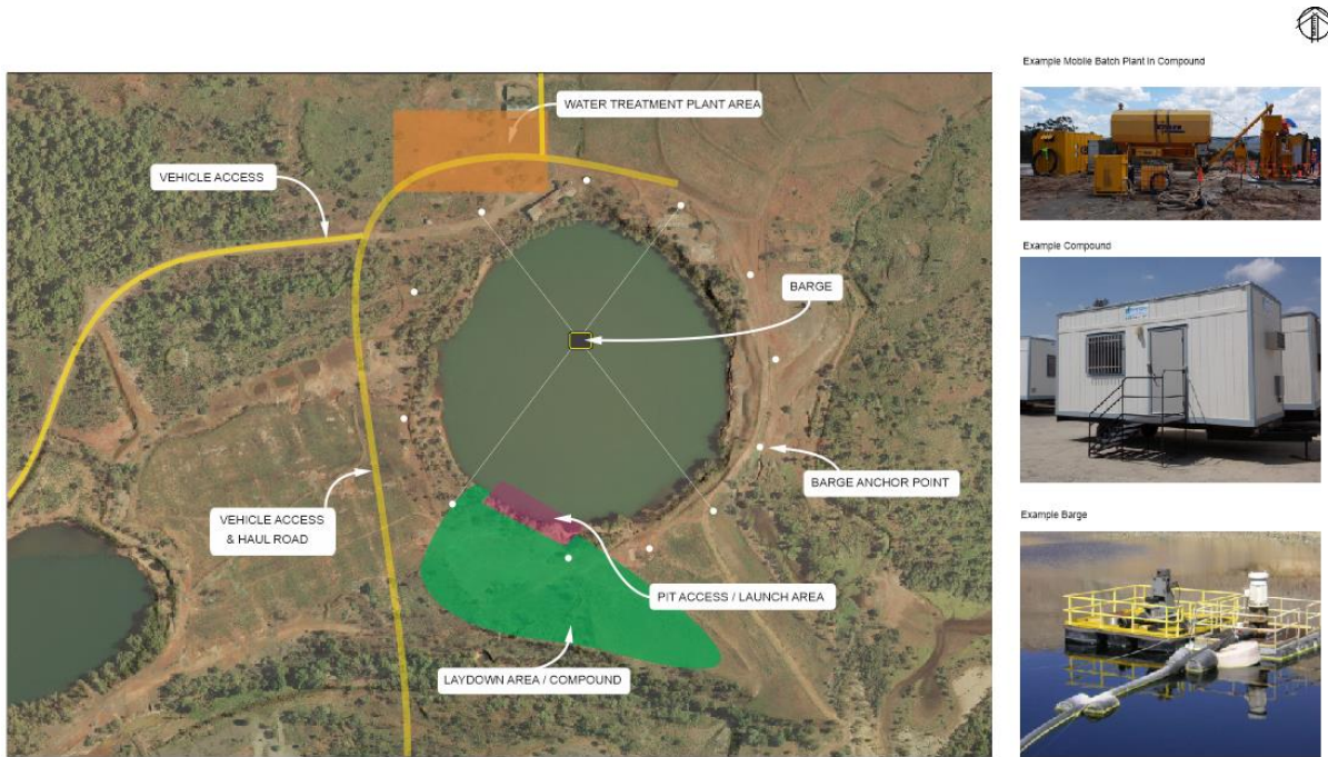
Figure 47 Anticipated Layout of Typical Backfilling Operations
