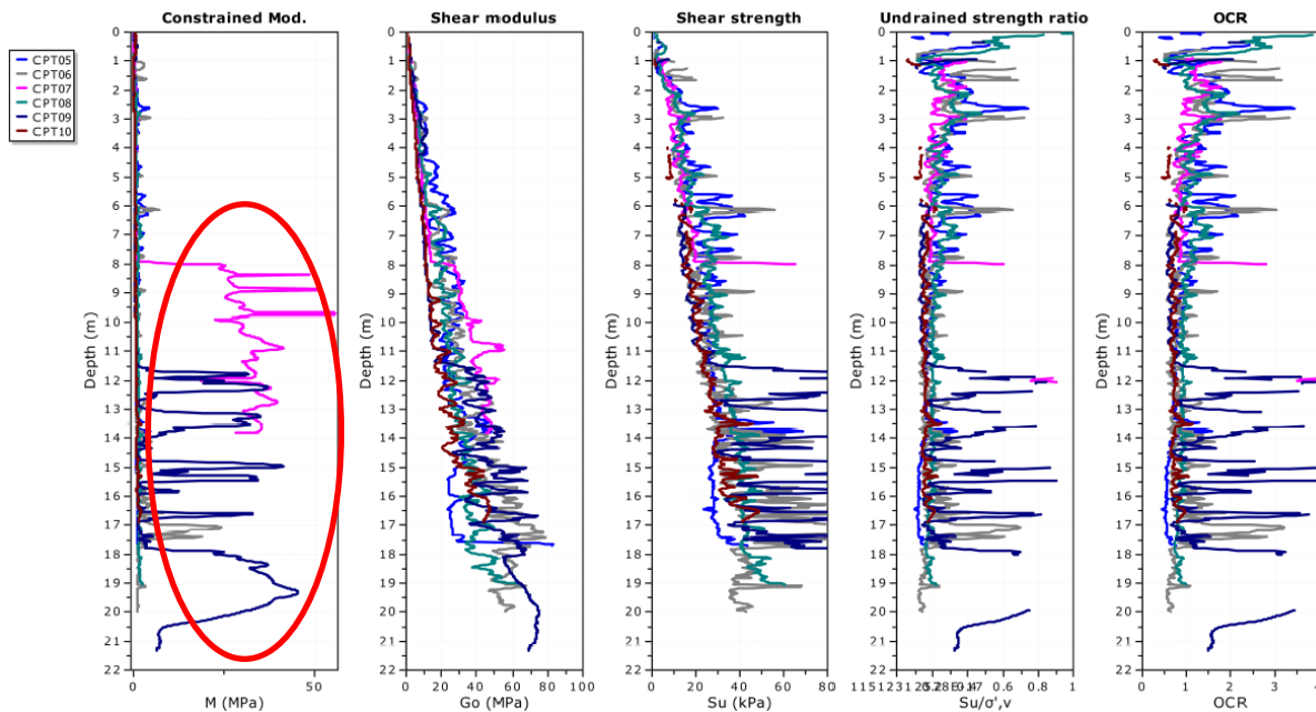
Figure 27 Inferred slopewash soils within tailings (circled)
