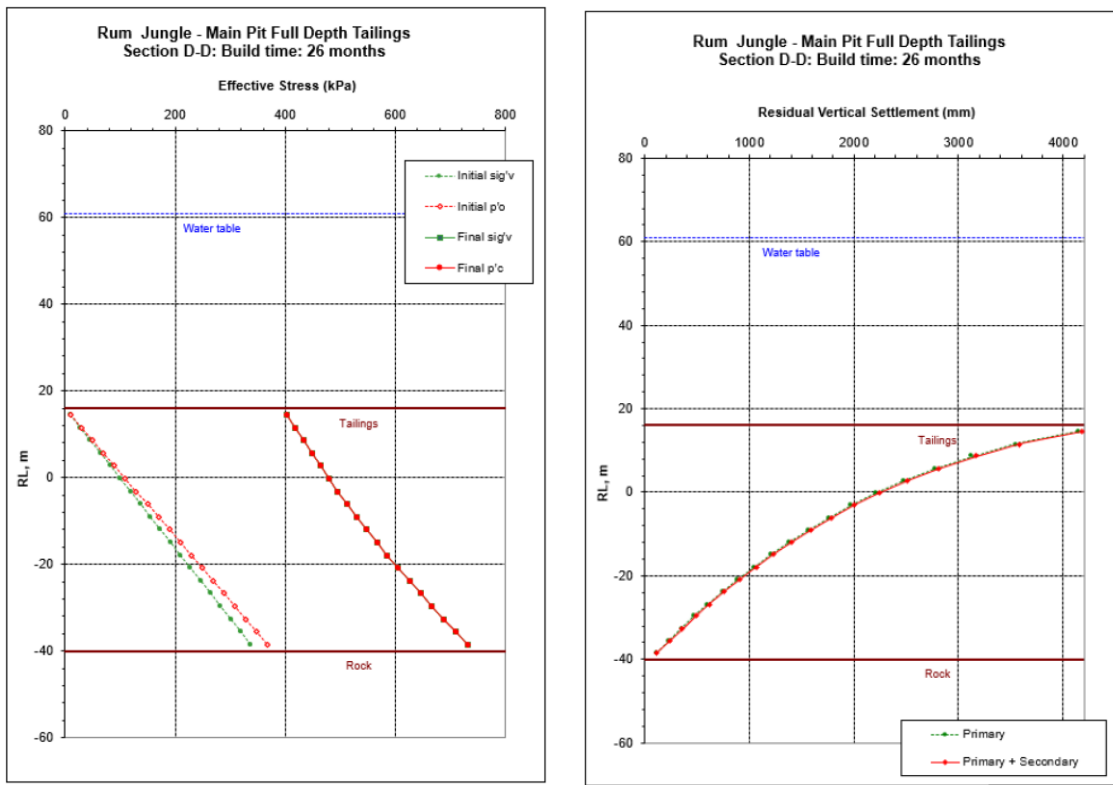
Figure 53 Stress and Settlement in Tailings Layer
