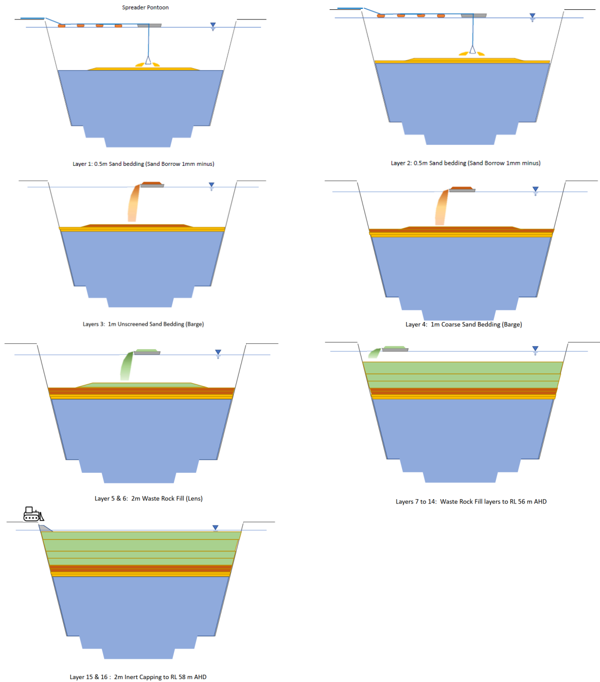
Figure 46 Schematic Backfill Sequence
