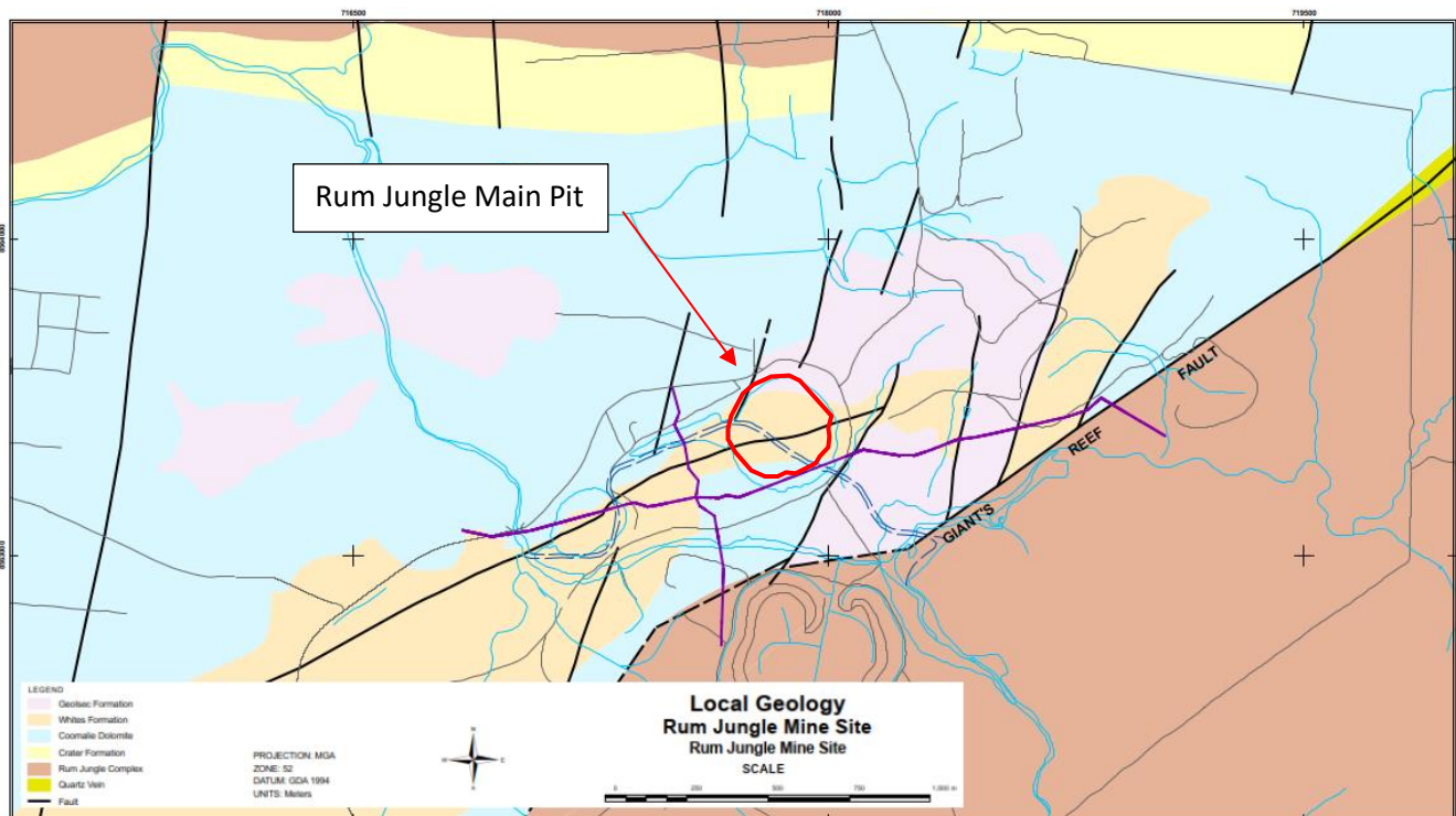
Figure 12 Rum Jungle Geological Setting – Reproduced from Robertson GeoConsultants (2012) [13]
