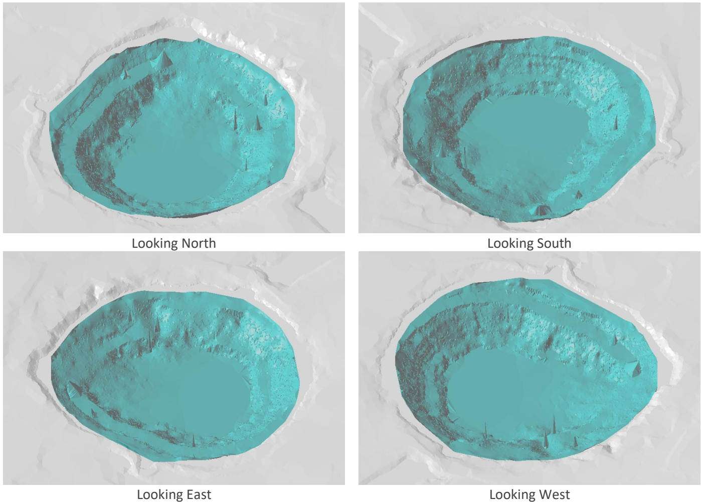
Figure 6 3D Obliques of Main Pit 2015 Surface (2015 Bathymetry Survey)
