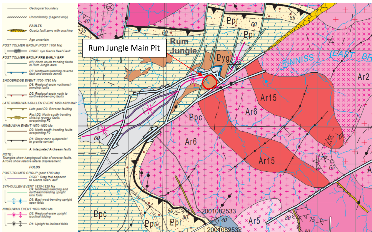
Figure 13 Rum Jungle 1:100:000 Geological Interpretation [30]
