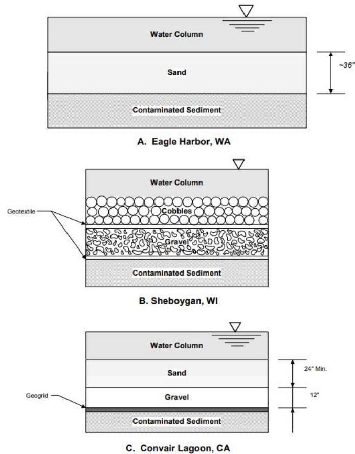
Figure 39 Typical Capping Types (Palermo [44])
