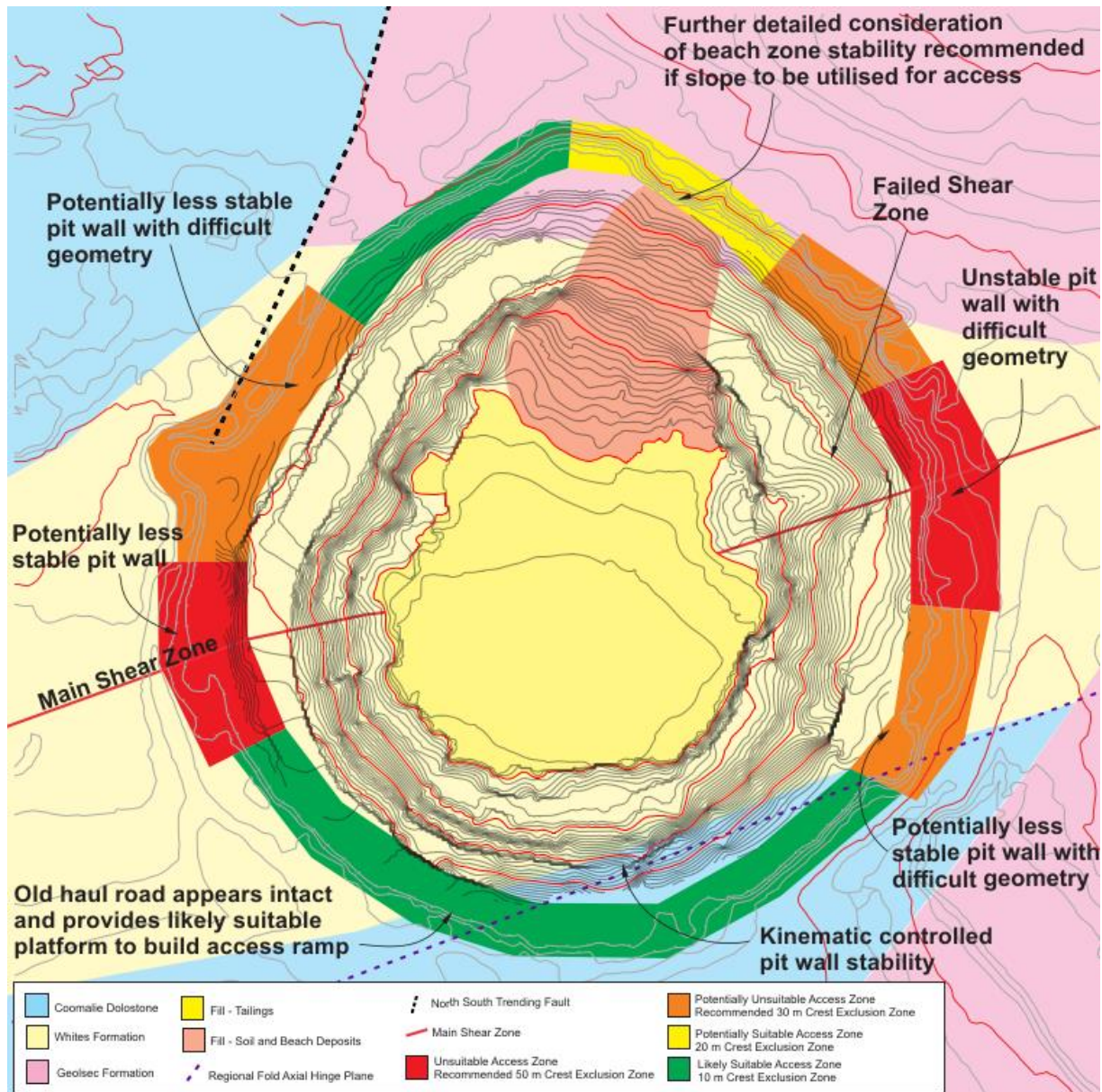
Figure 25 Rum Jungle Main Pit Stability Observations
