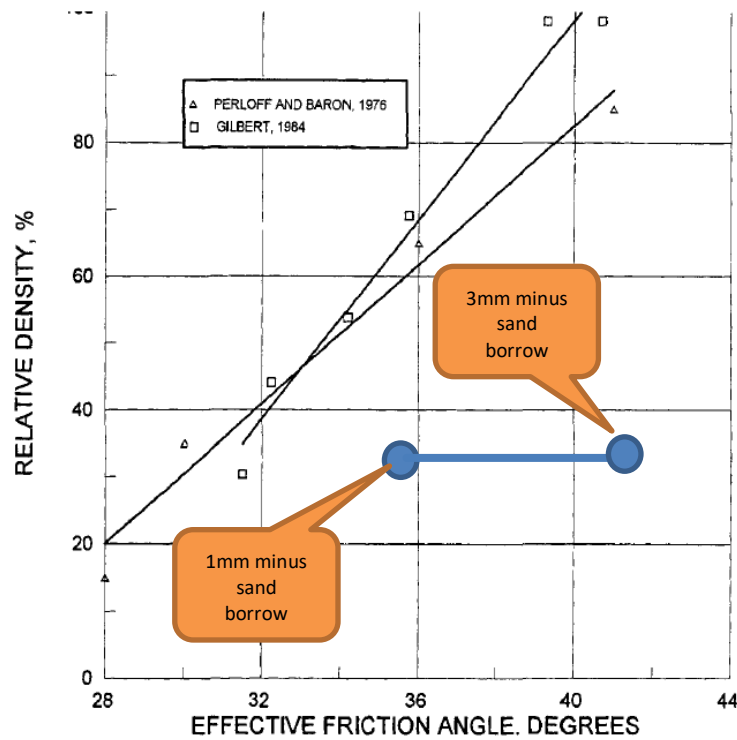
Figure 34 Typical and Measured Friction Angle for Sands
