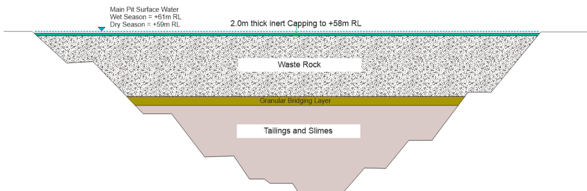
Figure 8 Generalised Main Pit Backfilled Profile
