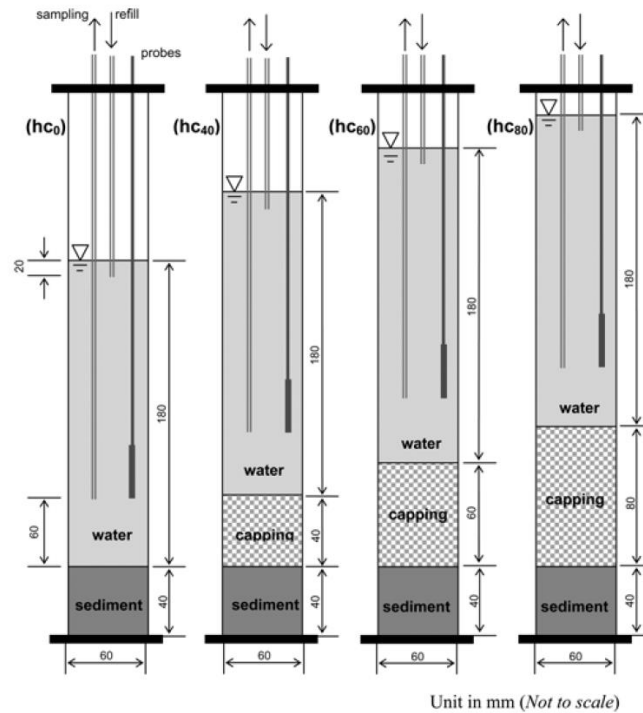
Figure 41 Schematic of bench scale sediment column testing
