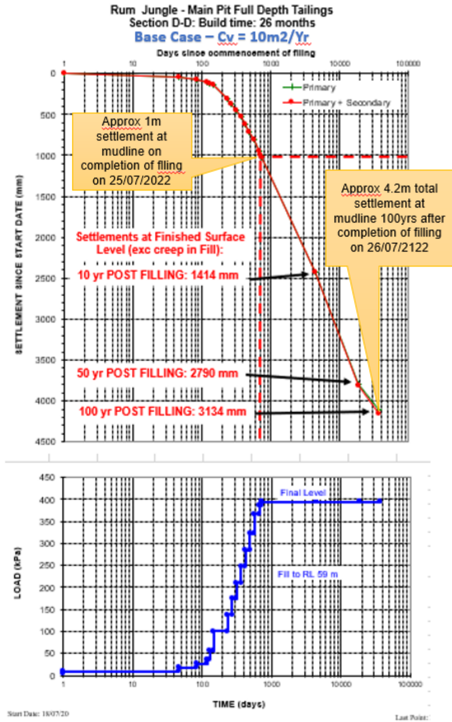
Figure 51 Settlement of Tailings
