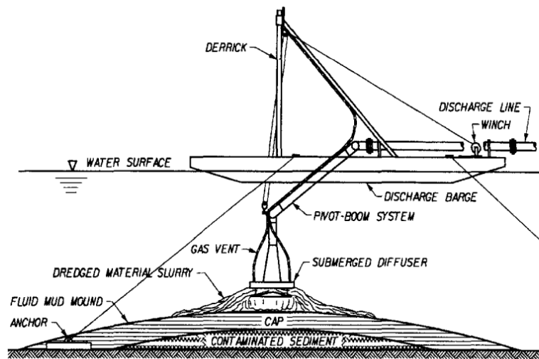
Figure 45 Example of Spreader Pontoon with Diffuser
