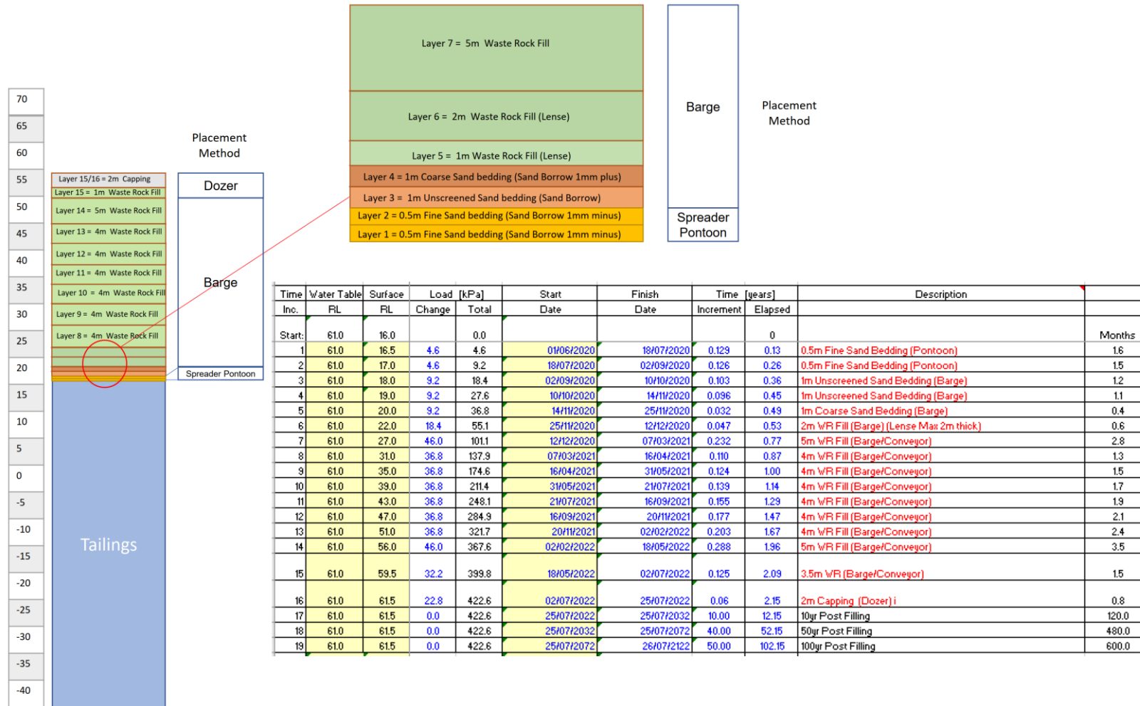
Figure 49 Backfilling Strategy and Indicative Program
