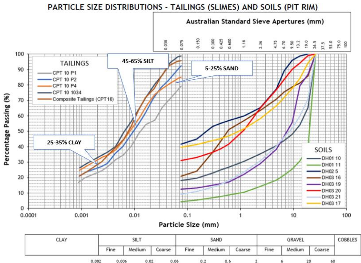
Figure 29 Particle Size Distribution Tailings and Pit Rim Soils
