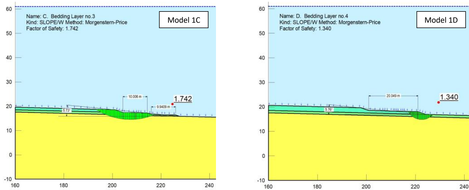
Figure 55 Models 1C and 1D
