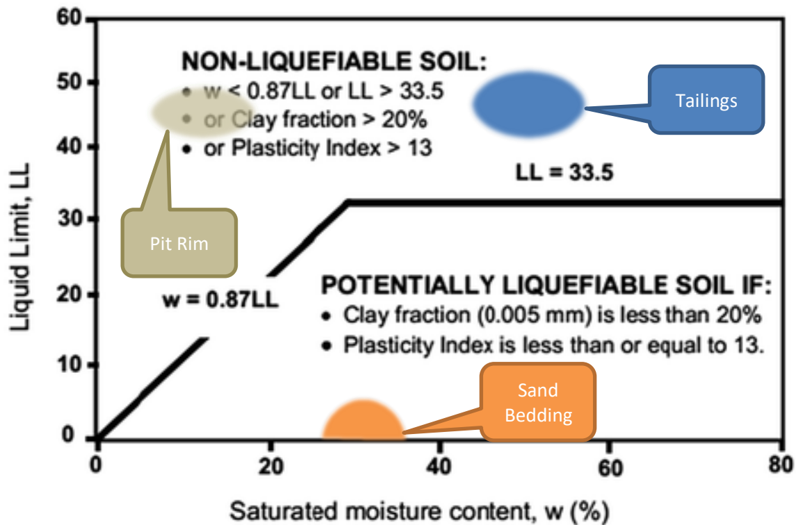
Figure 59 Liquefaction Screening Based on Material Classification
