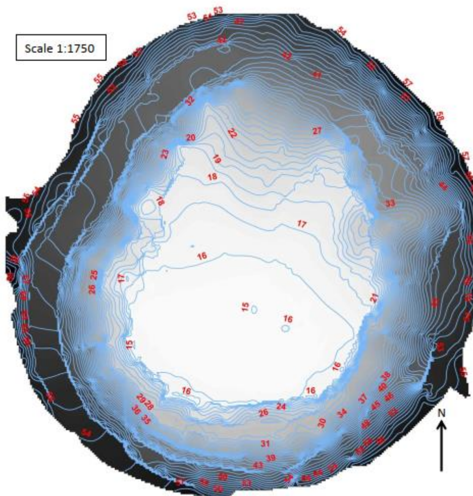
Figure 5 2015 Main Pit Bathymetric Survey (Miloshis and Fairfield [16])
