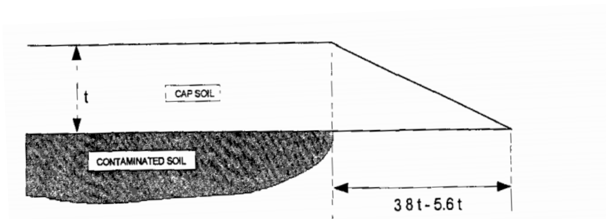
Figure 42 Typical Limiting Fill Slope for Stability
