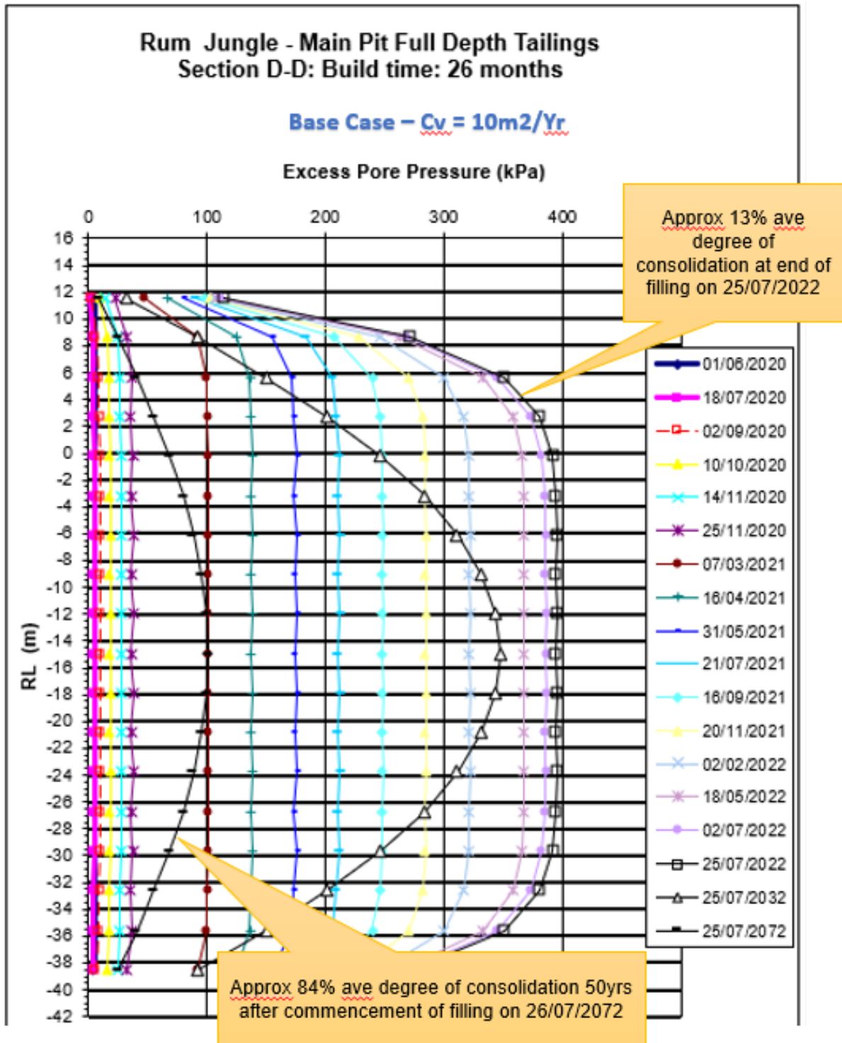
Figure 52 Excess Pore Pressure in Tailings
