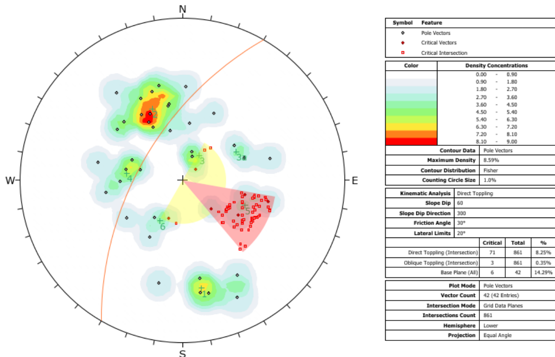
Figure 23 Direct Toppling Failure Analysis for South East Quadrant Slope
