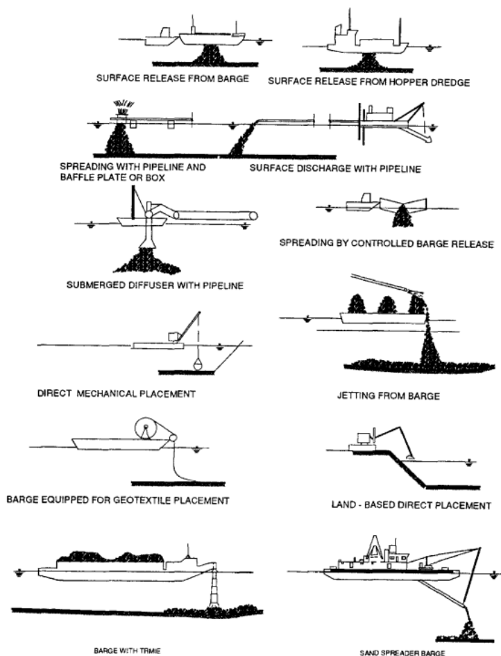
Figure 44 Examples of Typical Capping Layer Placement Methods (Image: US EPA [46])
