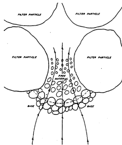
Figure 43 Granular Filter at Capping/Tailings Interface (Image: USACE [53])
