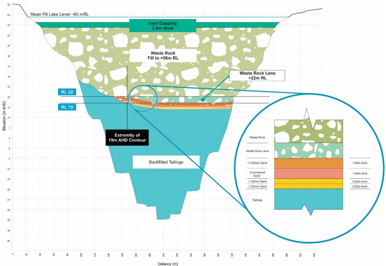
Figure 48 Proposed Layering of Fill Materials
