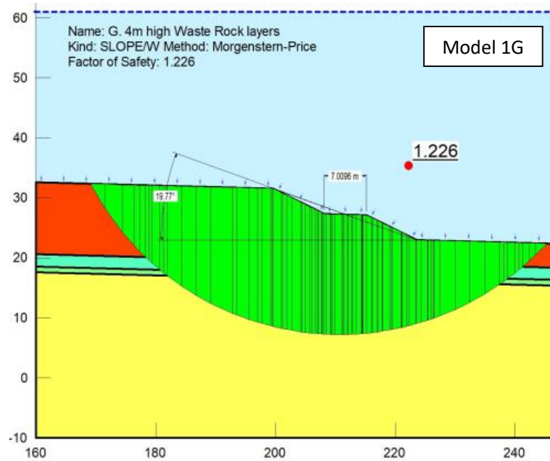
Figure 57 Models 1G and 1H without geotextile
