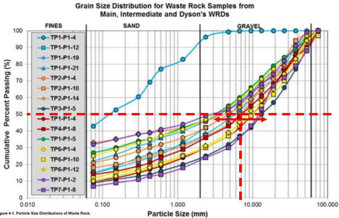
Figure 4-1. Particle Size Distributions of Waste Rock.
