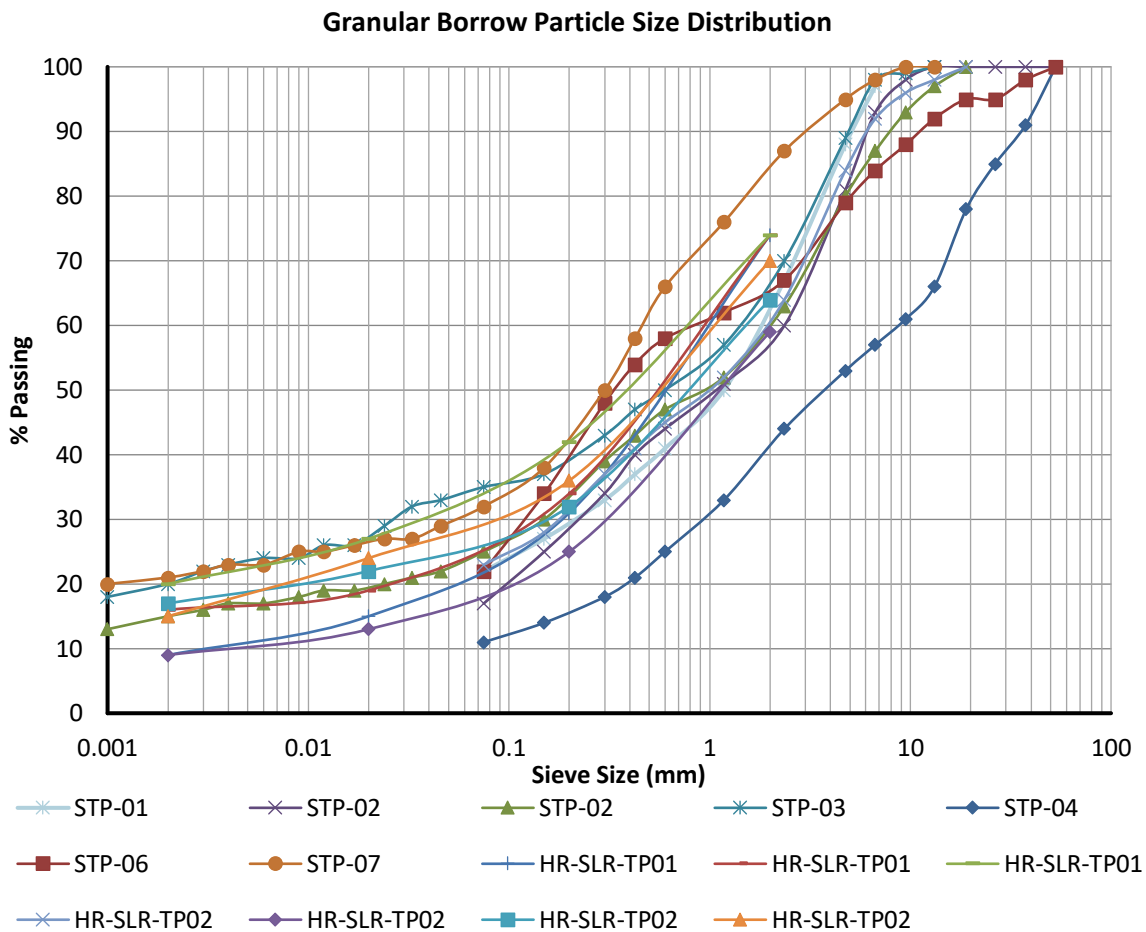
Figure 10 Compiled PSD Curves - Granular and Growth Borrow (Borrow Area B)
