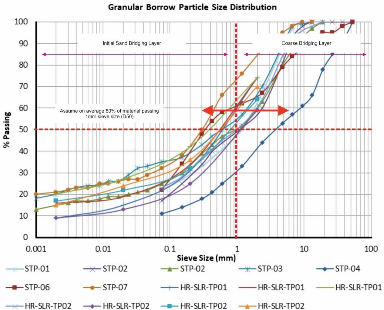
Figure 33 Sand Bedding Layer Grading Summary
