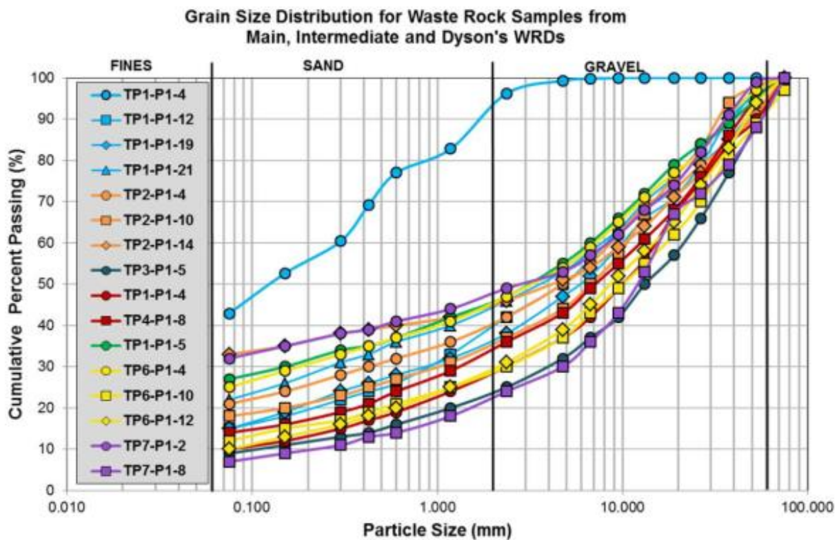
Figure 11 Waste Rock PSD Curves for Material <75mm (From RGC [18])
