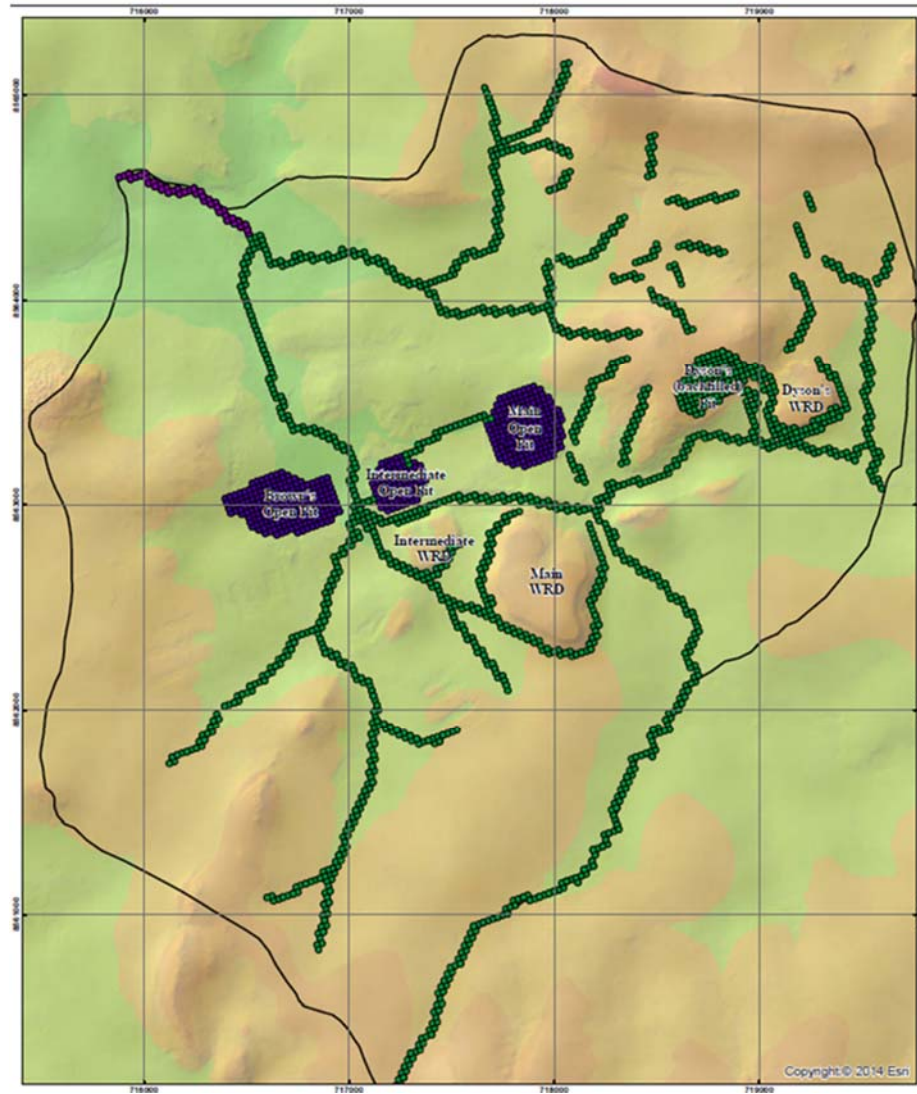
Figure E-2. Model Domain and Boundary Conditions
