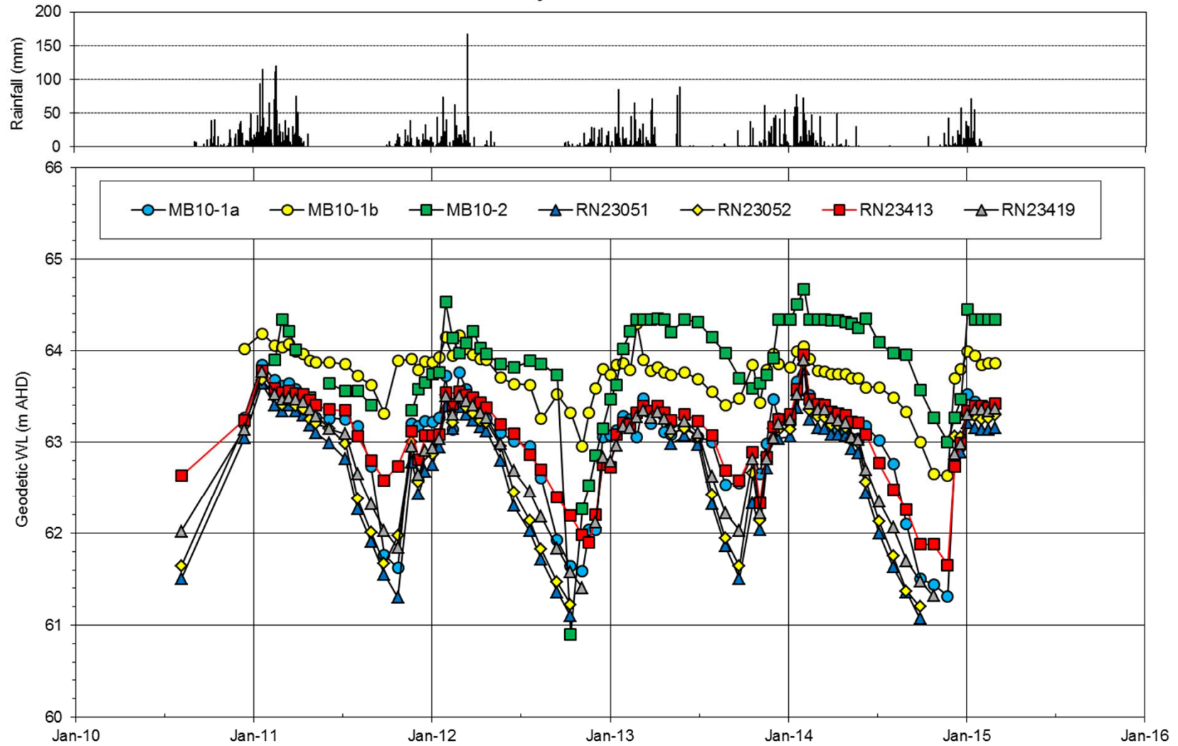
Groundwater Levels in Dyson's Area 2010 - 2015
