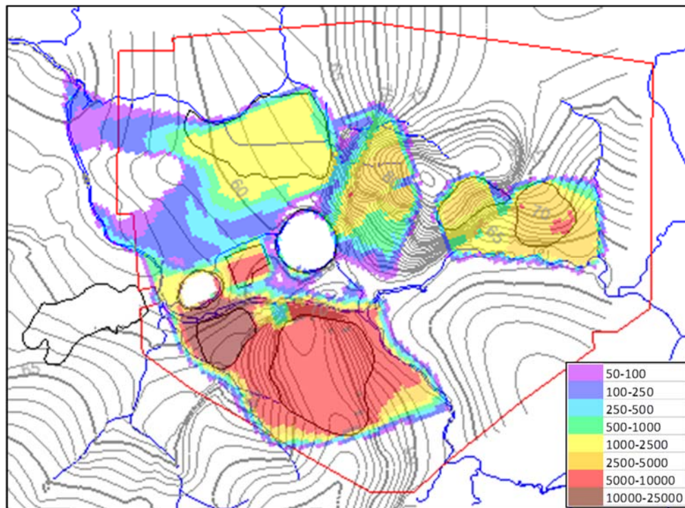
Figure E-4. Simulated 'Historic' SO 4 Concentrations (in mg/L) in Groundwater for Layer 3 (Before Initial Rehabilitation).
