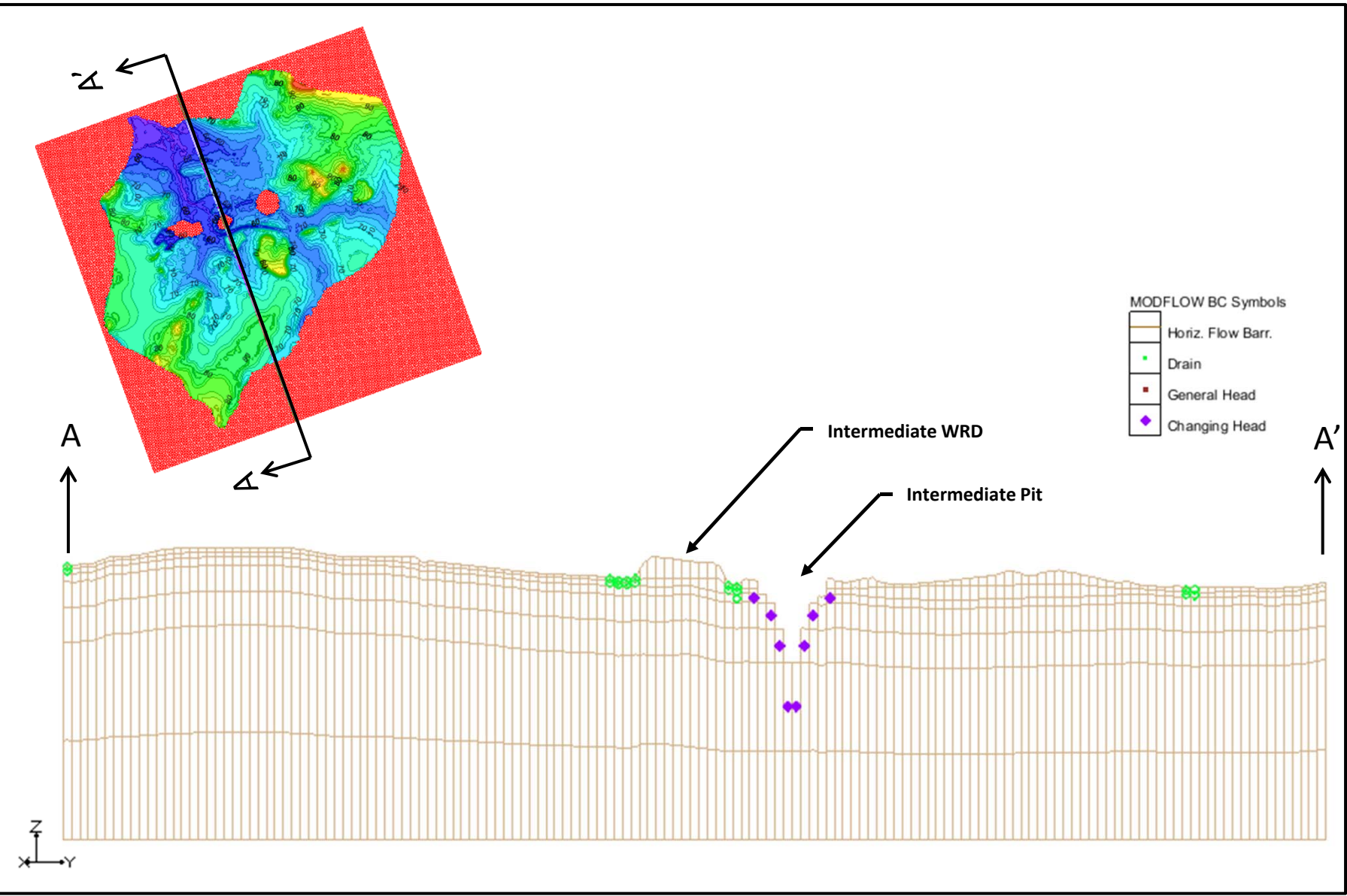
Model Cross-Section S-N Through Intermediate Pit and WRD (Column 87)
