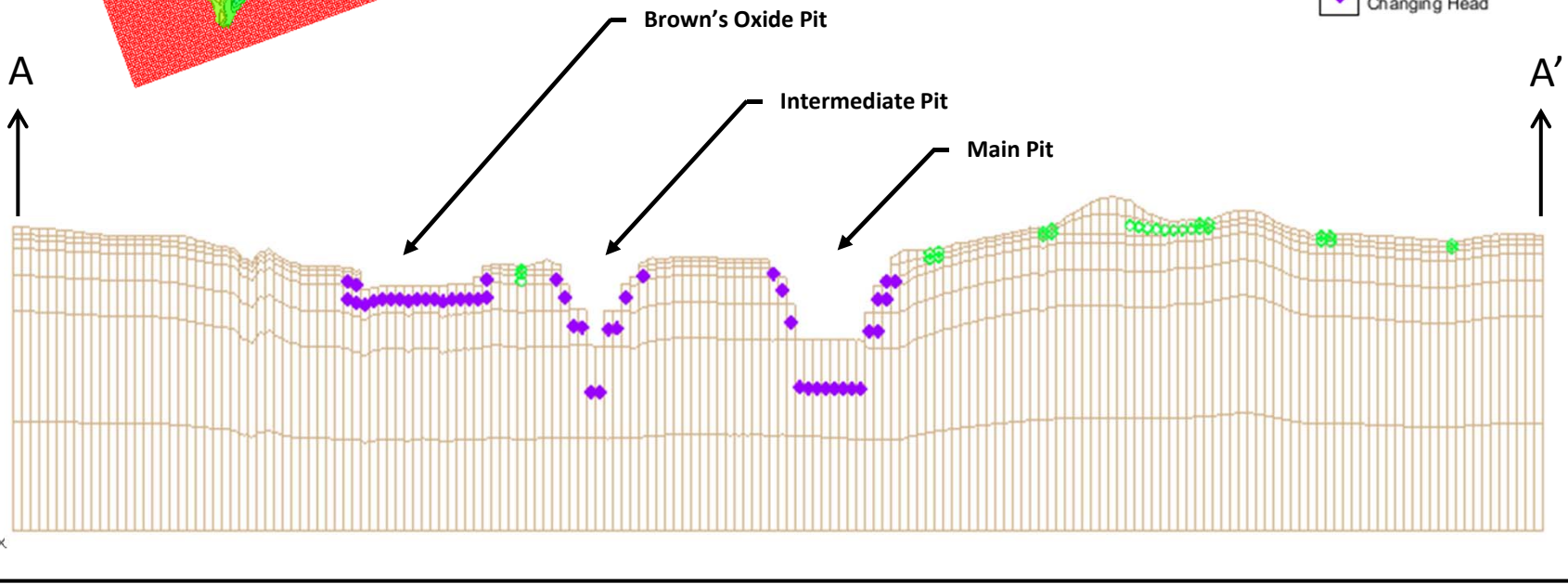
Model E-W Cross-Section Through Central Mining Area (Row 78)
