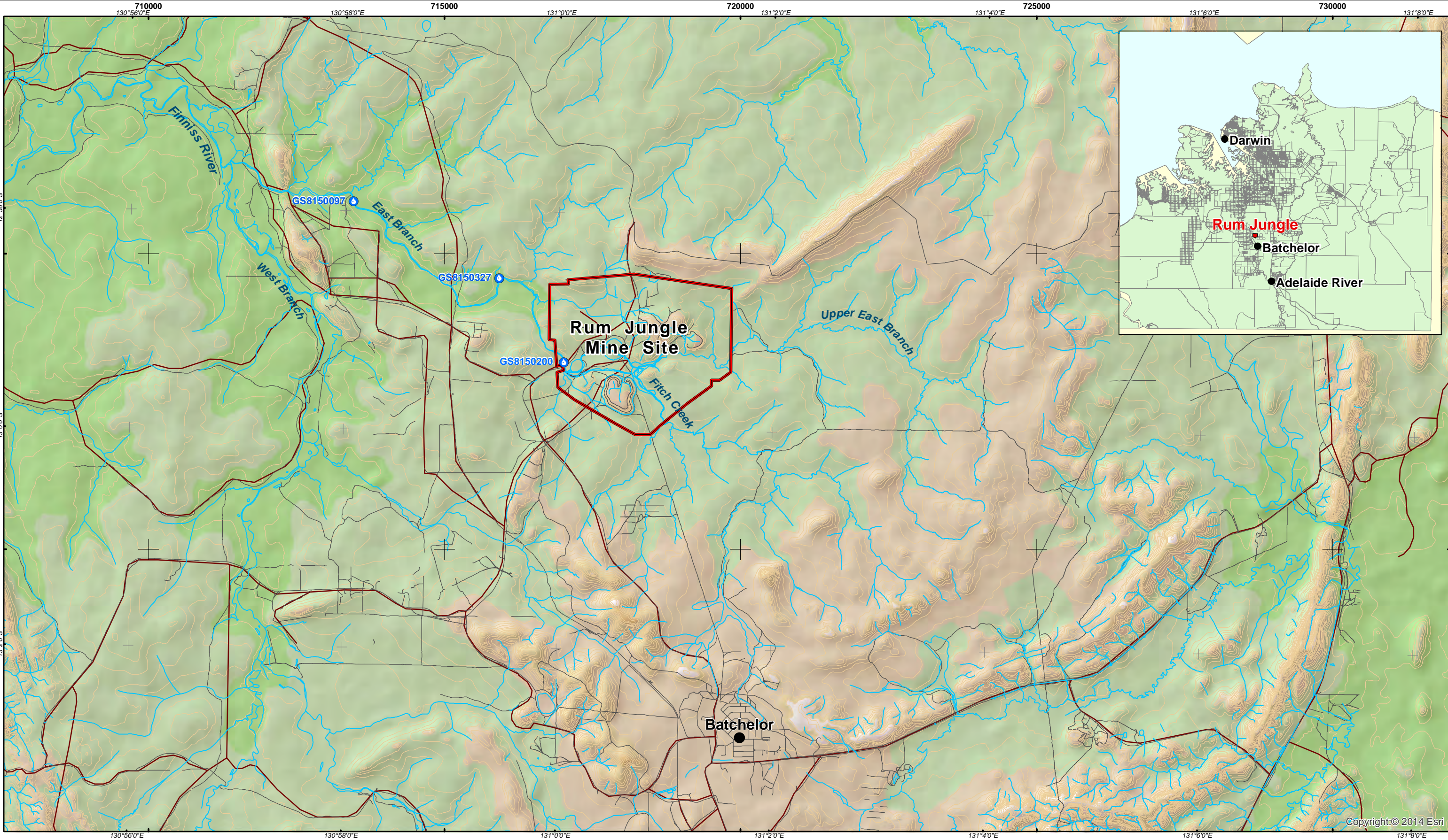
Location, Regional Topography and Drainage near Rum Jungle Mine Site
