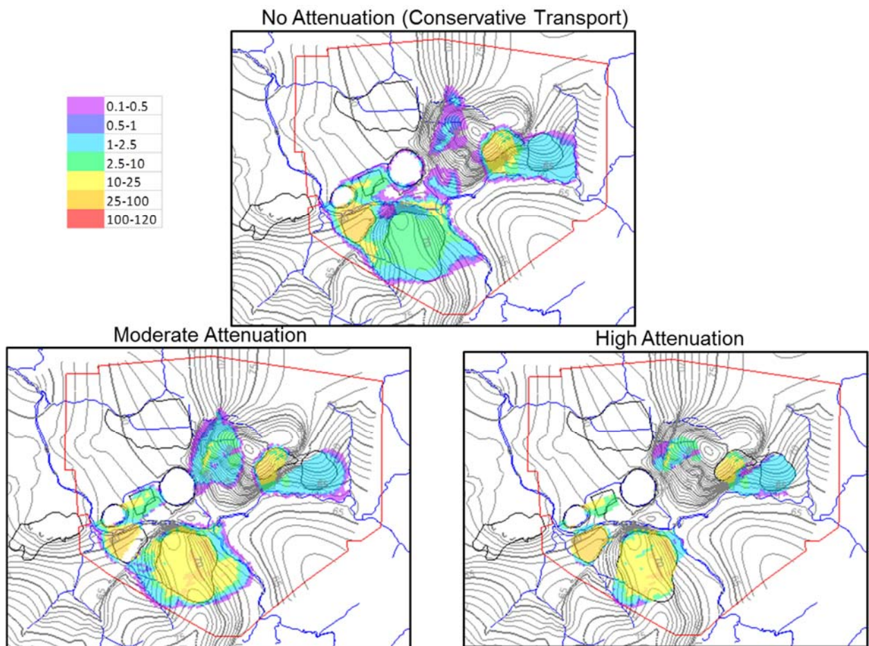
Figure E-6. Simulated 'Current' Cu Concentrations (in mg/L) in Groundwater for Layer 3 (Current Conditions).
