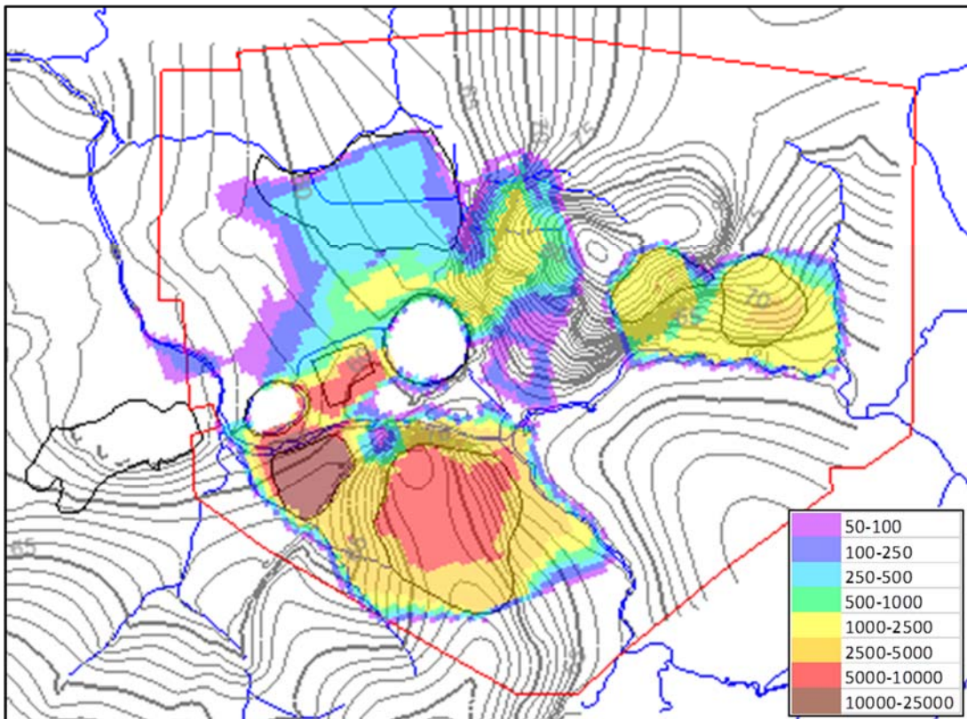
Figure E-5. Simulated 'Current' SO 4 Concentrations (in mg/L) in Groundwater for Layer 3 (Current Conditions).
