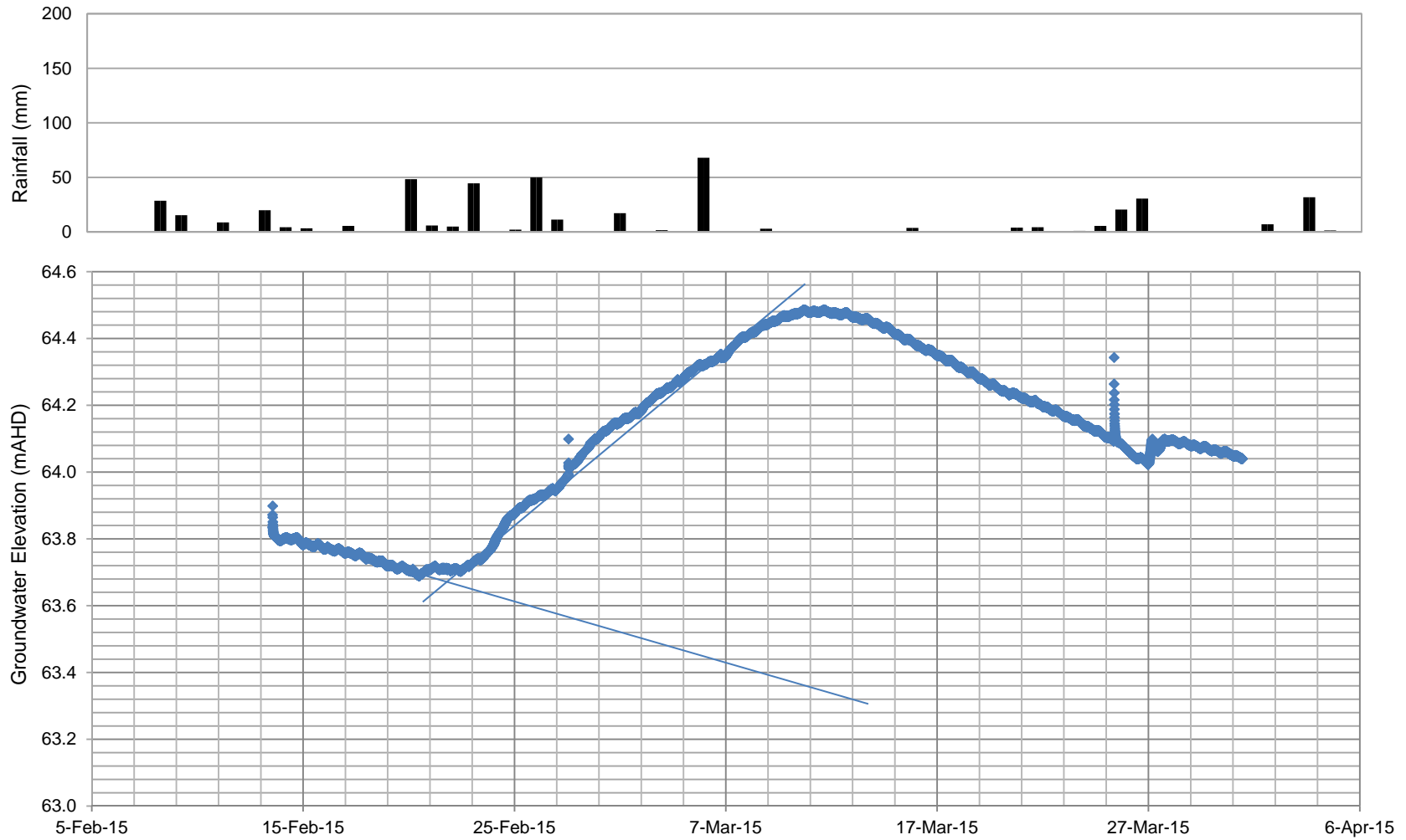
Response to Precipitation at Monitoring Bore MB14-20S
