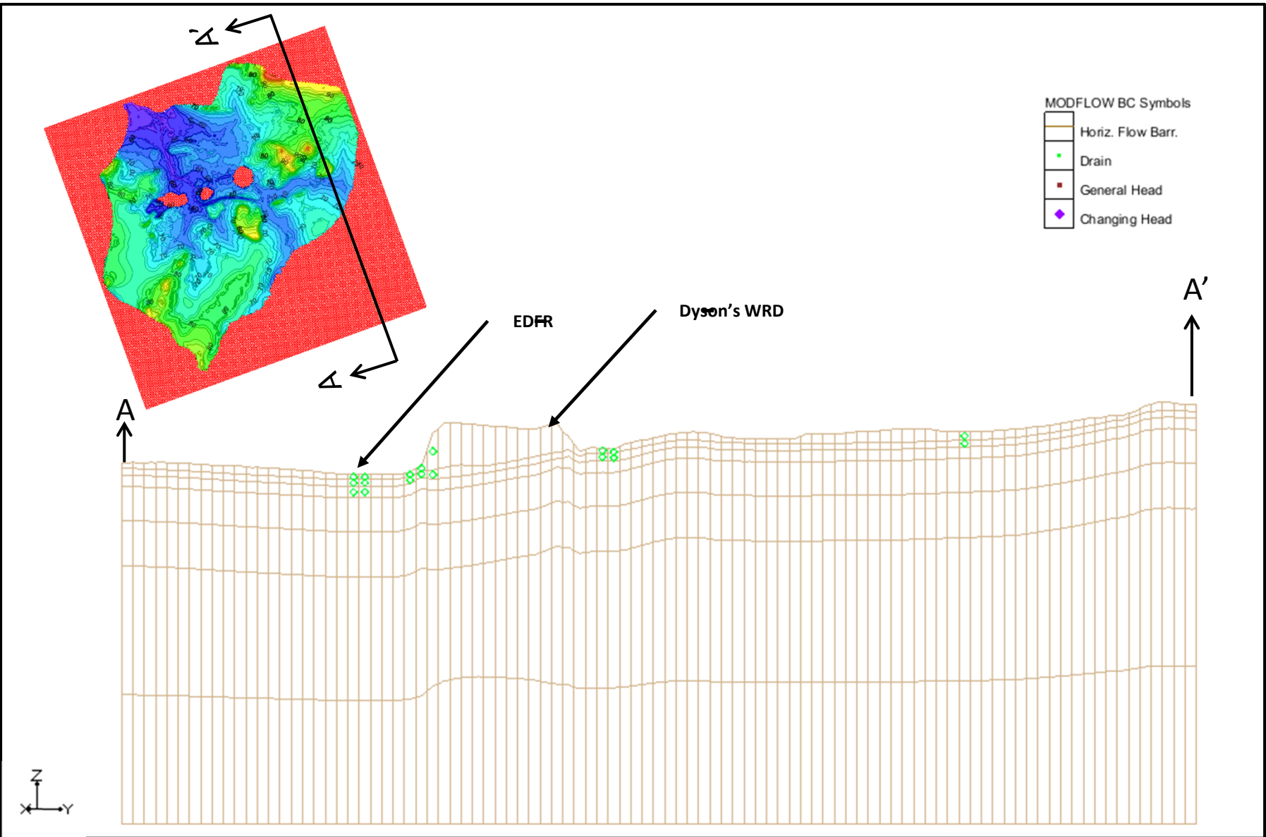
Model Cross-Section N-S Through Dyson's WRD (Column 169)
