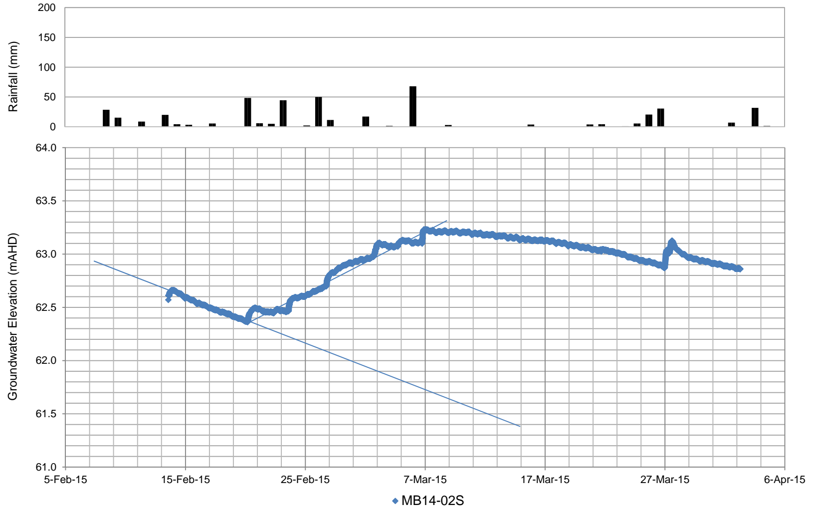
Response to Precipitation at Monitoring Bore MB14-02S
