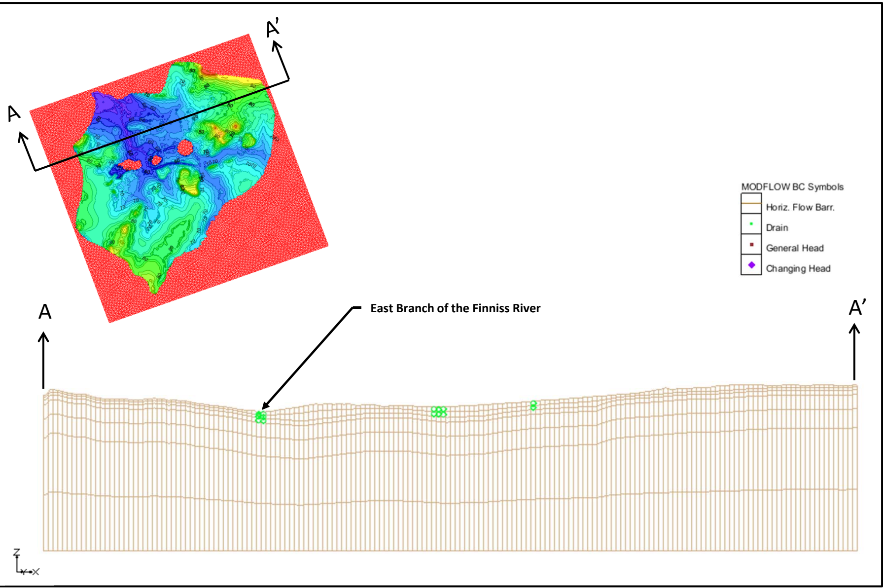
Model Cross-Section W-E Through Old Tailings Dam Area (Row 51)
