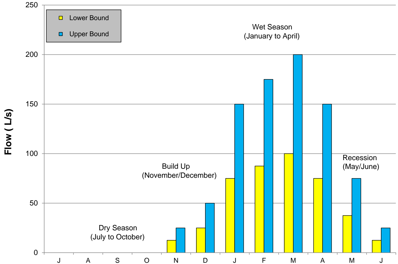
Potential Groundwater Flows to EBFR Downstream of Gauge GS8150200
