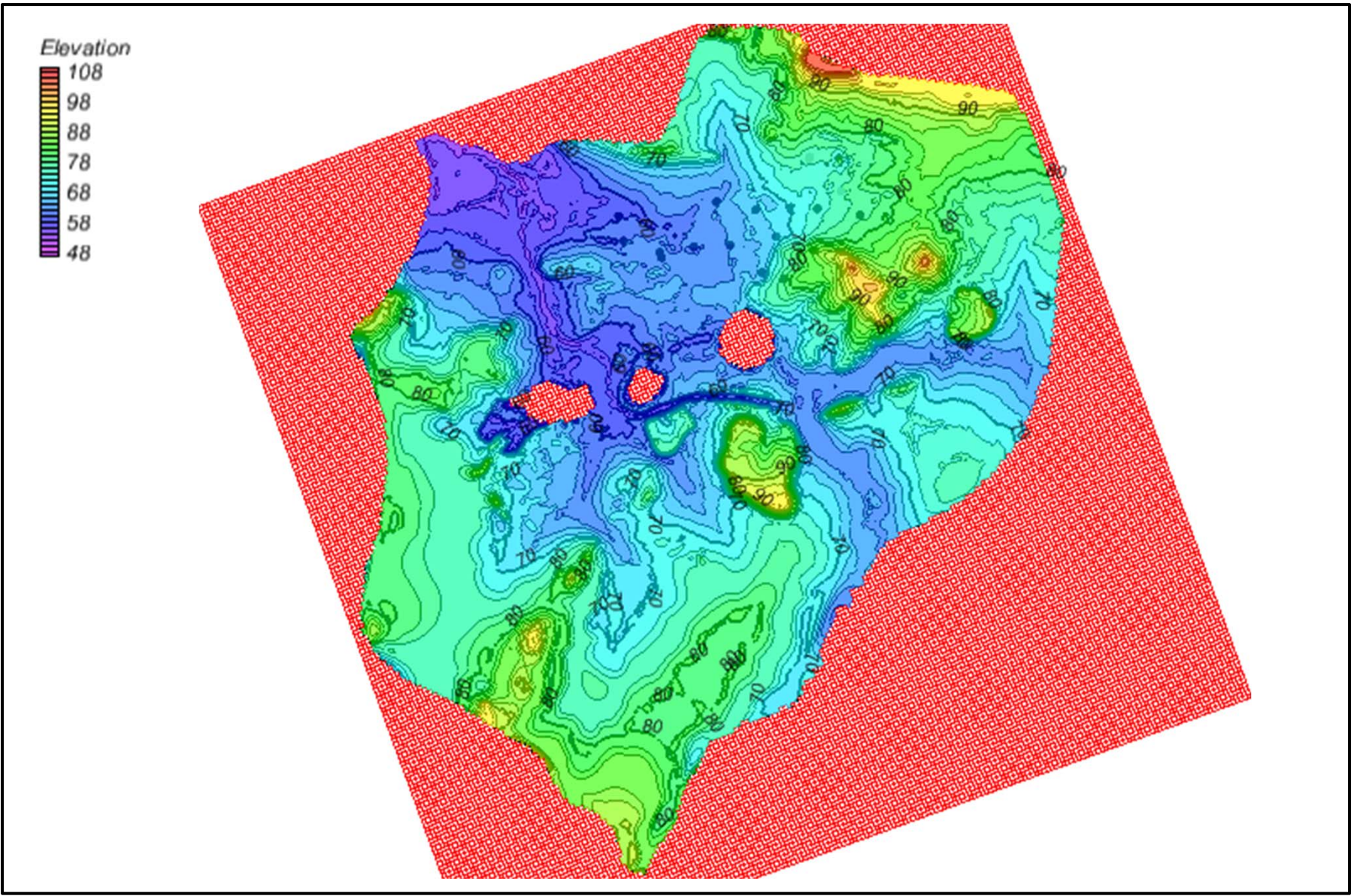
Current Model Topography (Top of Model Layer 1)
