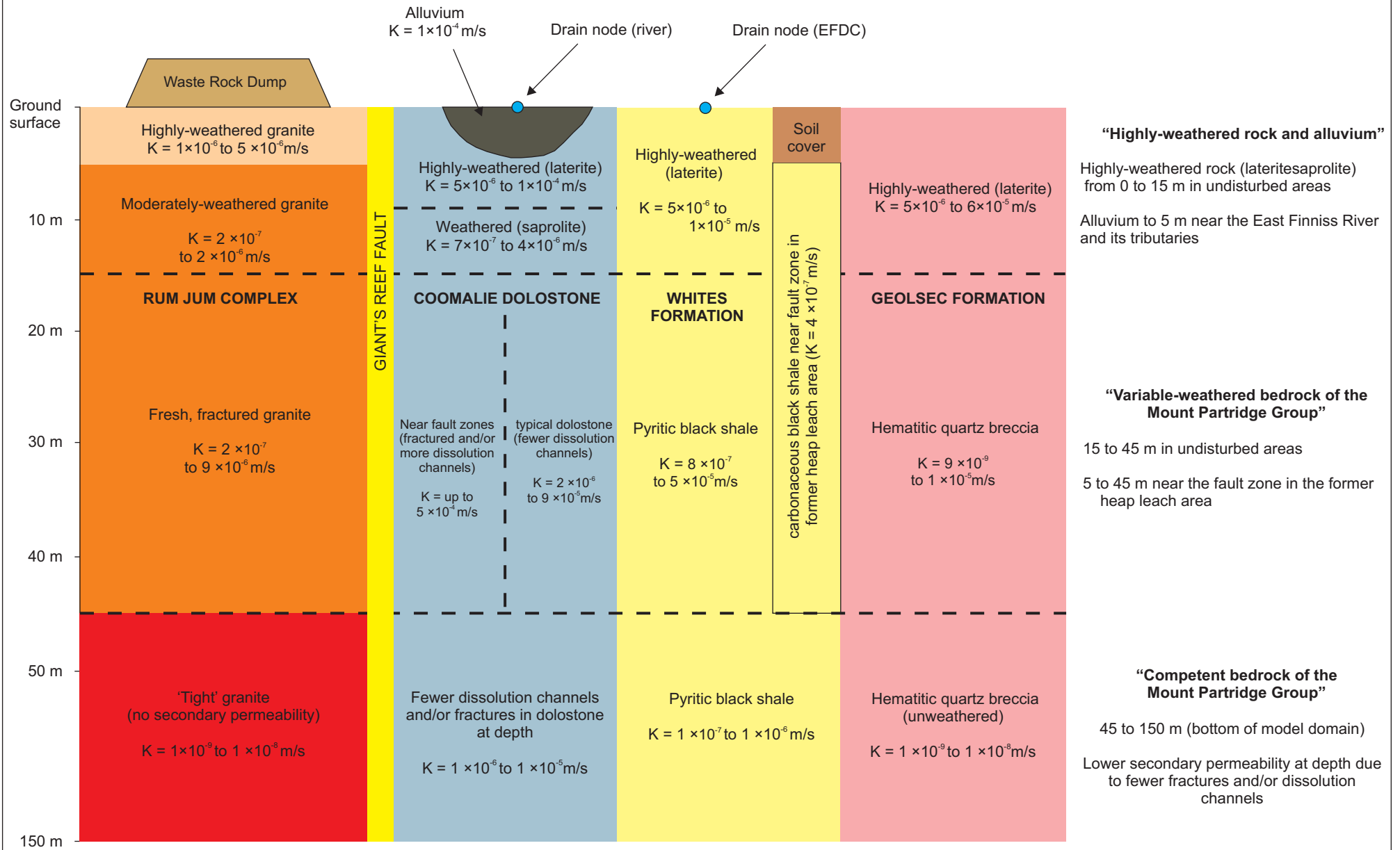
Conceptual Hydrostratigraphic Model for the Rum Jungle Mine Site
