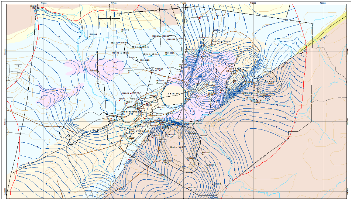
Figure E-3. Simulated Head Contours and Computed Residuals for March 2014 (Wet Season)
