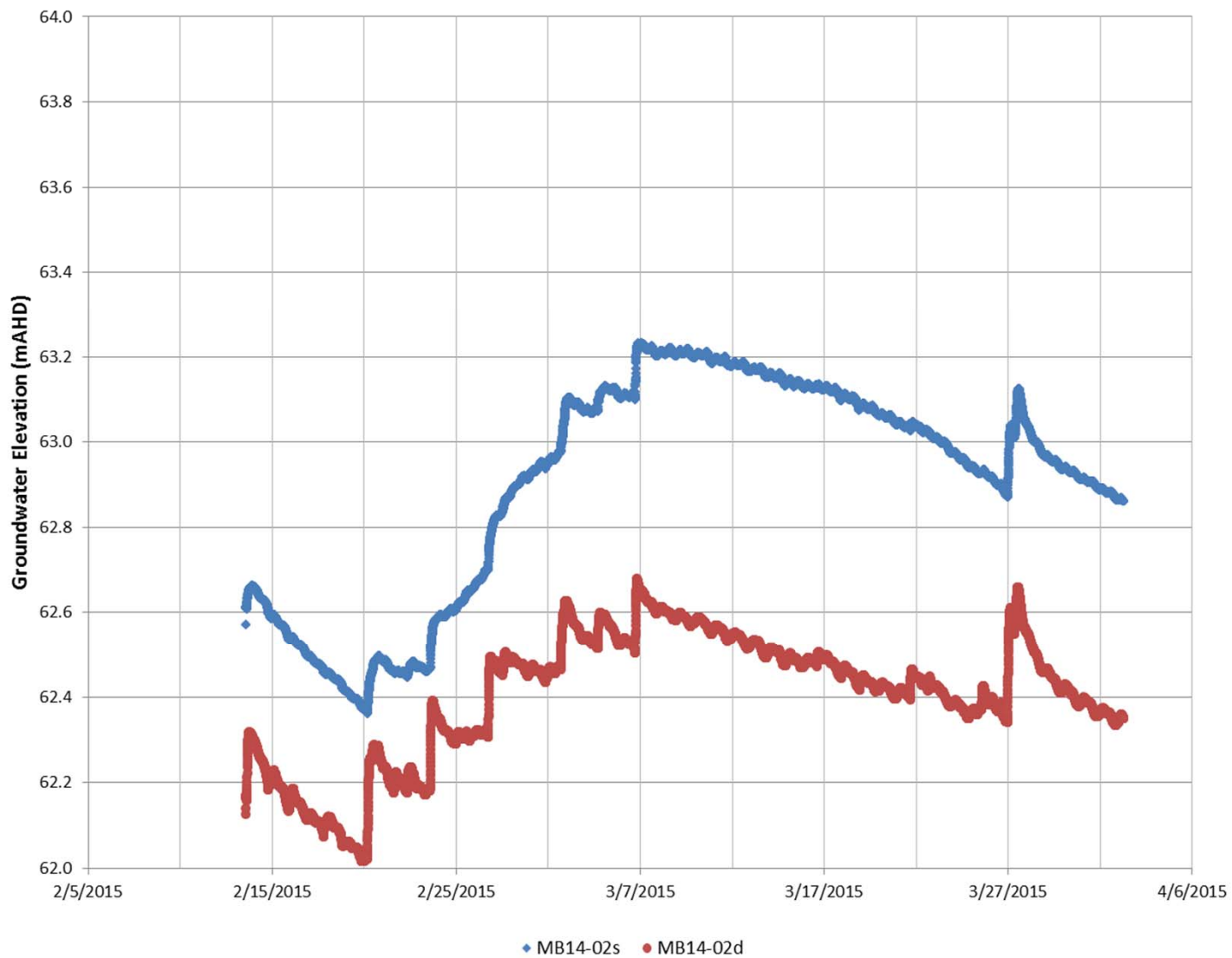
Datalogger Elevations for MB14-20S/D for February to April 2015
