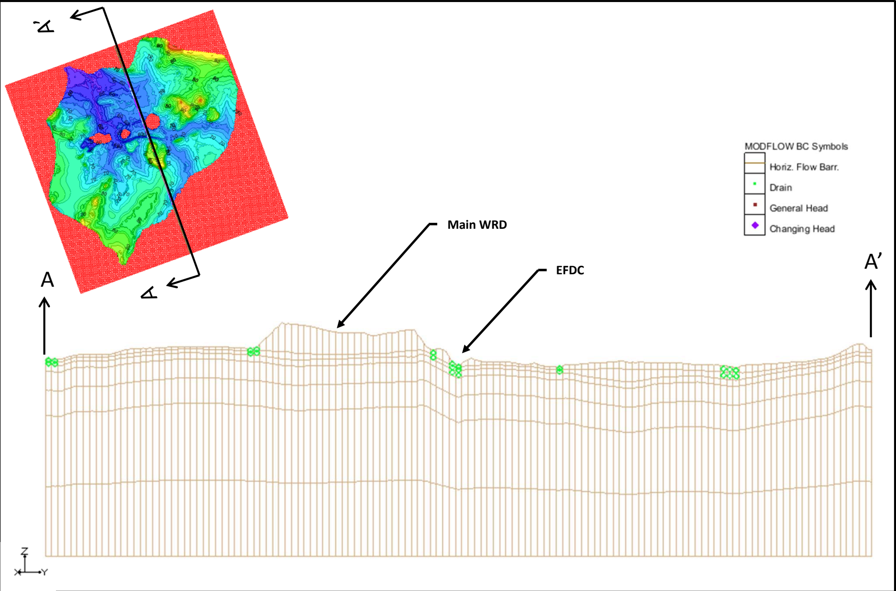
Model Cross-Section N-S Through Main WRD (Column 106)
