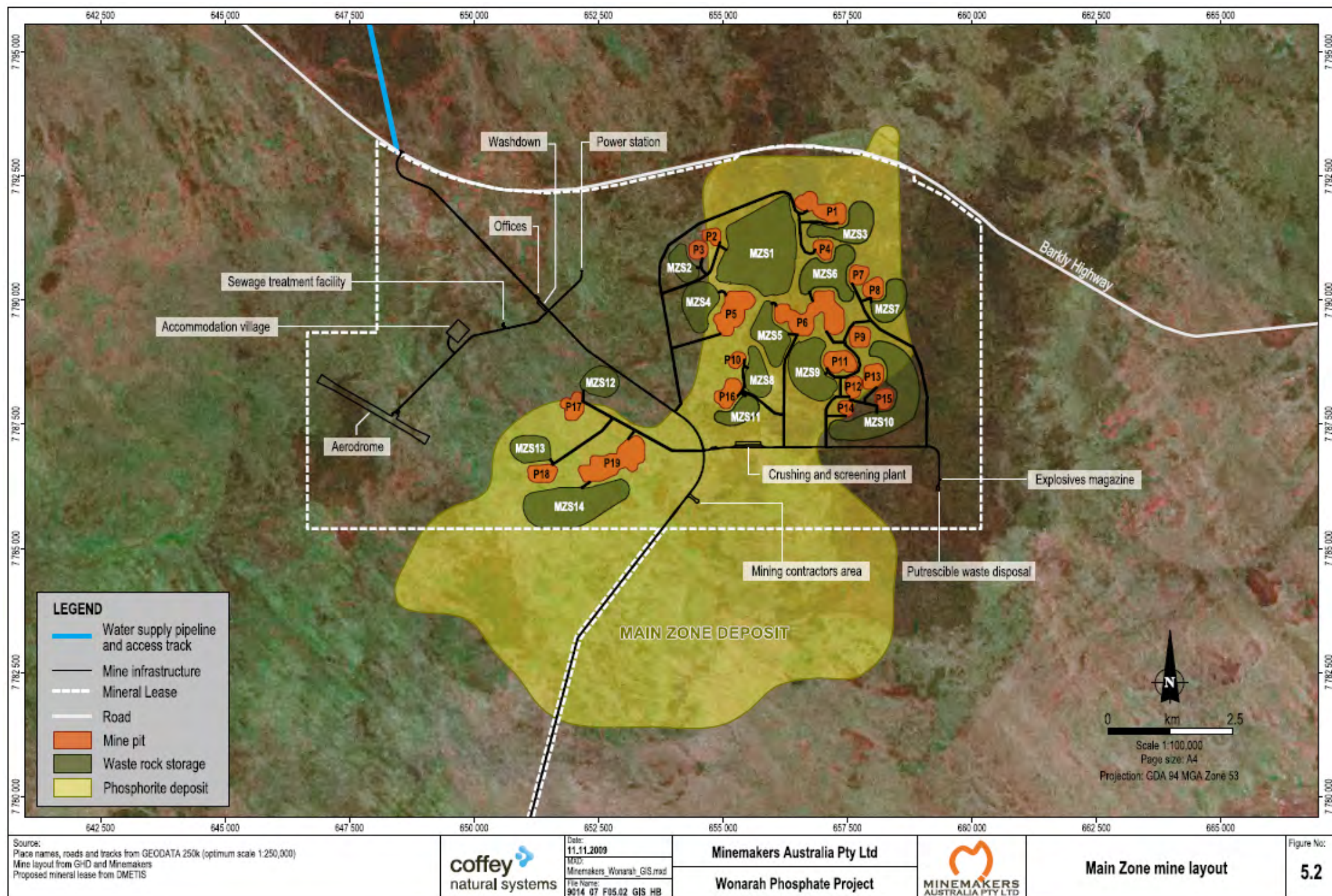
Figure 3 - Main Zone Layout
