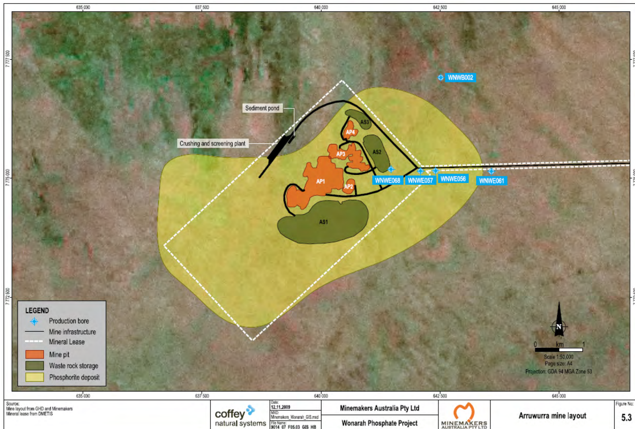
Figure 4 - Arruwarra mine layout
