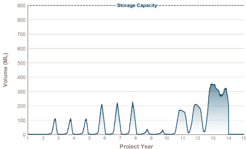
Graph 10-2 Median Quarry Water Inventory - Northern EL
