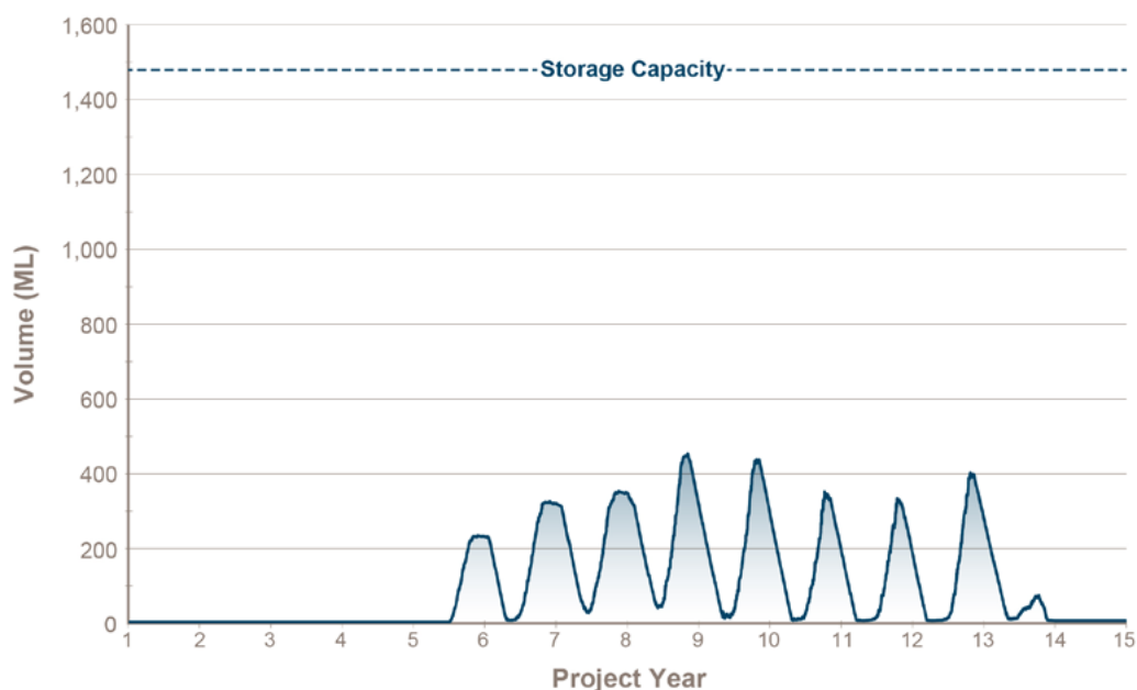
Graph 10-3 Median Quarry Water Inventory - Southern EL
