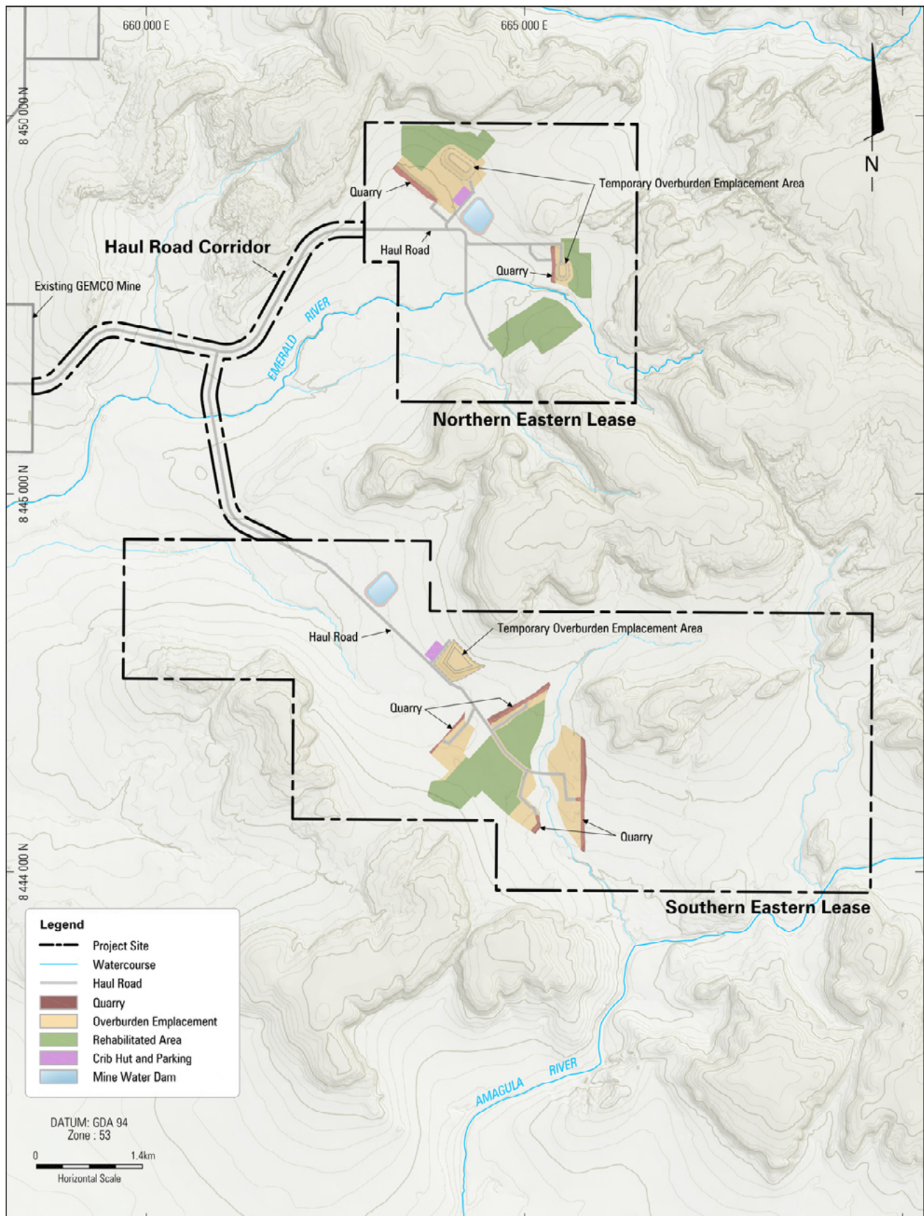
EASTERN LEASES PROJECT Indicative Mine Layout Project Year 9
