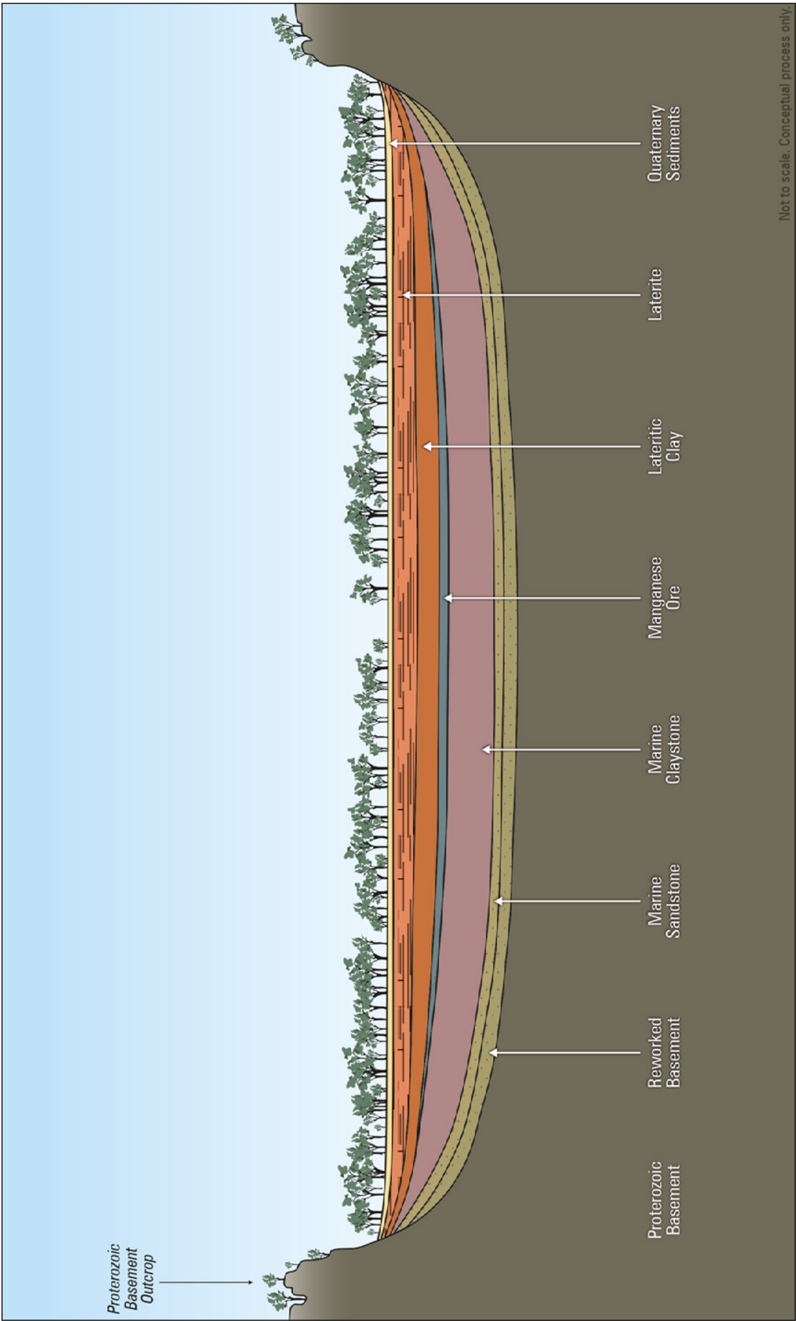
Conceptual Regional Geology Cross-Section
